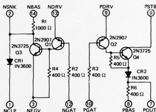
Fig. 1 Schematic of X-Y memory driver.
