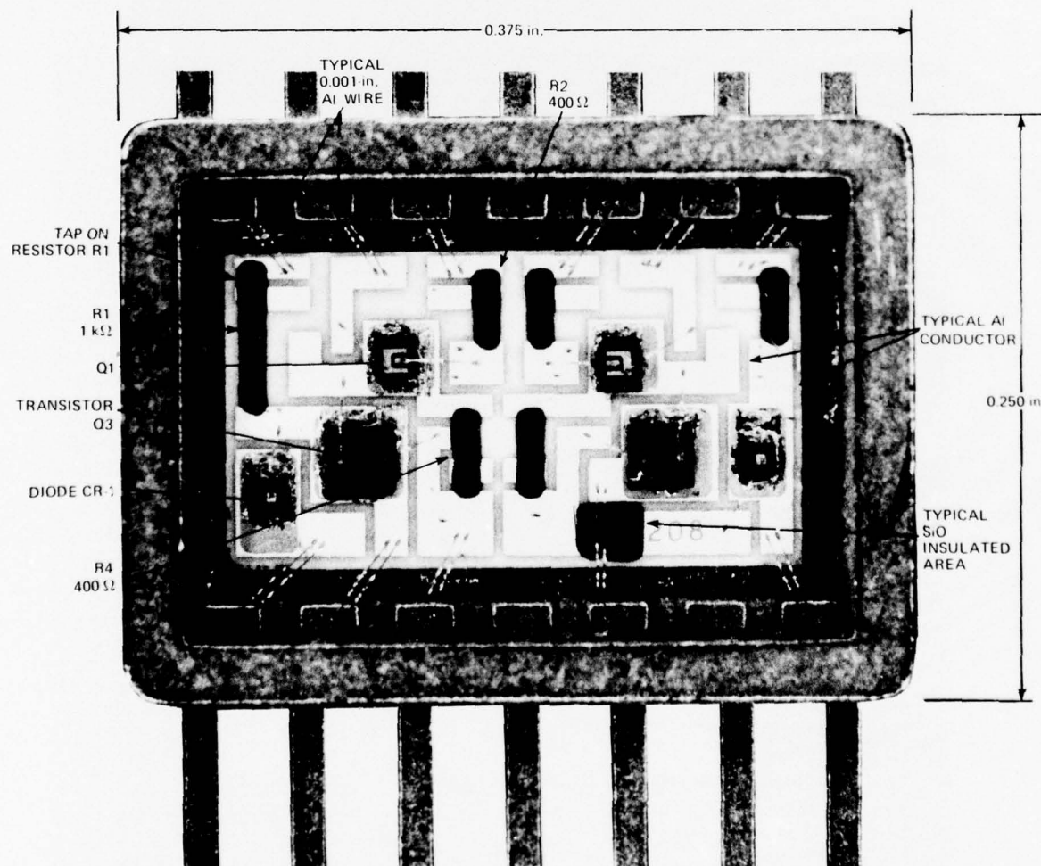
Fig. 2 X-Y memory driver hybrid microcircuit.
