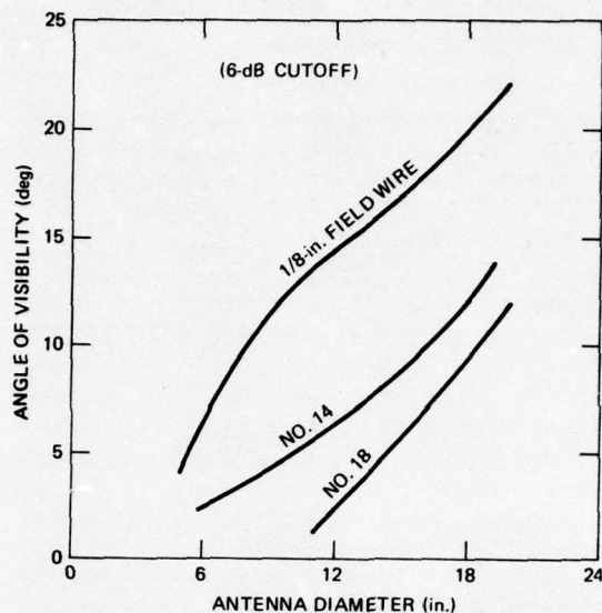
Fig. 3 Angular visibility of wire.
