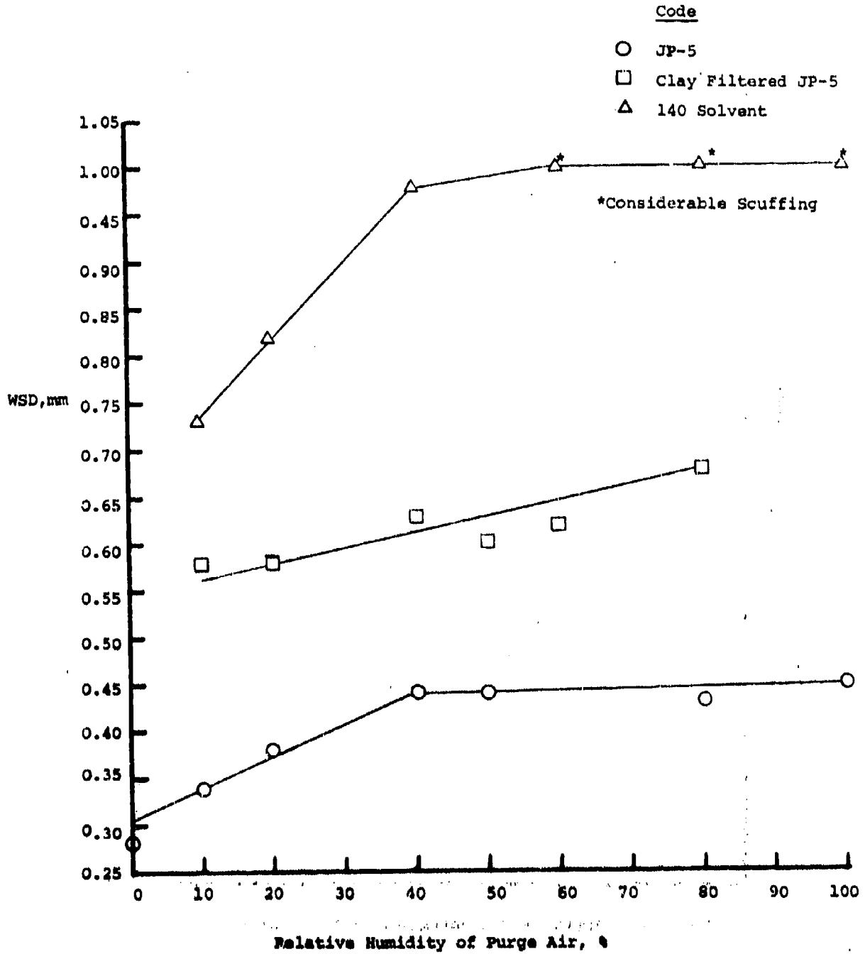
FIGURE 6: EFFECT OF HUMIDITY ON WEAR SCAR DIAMETER
