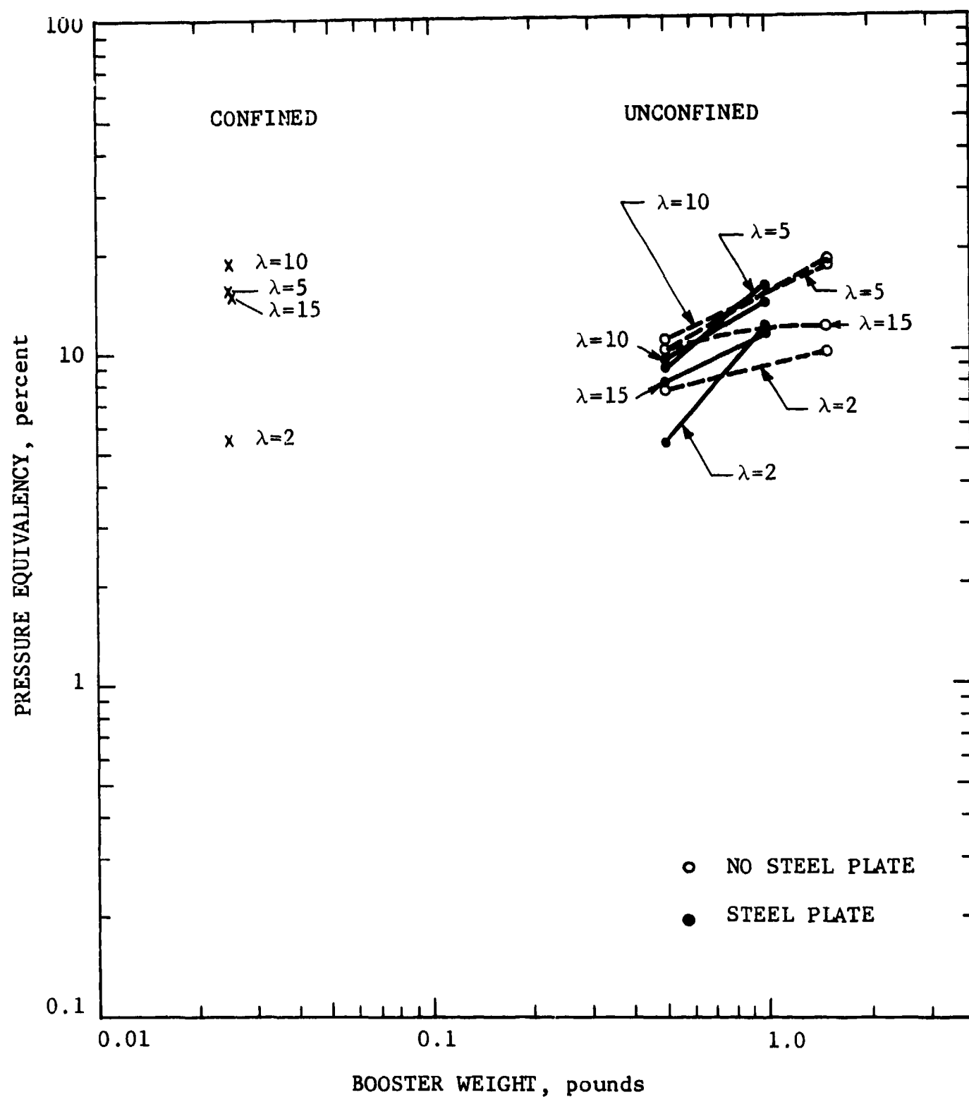
Figure 20 TNT PRESSURE EQUIVALENCY OF 75 LB BLACK POWDER AS A FUNCTION OF BOOSTER WEIGHT, FOR SELECTED SCALED DISTANCES
