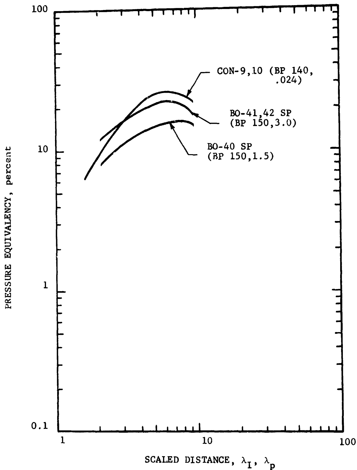
Figure 15 THE EFFECT OF BOOSTER WEIGHT AND CONFINEMENT ON TNT PRESSURE EQUIVALENCY, 140 AND 150 LB BLACK POWDER
