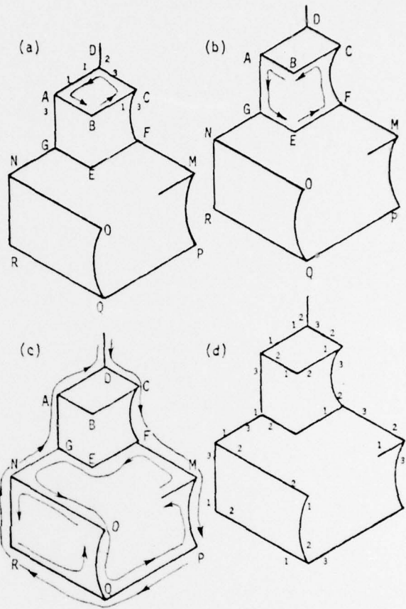
Fig. 2. Forced cyclic order.
