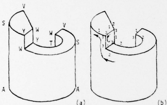
Fig. 1. Junction types and cyclic order.
