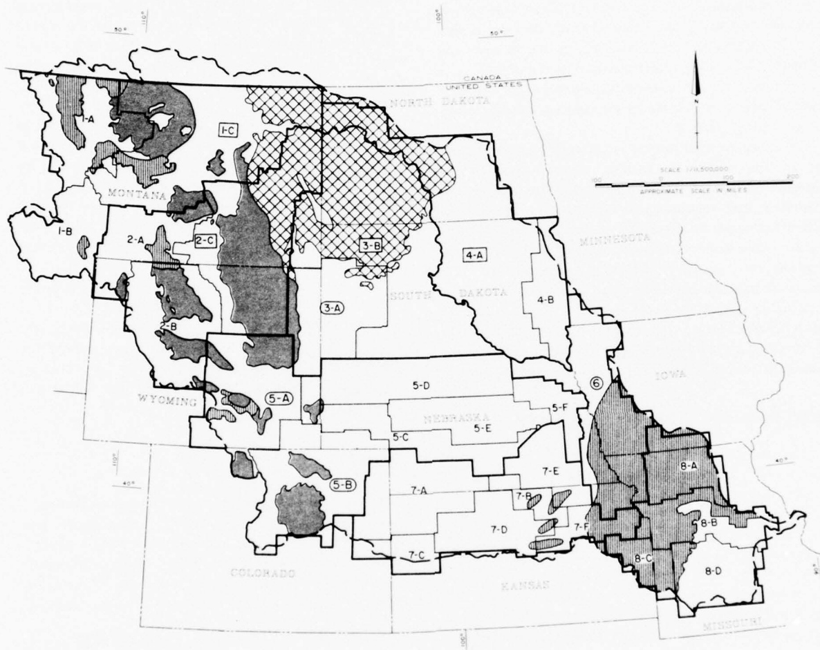
FIGURE 11 COAL FIELDS AND RESERVES, JUNE 1965
