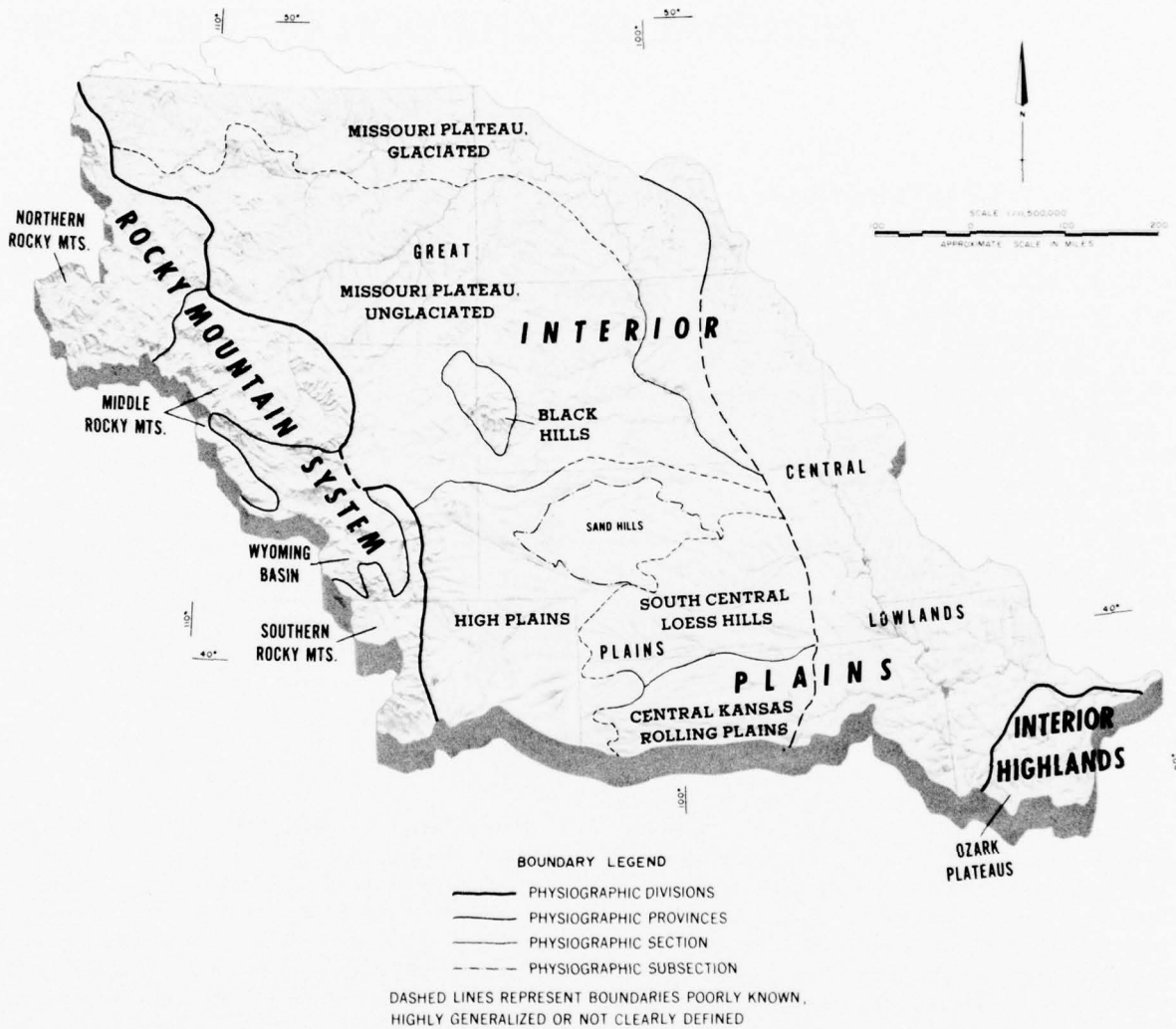
FIGURE 2 PHYSIOGRAPHIC DIVISIONS, PROVINCES, SECTIONS, AND SUBSECTIONS
