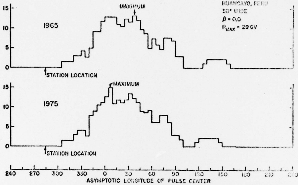
Figure 1. The response of a neutron monitor at Huancayo, Peru to a 30° wide square pulse cosmic ray anisotropy (lune of a celestial sphere) that extends to 29 GV and has a spectrum that is independent of rigidity for Epochs 1965 and 1975. The longitude of Huancayo is indicated by an arrow labeled "station location".
