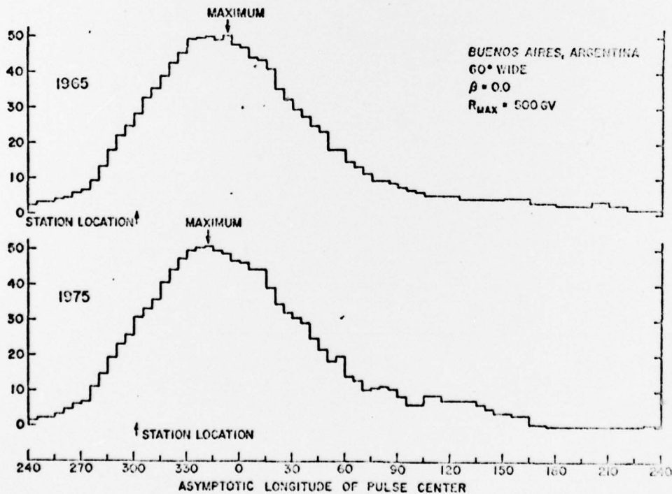
Figure 2. The response of a neutron monitor at Buenos Aires, Argentina to a 60° wide square pulse cosmic ray anisotropy (lune of a celestial sphere) that extends to 500 GV and has a spectrum that is independent of rigidity for Epochs 1965 and 1975. The longitude of Buenos Aires is indicated by an arrow labeled "station location".
