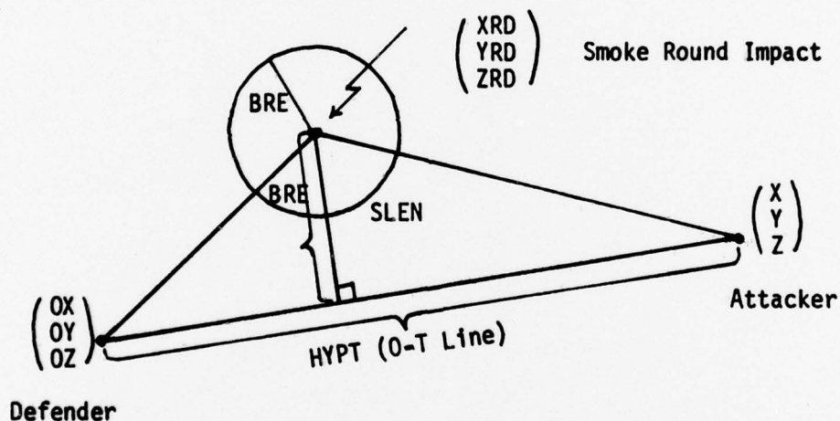
Figure C-1. Sphere/Line Intersection
