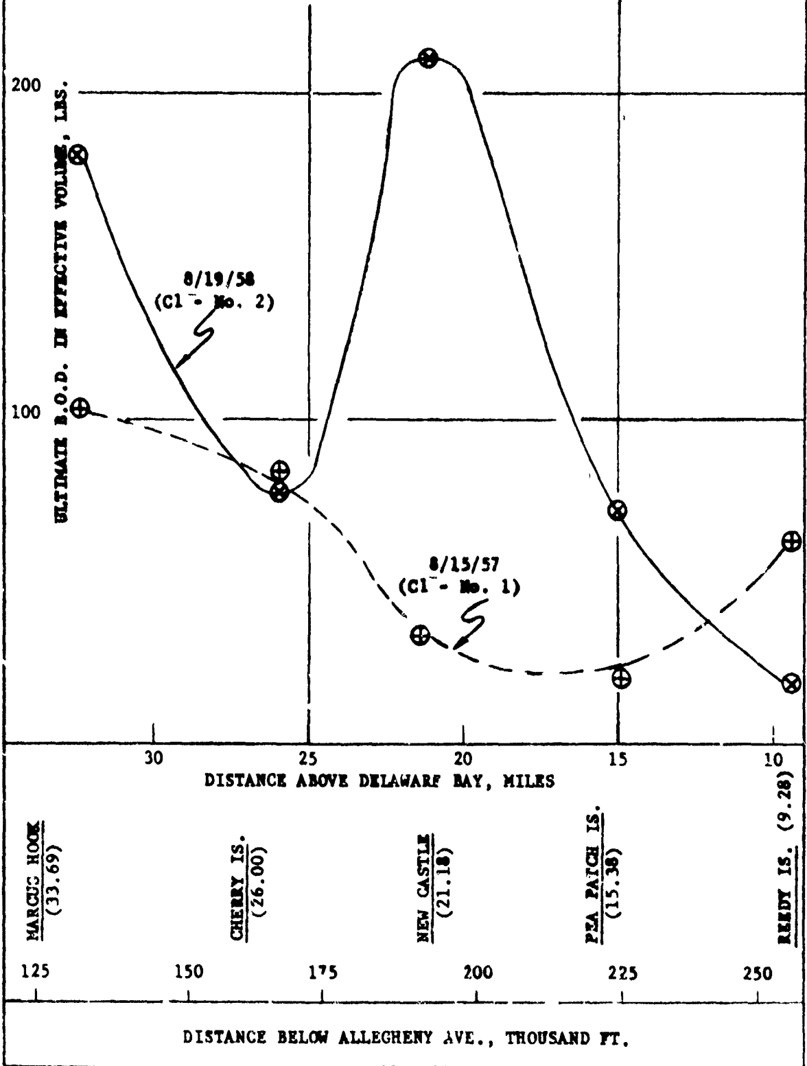
EFFECT OF FRESH WATER FLOW ON ULTIMATE BOD CONTENT MEASURED DURING LOW WATER SLACK FIG. 25 1957-1958
