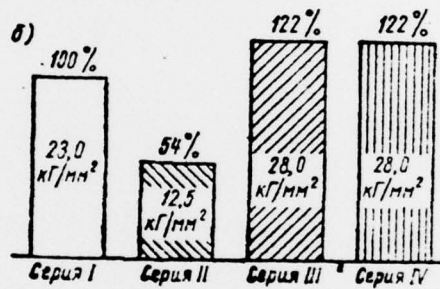
Fig. 4. Specimen cyclic load test results: a - fatigue curves in semi-logarithmic coordinates; b - the correlation of the fatigue strengths of the various series: o, I - parent metal; \blacktriangle , II - specimens with a weld without thermal treatment; \triangle , III - parent metal after thermal treatment; \bullet , IV - specimens with a weld after thermal treatment
