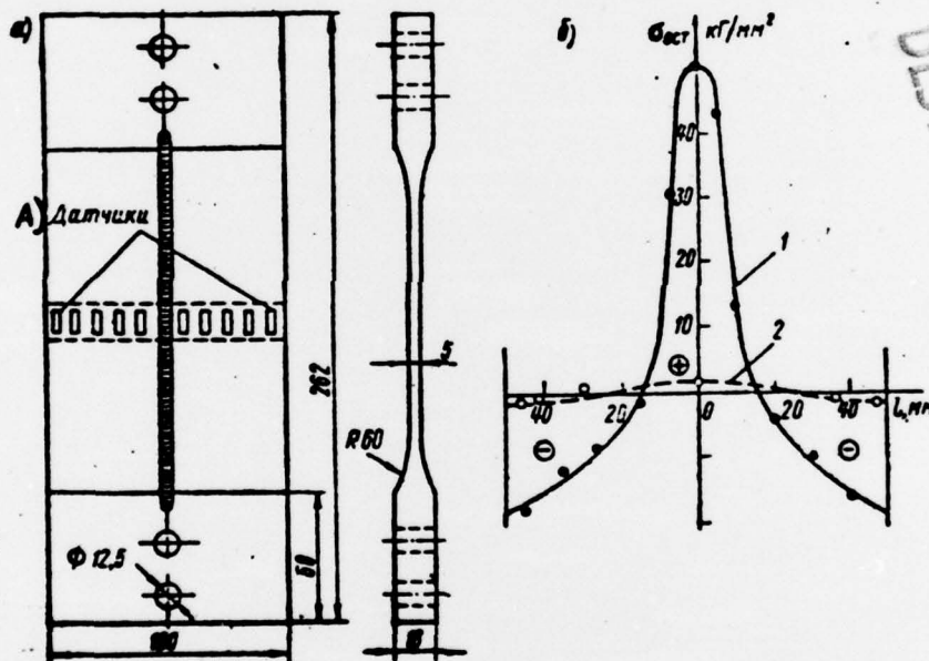
Fig. 1. The specimen used in tests (a), and the residual stress curves (b): 1 - after penetration; 2 - after thermal treatment.
