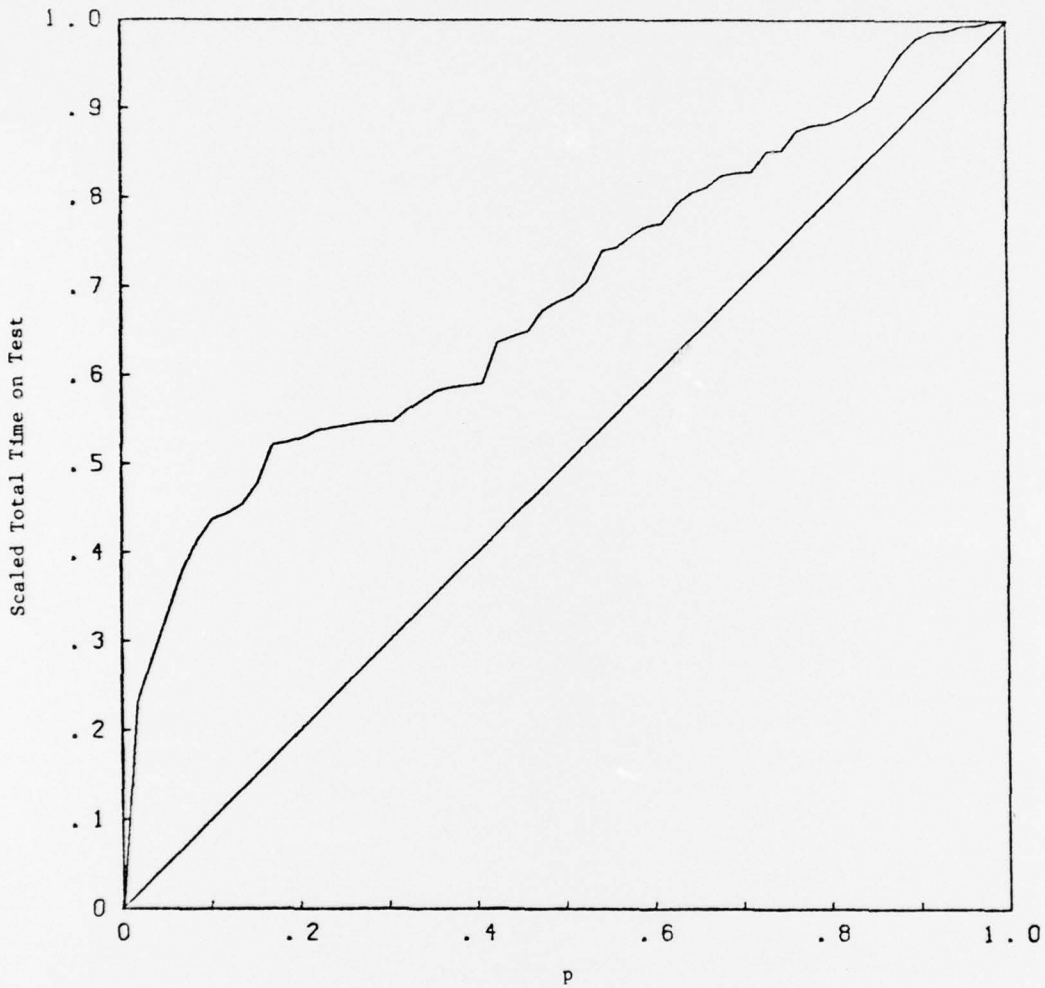
TOTAL TIME ON TEST PLOT FOR NON-HOMOGENEOUS POISSON MODEL - ENGINE FAILURE DATA
