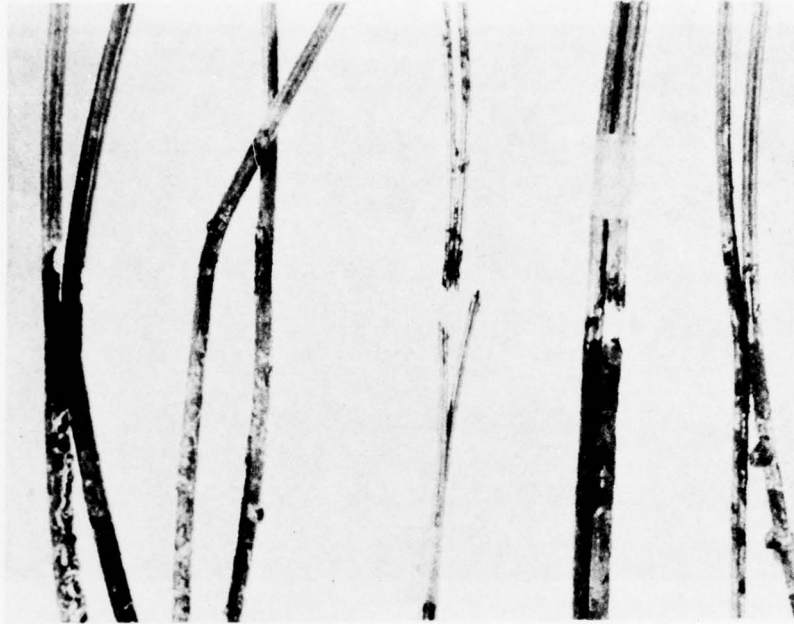
Figure 6. Spot-welded stainless steel wire specimens exposed 15 months in brackish water. From left: AM 363, AISI 201, Armco 18-2, AISI 430, and AISI 301. (Block W-2)
