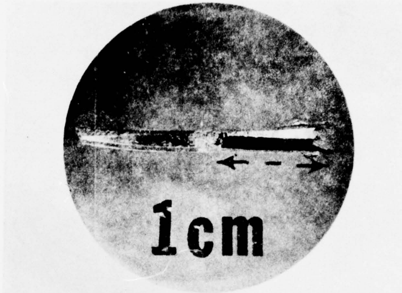
Figure 15. Exposed end of copper-clad steel wire after exposure. Note the porous steel core and the attack on the inside of the copper cladding. (55x)
