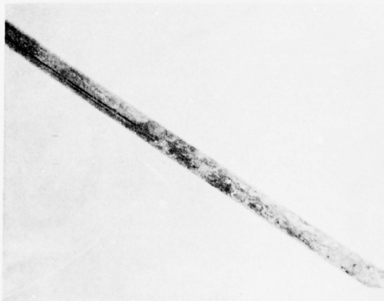
Figure 9. Corrosion and pitting in AM 363 stainless steel wire after 15 months of exposure in brackish water. (Block 48)
