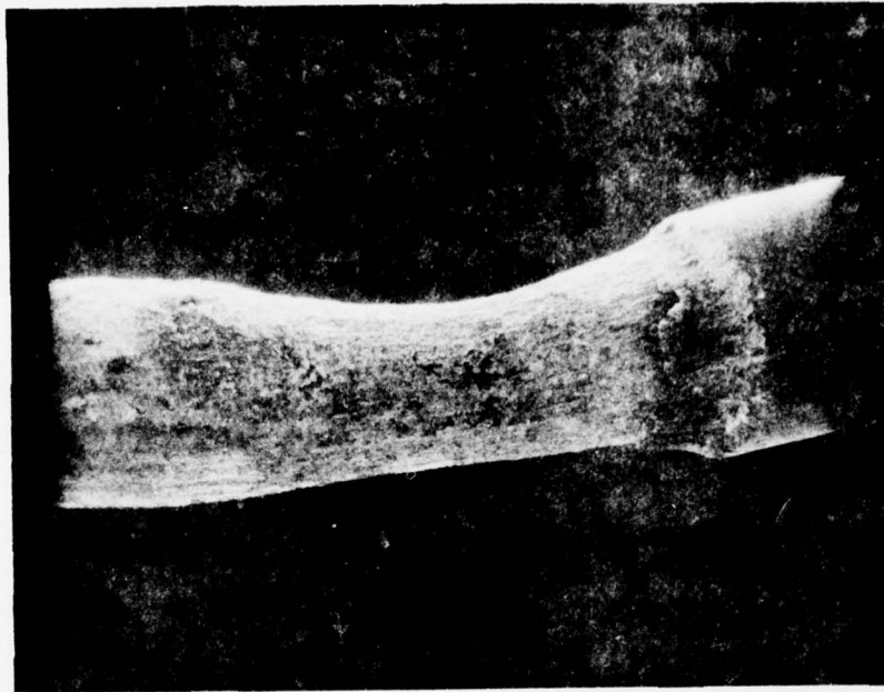
Figure 11. SEM photograph of the accelerated corrosion region in plain carbon steel wire. Note the geometry of attack, the layered corrosion region, and the apparent attack at the grain boundaries.
