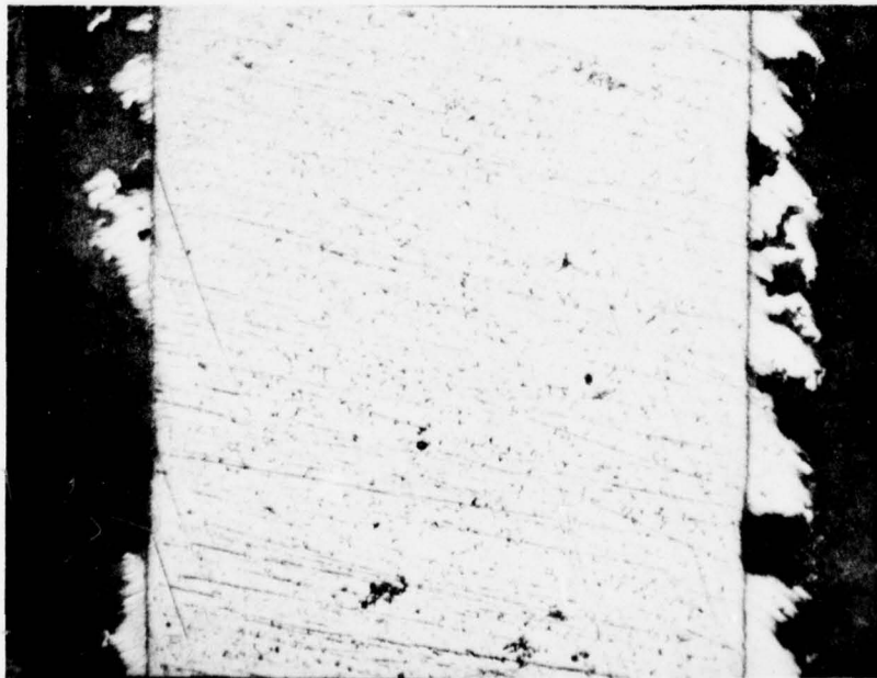
Figure 12. Micrograph of galvanized wire after exposure for 1 year. Note the presence of deep pits in the zinc outer layer which penetrate to the surface of the steel. (50x)
