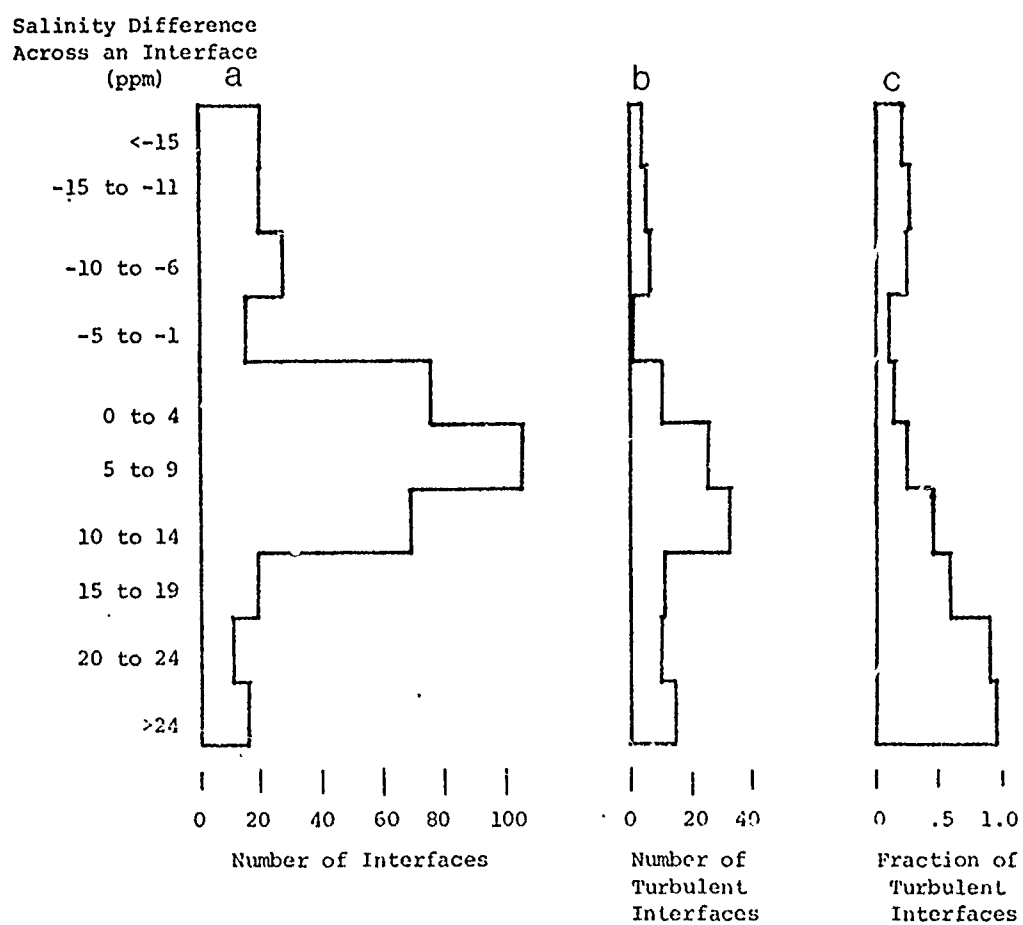
FIGURE 3.13 Distributions of interfaces and turbulent interfaces as a function of salinity difference. When salinity decreases with increasing depth, the salinity difference is positive. The fraction of turbulent interfaces is shown on the right, and it is monotonically increasing with increasing positive salinity difference.
