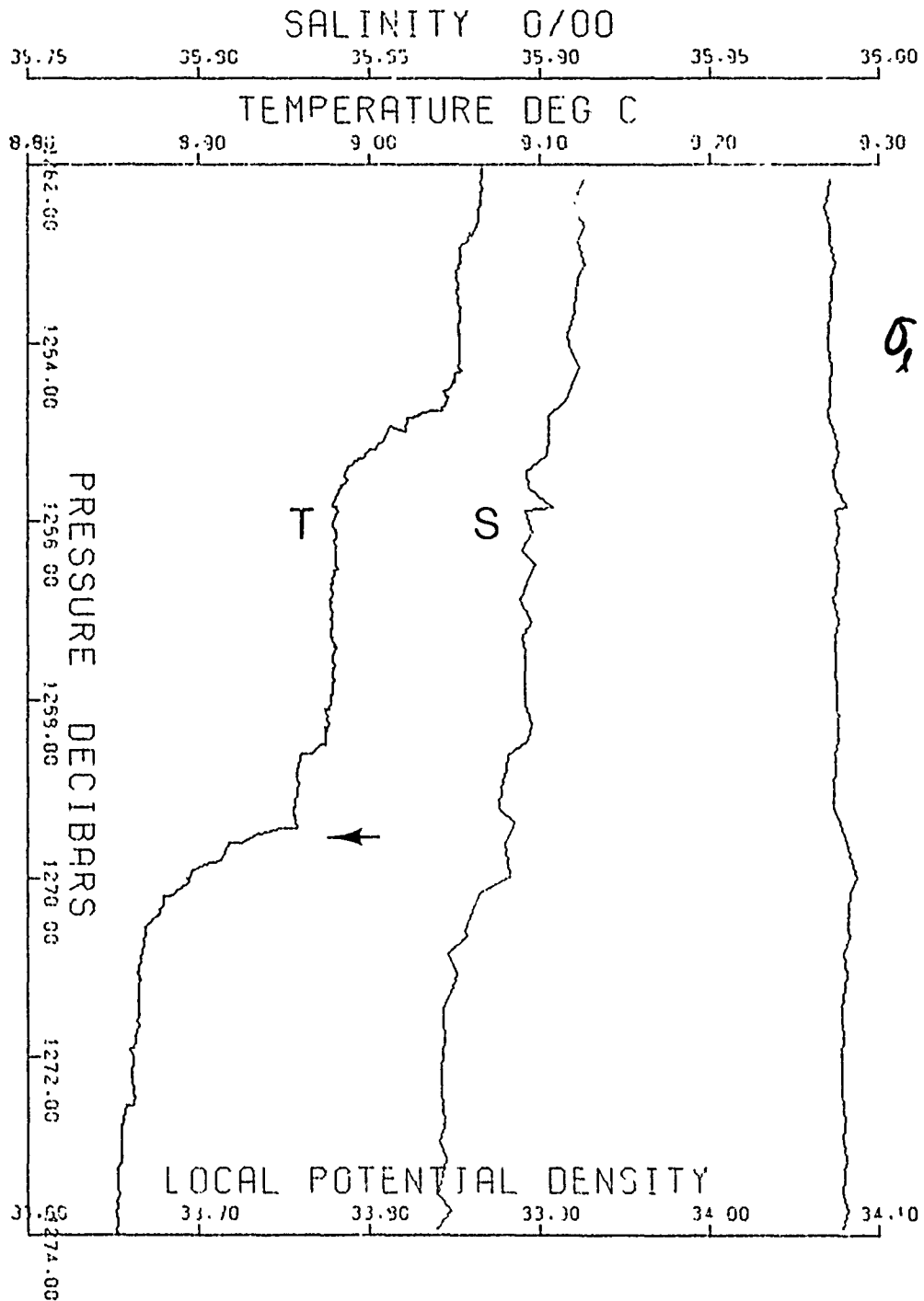
FIGURE 3.27 Profiles of temperature, salinity, and local potential density just below a secondary salinity maximum from SCIMP 2. The arrow marks the position of high contrast images in the shadowgraphs.
