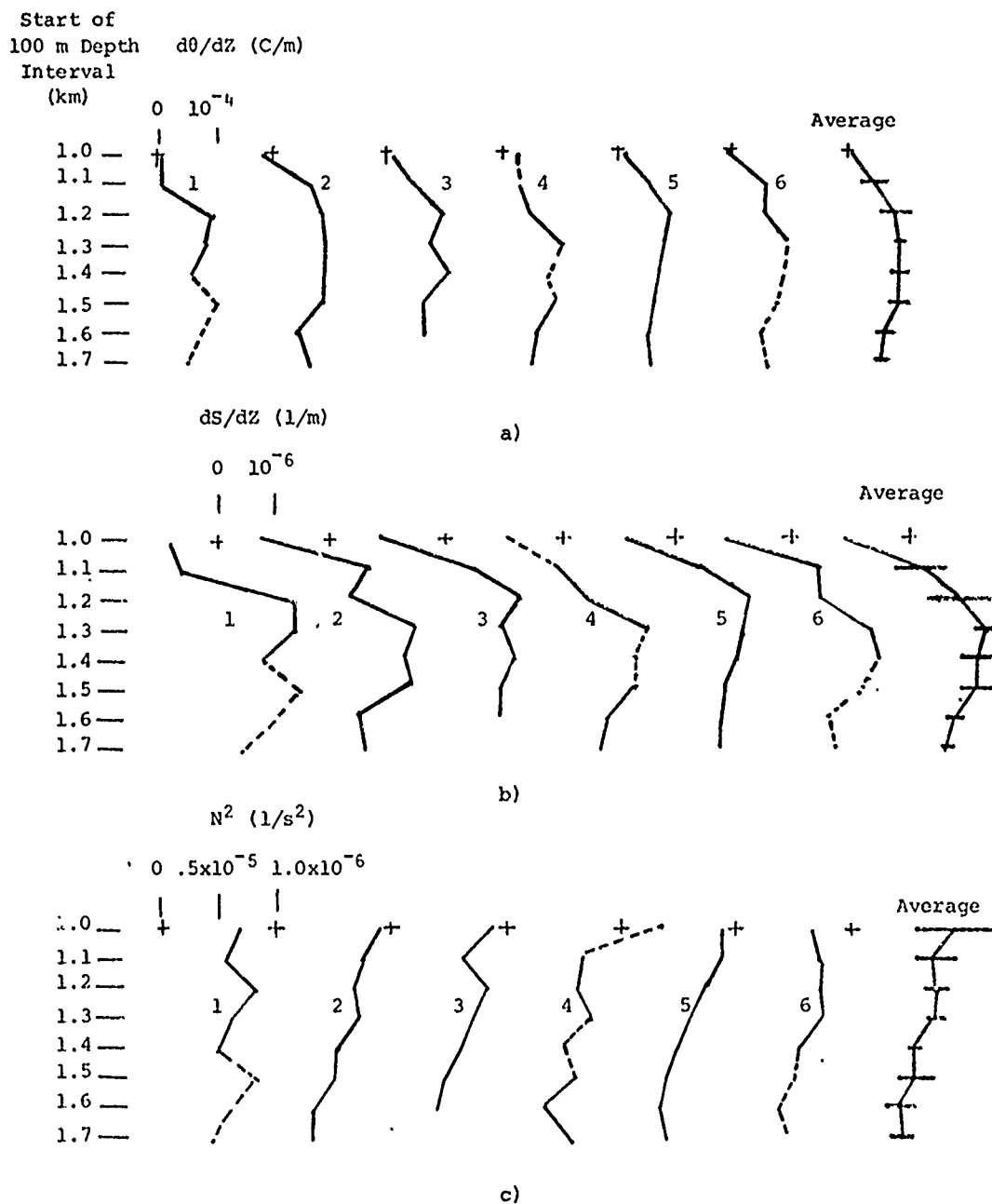
FIGURE 3.15 Mean gradient profiles of a) potential temperature, b) salinity, and c) density expressed as the square of the Brunt-Väisälä frequency. Each of the 6 SCIMP dives is plotted as well as the average of the 6. The standard deviation is shown as a horizontal bar at each level on the average. Each profile is offset horizontally by a constant distance as indicated by the positions of the crosses. The profiles are dashed where the pressure sensor was performing erratically.
