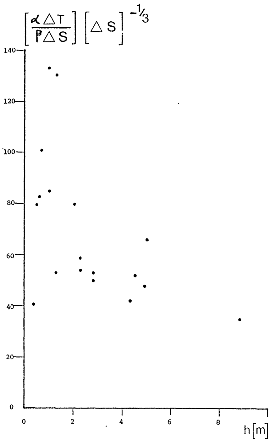
FIGURE 3.3 Comparison of calculated interface thickness to measured distance between mixed layers. The ordinate is proportional to the length of salt fingers calculated from the conditions at the interface. Each point represents an interface where there is high contrast banded structure in the shadowgraphs. The measured distance is not well represented by the calculation.
