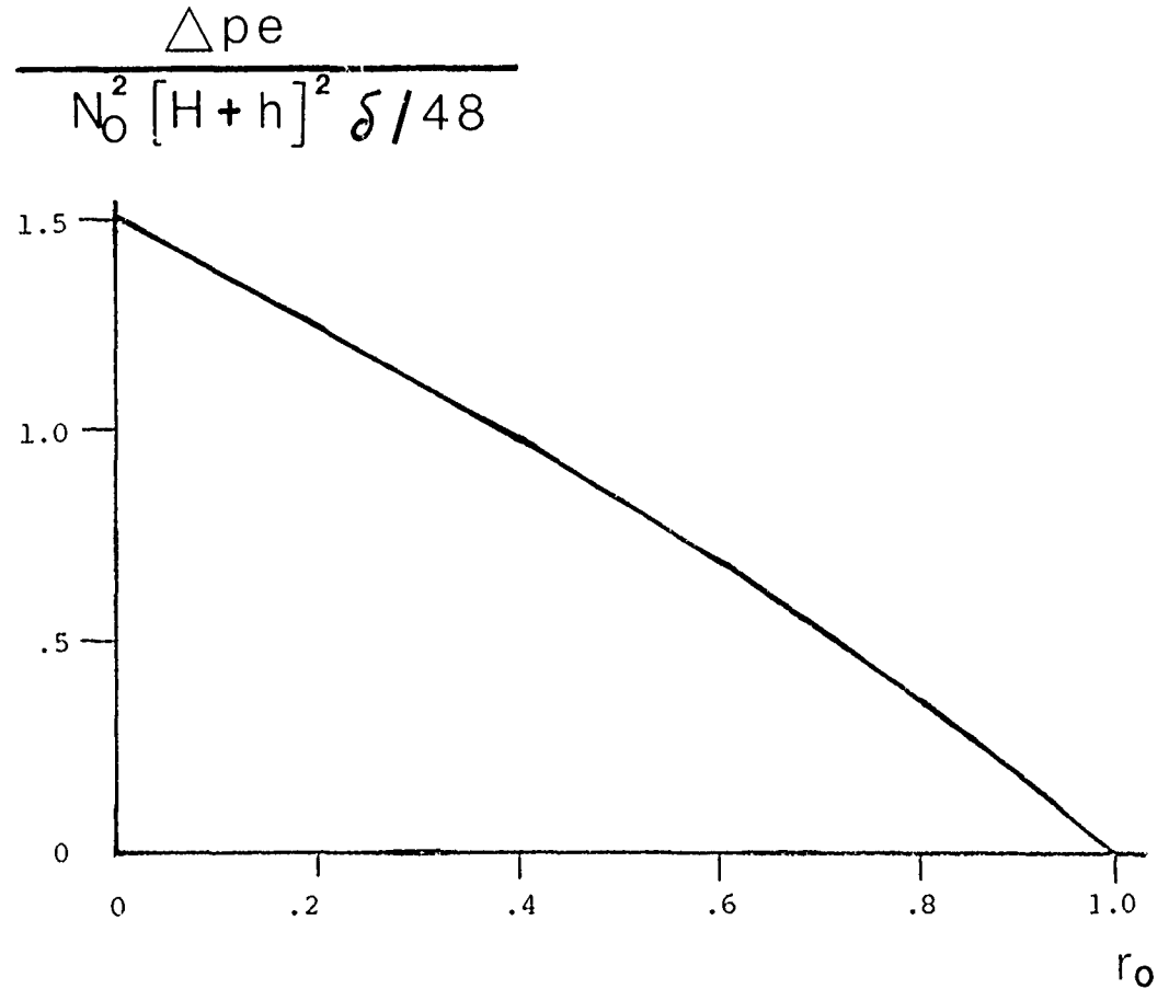
FIGURE 2.7 Dimensionless potential energy change for thickening an existing homogeneous layer in a homogeneous layer and constant density gradient system. The abscissa is the ratio of the interface thickness to the sum of the layer and the interface thicknesses. As the interface becomes relatively thin, an increasingly large amount of energy is required to thin it further. The rate of increase is very nearly linear.
