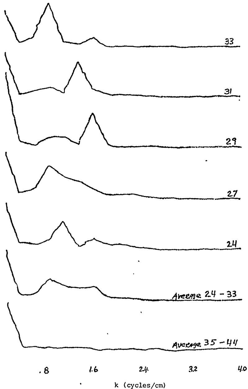
FIGURE B-3 Spectra of photointensity for a horizontal scan across the photographs in Figure B-2. A number identifies each spectrum with a photograph. There is a strong peak in the spectrum near 1 cycle/cm for each of the photographs. Each estimate has 10 degrees of freedom. The average of the 5 spectra is also shown as well as the average of the 5 spectra from the photographs of the lower part of the interface. The units of the ordinate are arbitrary but uniform.
