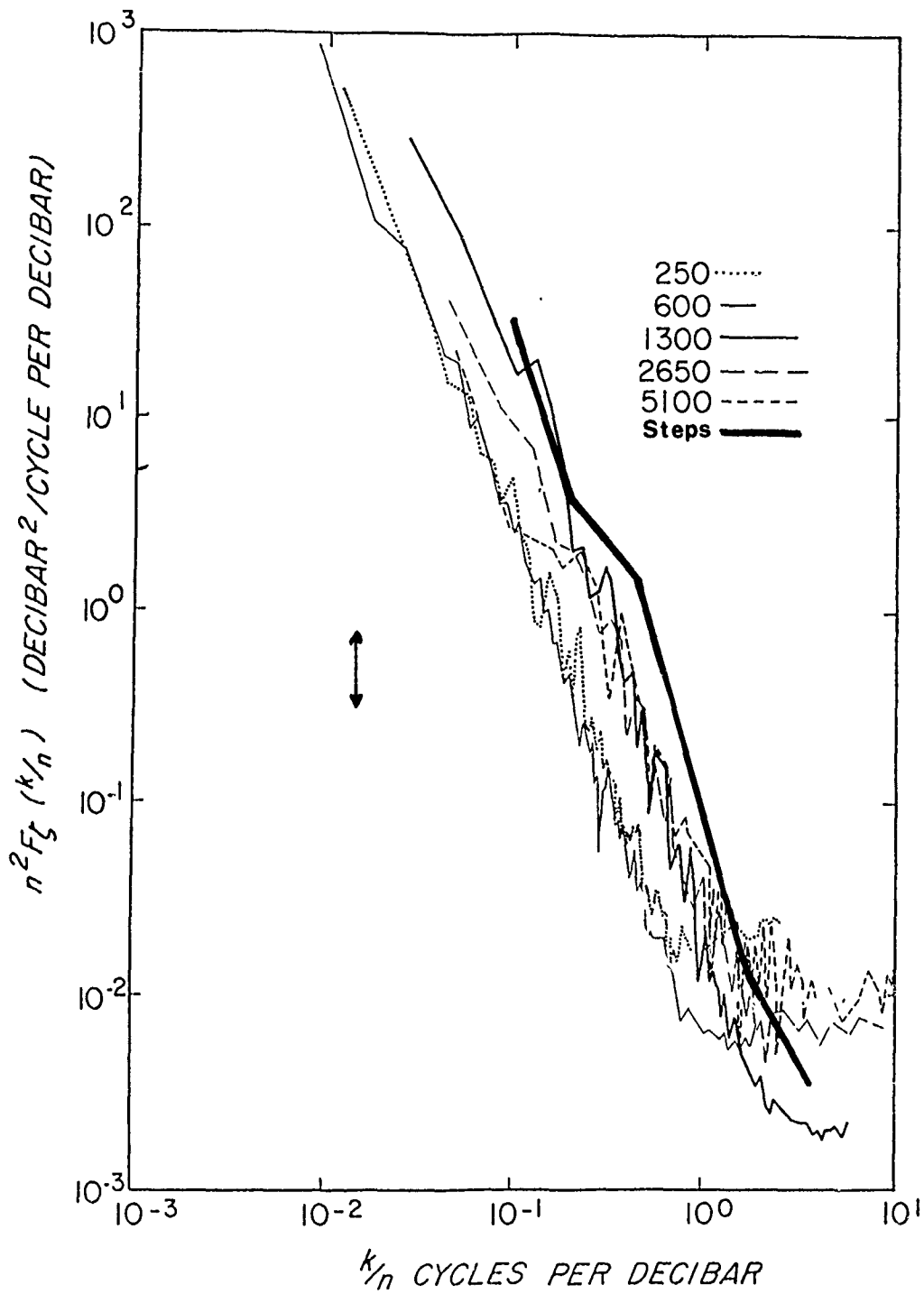
FIGURE 3.20 Normalized displacement spectra assuming Garrett and Munk 1975 model spectrum. The normalized spectra are essentially the same as the unnormalized displacement spectra in 3.19. The bar indicates 90% confidence limits.
