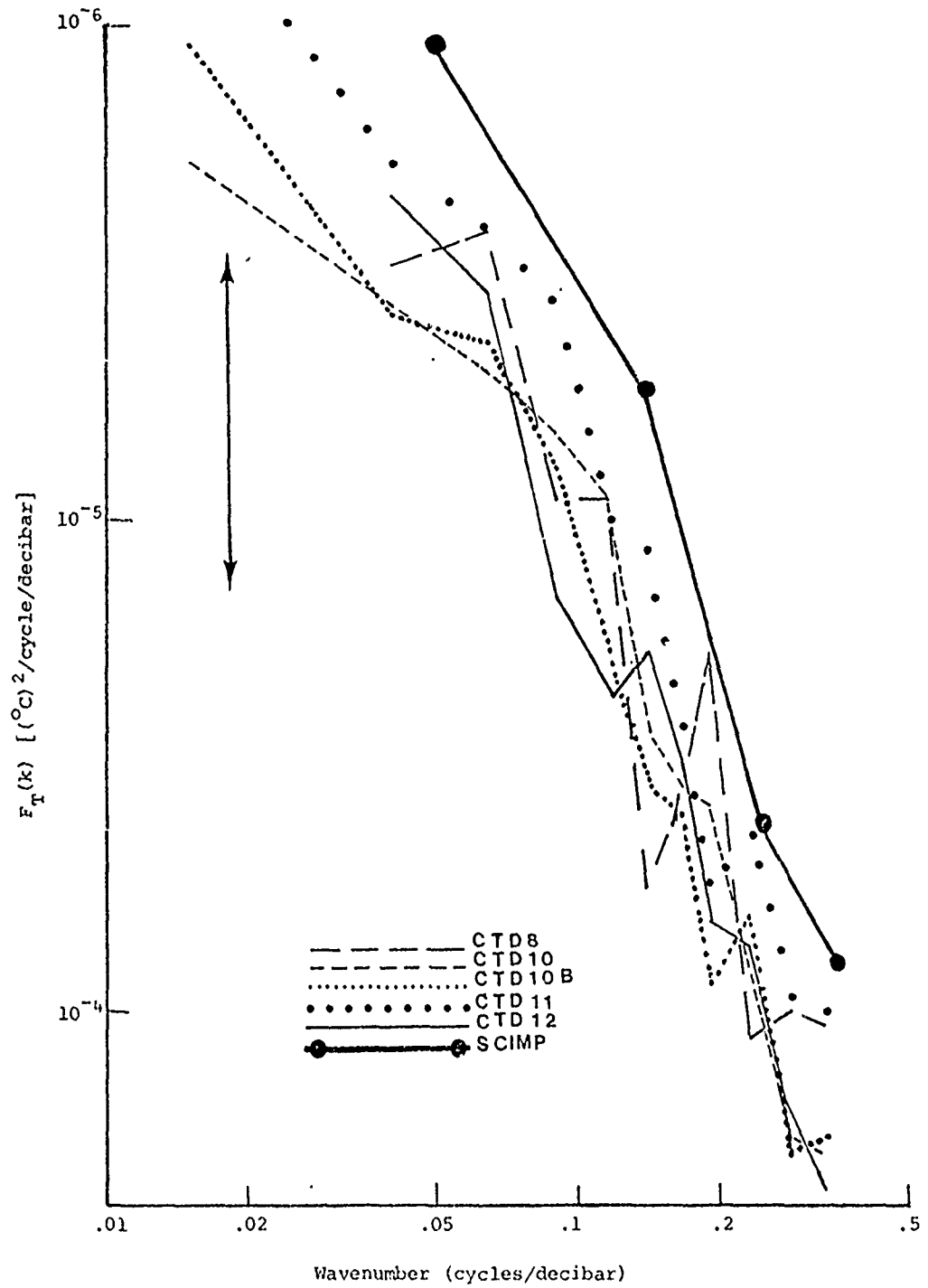
FIGURE 3.18 Comparison of individual CTD autospectra of vertical temperature with SCIMP in low wavenumber band. The spectrum from SCIMP is above the CTD's throughout the band. The bar indicates 90% confidence limits for the CTD.
