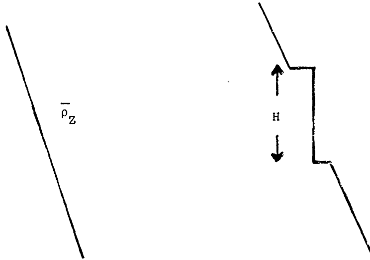
FIGURE 2.5 Formation of a homogeneous layer from a constant density gradient.
