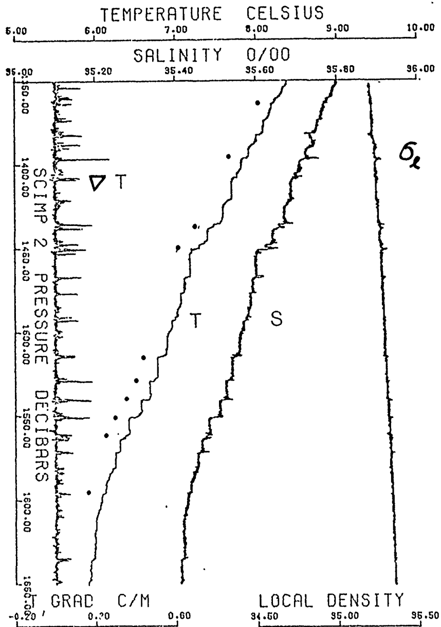
FIGURE 3.2 Expanded profiles of temperature, salinity, local potential density and temperature gradient for SCIMP 2 (Fig. 3.1). The stepped structure is included and the dots beside the temperature profile mark interfaces with high contrast banded structure in the shadowgraphs.
