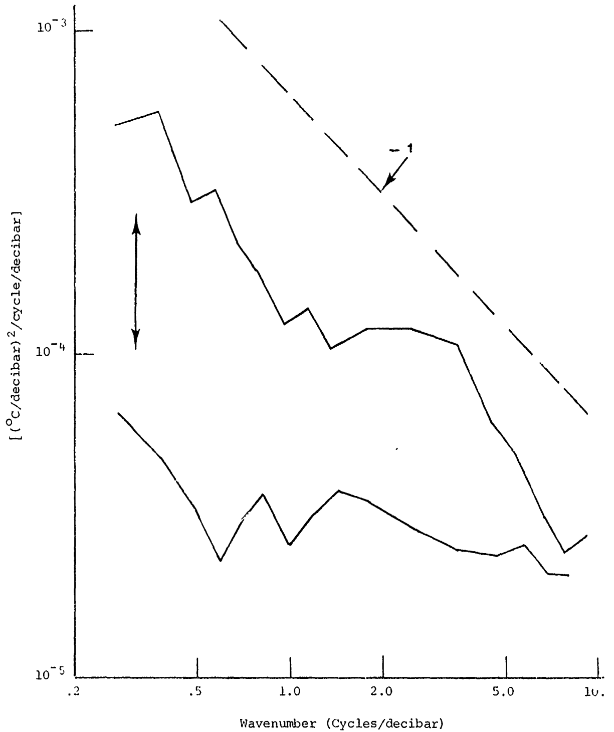
FIGURE 3.21 Temperature gradient spectra from SCIMP. The upper solid line is from the steps measured on SCIMP 2; the lower is from a featureless portion of SCIMP 5. The dashed line has a slope of -1. The 90% confidence limits are indicated with a bar.
