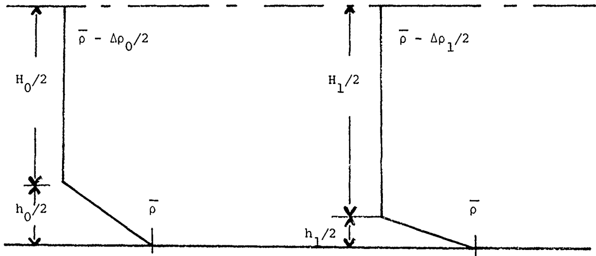
FIGURE 2.6 Thickening of a homogeneous layer. Half an interface and half a layer are shown. The density at the center of the interface is constant, as is the sum of the layer and interface thicknesses.
