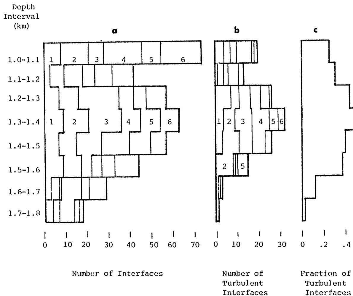
FIGURE 3.11 Distributions of interfaces and turbulent interfaces for the 6 SCIMP dives as a function of depth. The depth interval between 1.0 and 1.8 km is divided into 100 m increments for the census. The numbers within the diagrams show how the interfaces are distributed among the dives. The diagram on the right shows what fraction of interfaces are turbulent as a function of depth.
