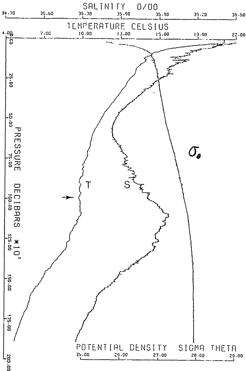
FIGURE 3.1 Profiles of temperature, salinity and potential density from SCIMP 2. The measurements were made from the P/V ATLANTIS II, 0017Z, 18 July 1973 at 34-16.1°N, 10-49.8°W. The arrow indicates where the OSFD was turned on.
