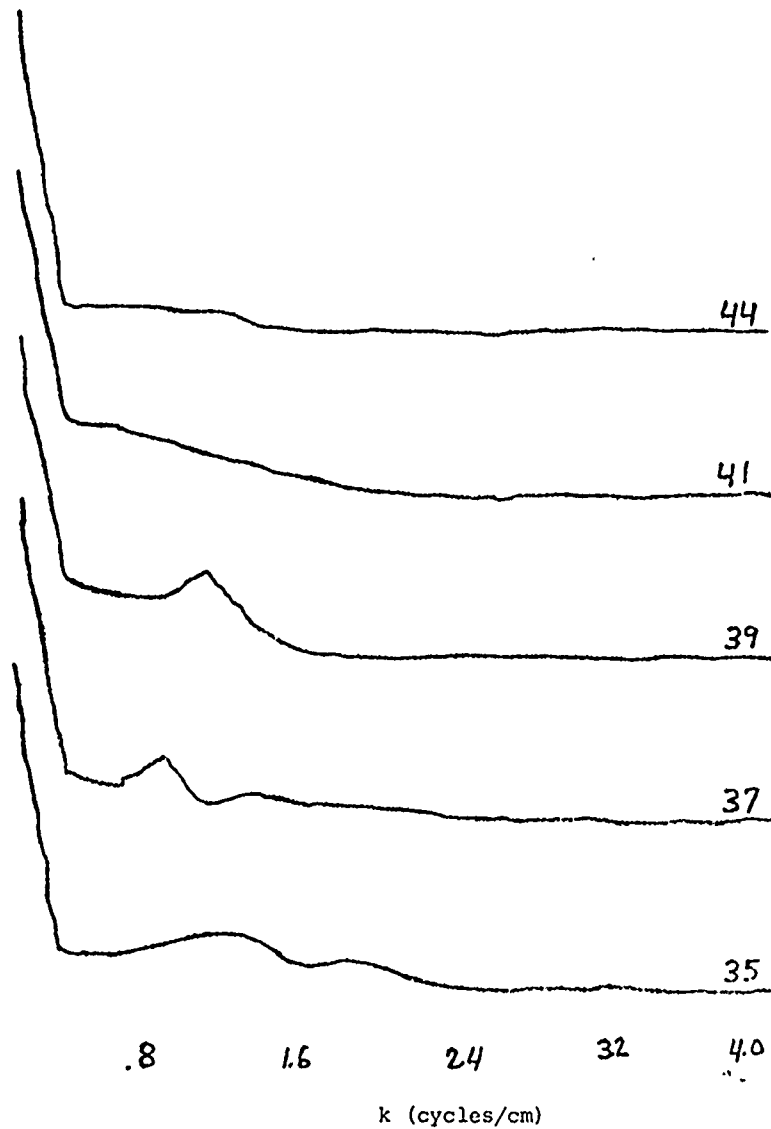
FIGURE B-4 Spectra of photointensity for 5 photographs from the lower part of the interface in Figure B-1. The ordinate is magnified by a factor of 5 over the spectra in Figure B-3. There are also 10 degrees of freedom here and the average of these 5 is shown in B-3.
