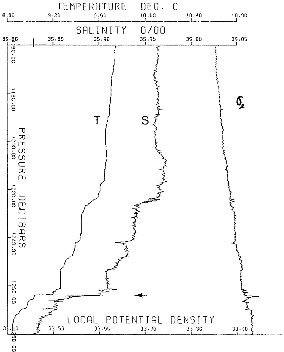
FIGURE 3.25 A section of the profile from SCIMP 1 showing the very sharp interface at 1264 db and its relation to the salinity maximum at 1209 db. The shadowgraphs from this interface have very distinct bands. The arrow is at the point where the bands are strongest.
