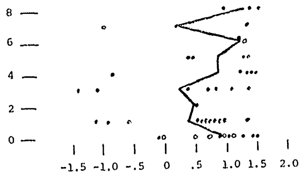
b) ds/dz \times 10^6 (1/m)
