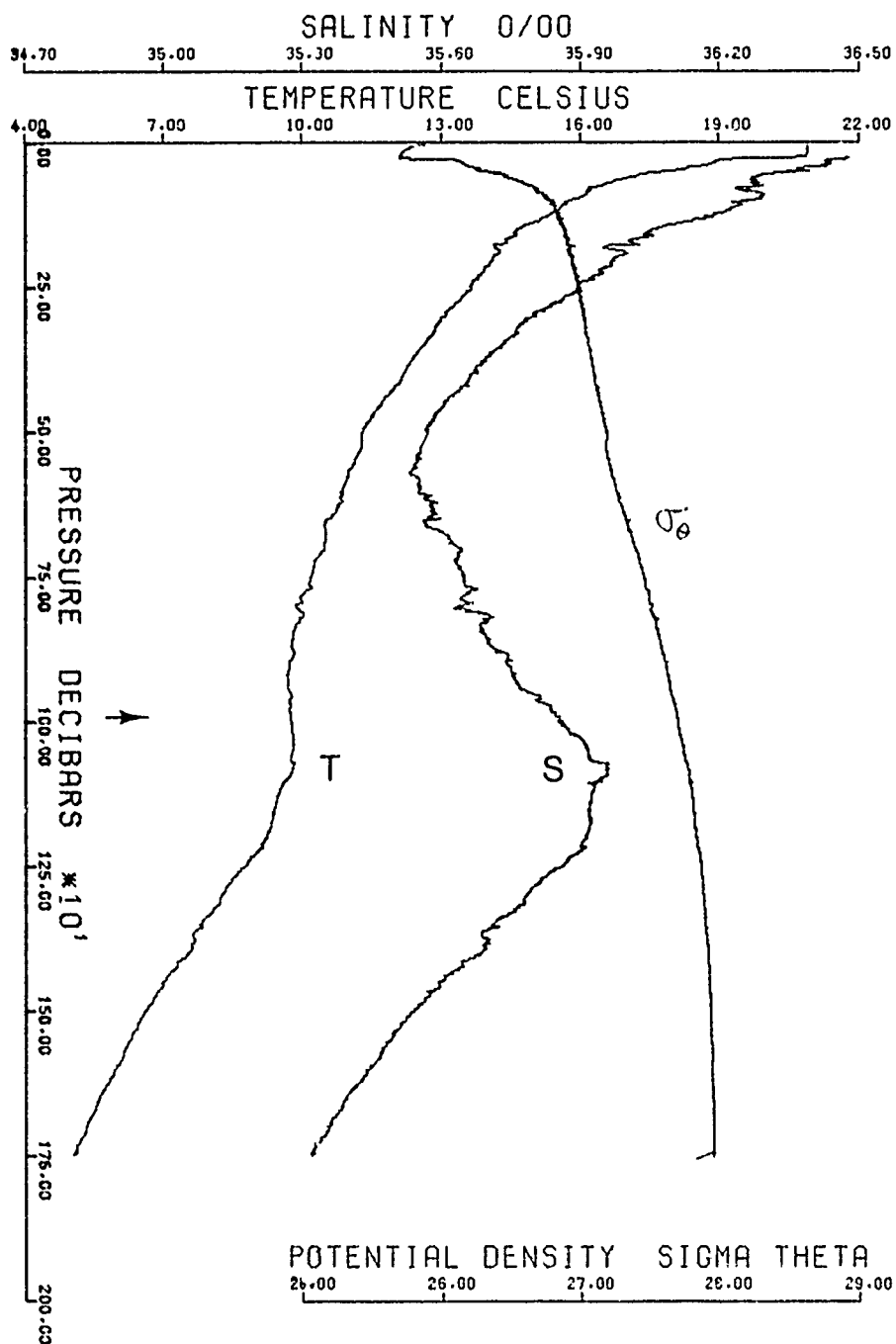
FIGURE 3.7 Profiles of temperature, salinity, and potential density for SCIMP 3. Launch at 0710Z, 19 July 1973; 34-06.0°N, 11-09.1°W. The arrow indicates where the OSFD was turned on.
