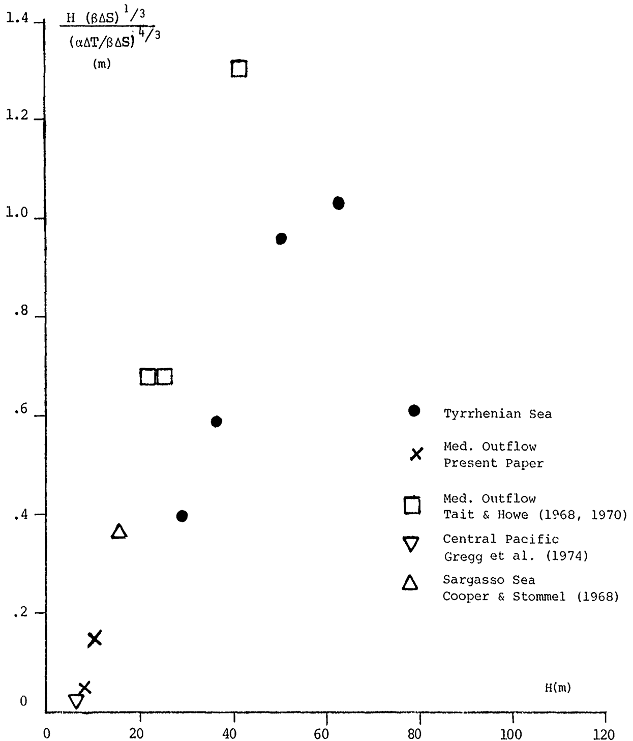
FIGURE 3.32 Evaluation of dimensionless layer thickness calculated for salt finger convection. The abscissa is the measured layer thickness for examples of regularly spaced steps where the gradients allow salt finger convection. If the measurements supported the theory, the value of the ordinate for the points would be a constant.
