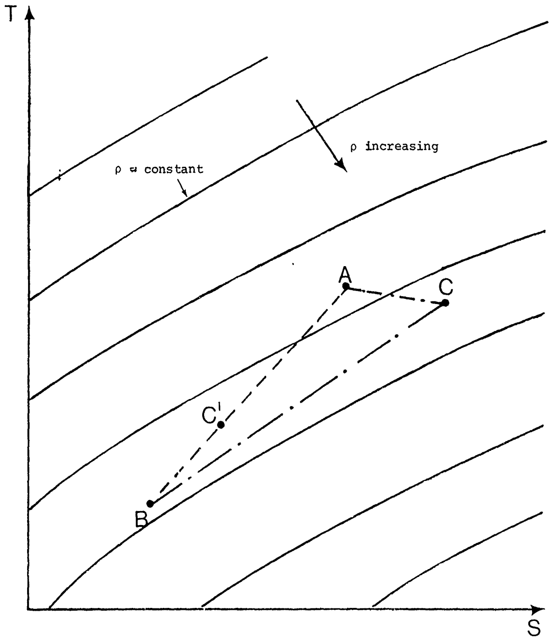
FIGURE 1.1 Schematic T-S plot. Each point is a particular water type and a straight line connecting two points represents all combinations of the two water types at the end points. Lines of constant density are also shown with an increase toward the lower right.
