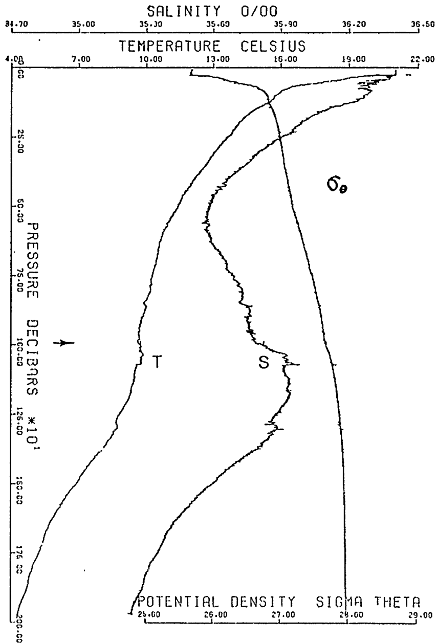
FIGURE 3.8 Profiles of temperature, salinity, and potential density for SCIMP 4. Launch at 0340Z, 20 July 1973; 34-14.0°N, 10-51.2°W. The arrow indicates where the CSFD was turned on.
