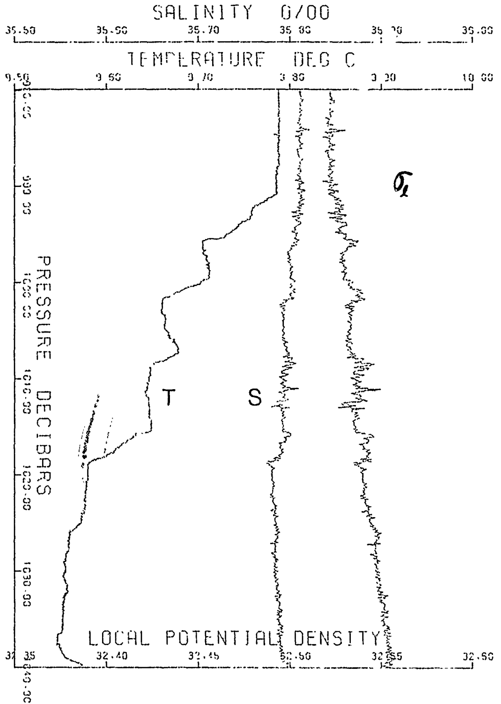
FIGURE 3.28 Series of steps below a secondary salinity maximum from SCIMP 1. At the bottom of the steps the salinity begins to increase.
