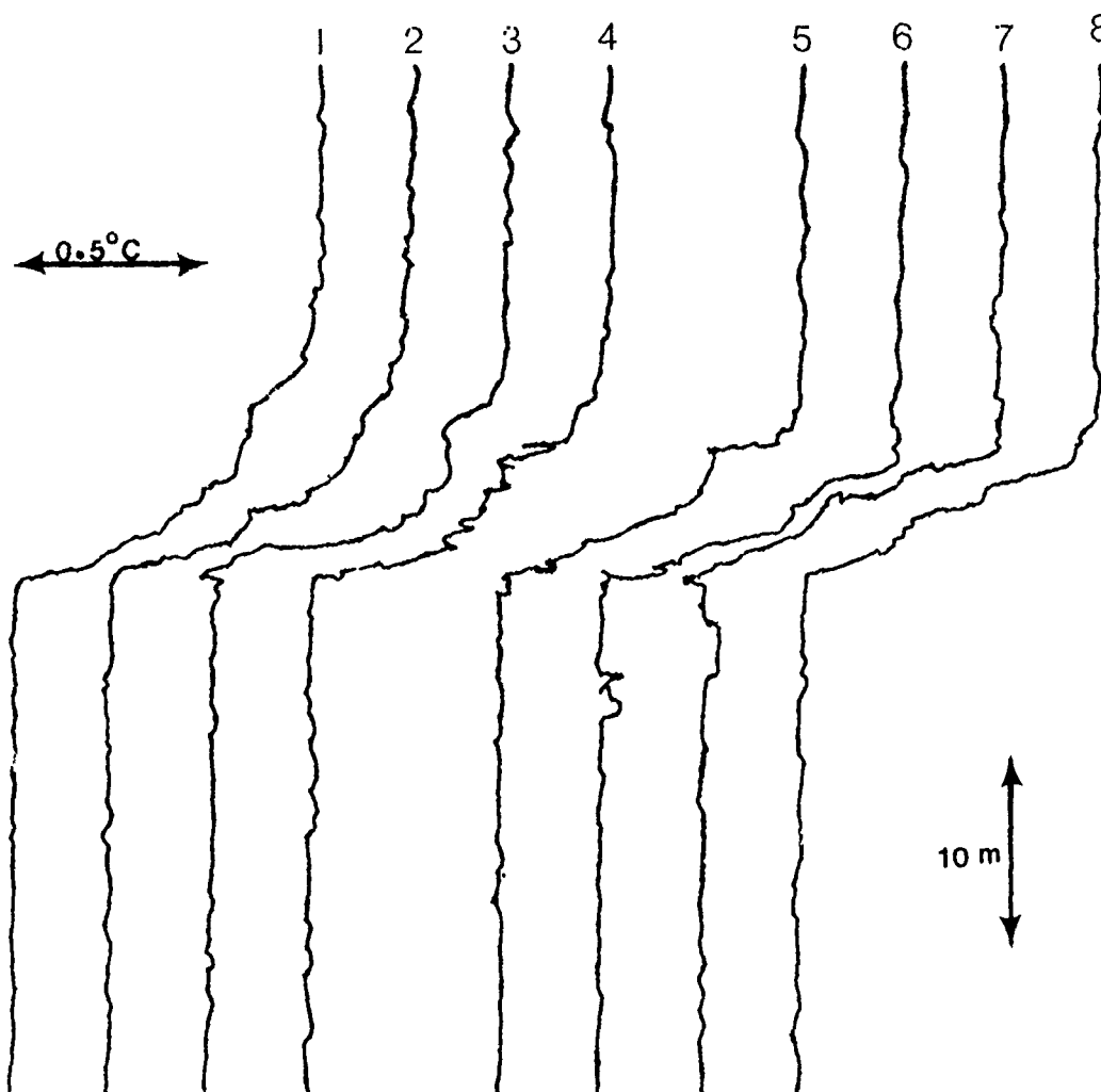
FIGURE 3.34 Potential temperature profiles for interface near 780 decibars in Figure 3.33. Each profile has been positioned so that the bottom edge is at the same level and offset 0.02 C. There is an additional offset of 0.02 C between the two groups of four.
