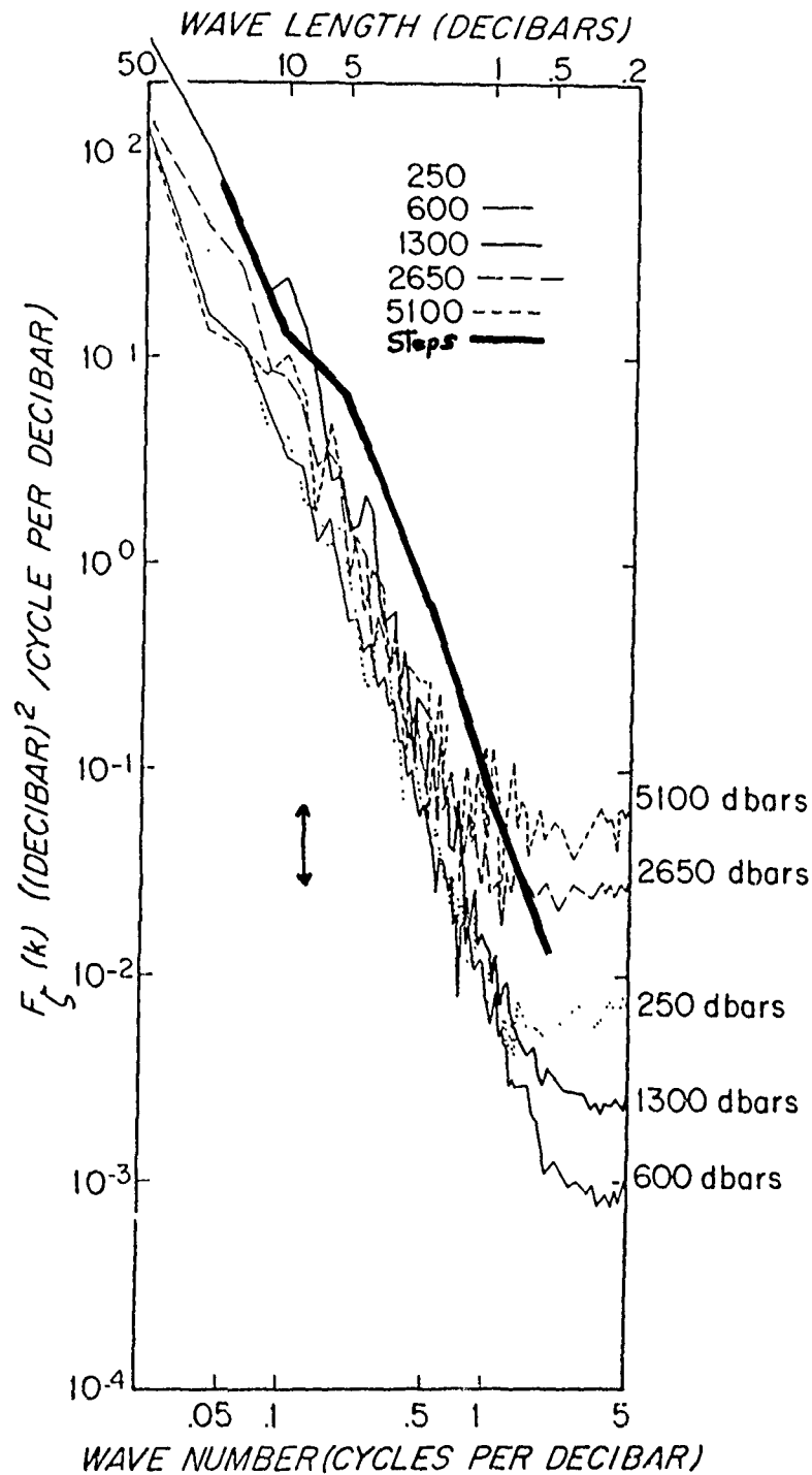
FIGURE 3.19 Vertical displacement spectra for stepped structure compared to various depths in the Sargasso Sea (Hayes et al., 1975). The spectrum from the steps has a higher level throughout except for very low wavenumber in the Mediterranean Water (1300 dbar) and for very high wavenumber where the spectra are dominated by noise. The bar indicates 90% confidence limits.
