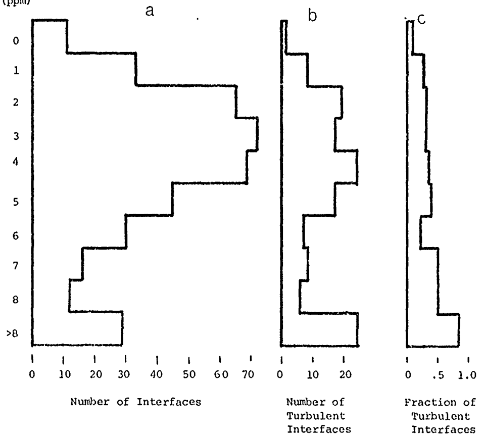
FIGURE 3.12 Distributions of interfaces and turbulent interfaces as a function of density difference across an interface. The fraction of turbulent interfaces is shown on the right.
