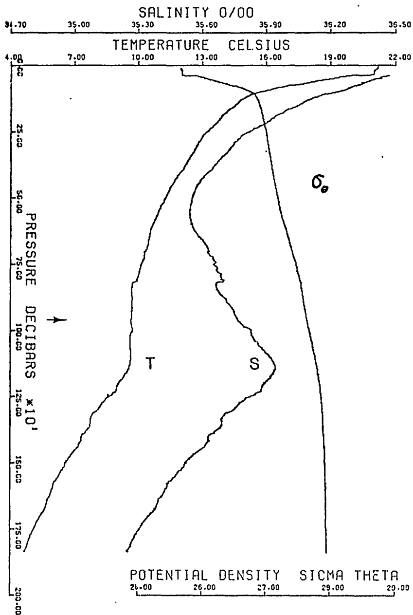
FIGURE 3.9 Profiles of temperature, salinity, and potential density for SCIMP 5. Launch at 1817Z, 20 July 1973; 34-22.5°N, 11-14.5°W. The arrow indicates where the CSFD was turned on.
