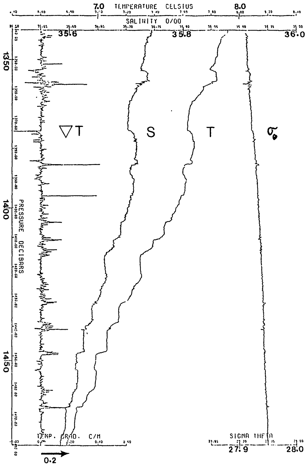
FIGURE 3.30 Weak inversion and steps below from SCIMP 3. The steps are the same as those in Figure 3.29. The layering appears to be the result of salt finger convection. The warm, saline intrusion increases the mean salinity gradient below, stimulating the convection.
