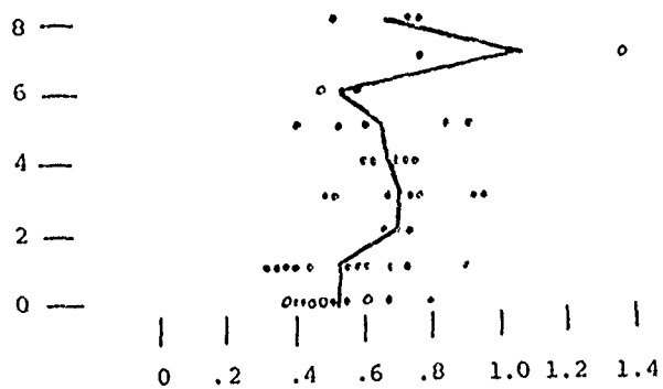
c) N^2 \times 10^5 (1/s 2 )
