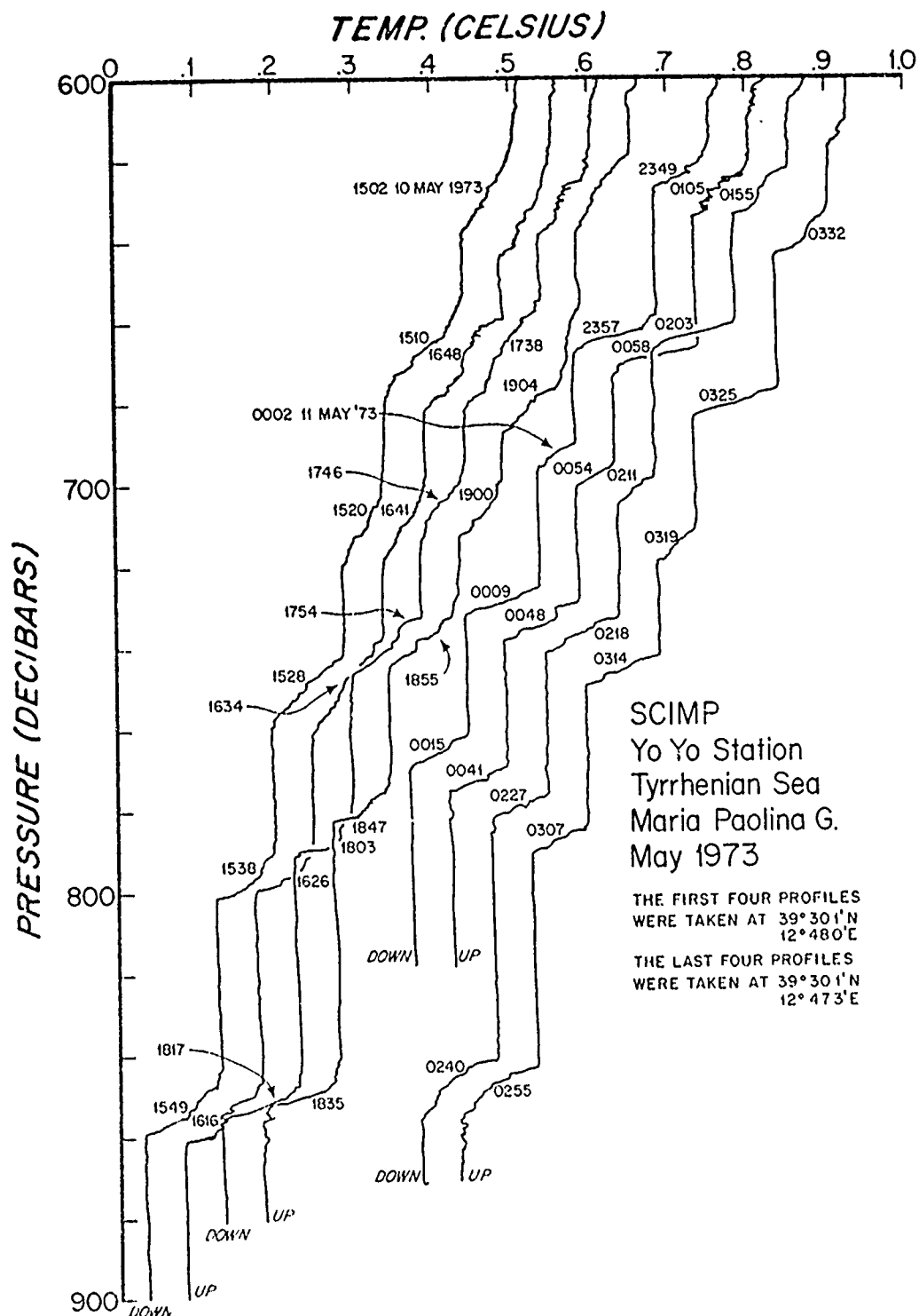
FIGURE 3.33 Composite of temperature profiles through stepped structure. Each profile is offset 0.05 C with an additional 0.05 C between the two groups of four. The numbers beside the interfaces are the time. This figure is an excerpt from Molcard and Williams, 1975.
