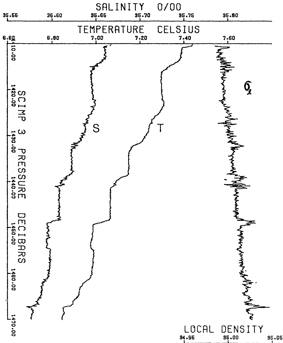
FIGURE 3.29 Series of steps from SCIMP 3. These layers appear to be more homogeneous than those in Figure 3.28.
