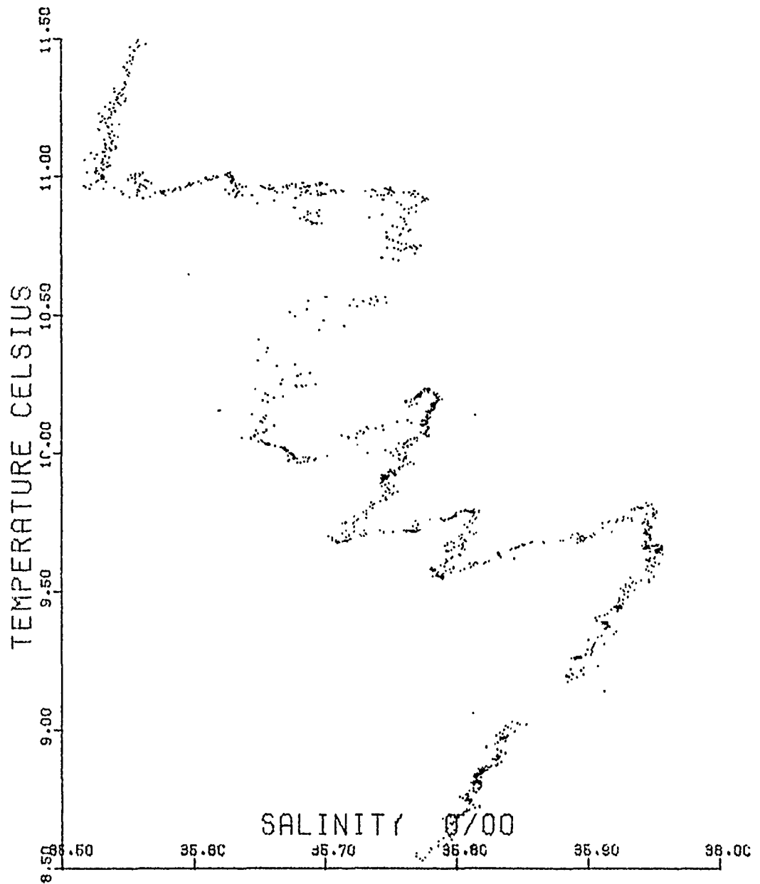
FIGURE 3.22 T-S plot for SCIMP 1 covering the depth interval 500-1300 m. The jagged appearance of the curve shows that the water column at this level is formed by a complex interleaving of layers with different T-S characteristics.
