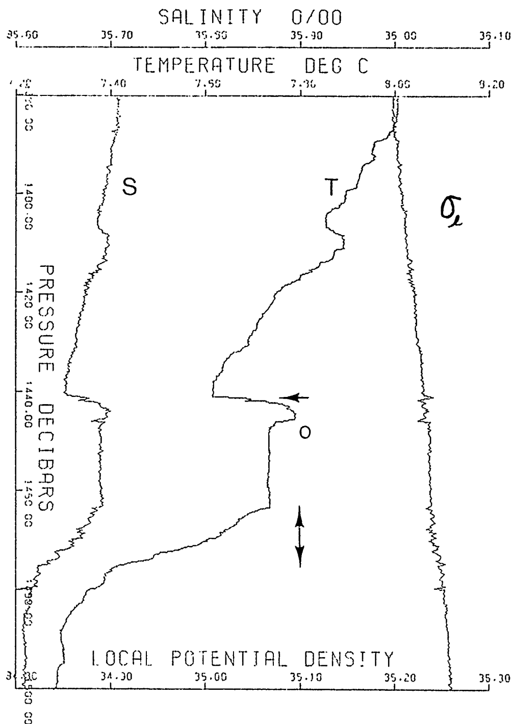
FIGURE 3.23 Warm, salty intrusion from SCIMP 1. On the shadowgraphs there are bands at the top of this intrusion and a long sequence of bands and turbulence on the underside. At the point marked with an O, there are no images even though the conditions are correct for salt fingers.
