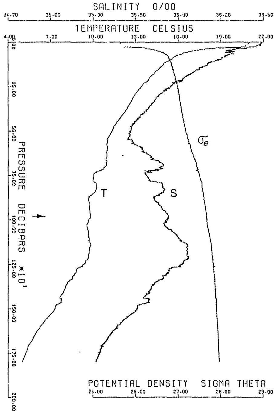
FIGURE 3.6 Profiles of temperature, salinity, and potential density for SCIMP 1. Launch at 0930Z, 16 July 1973; 34-58.4°N, 10-28.1°W. The arrow indicates where the OSFD was turned on.
