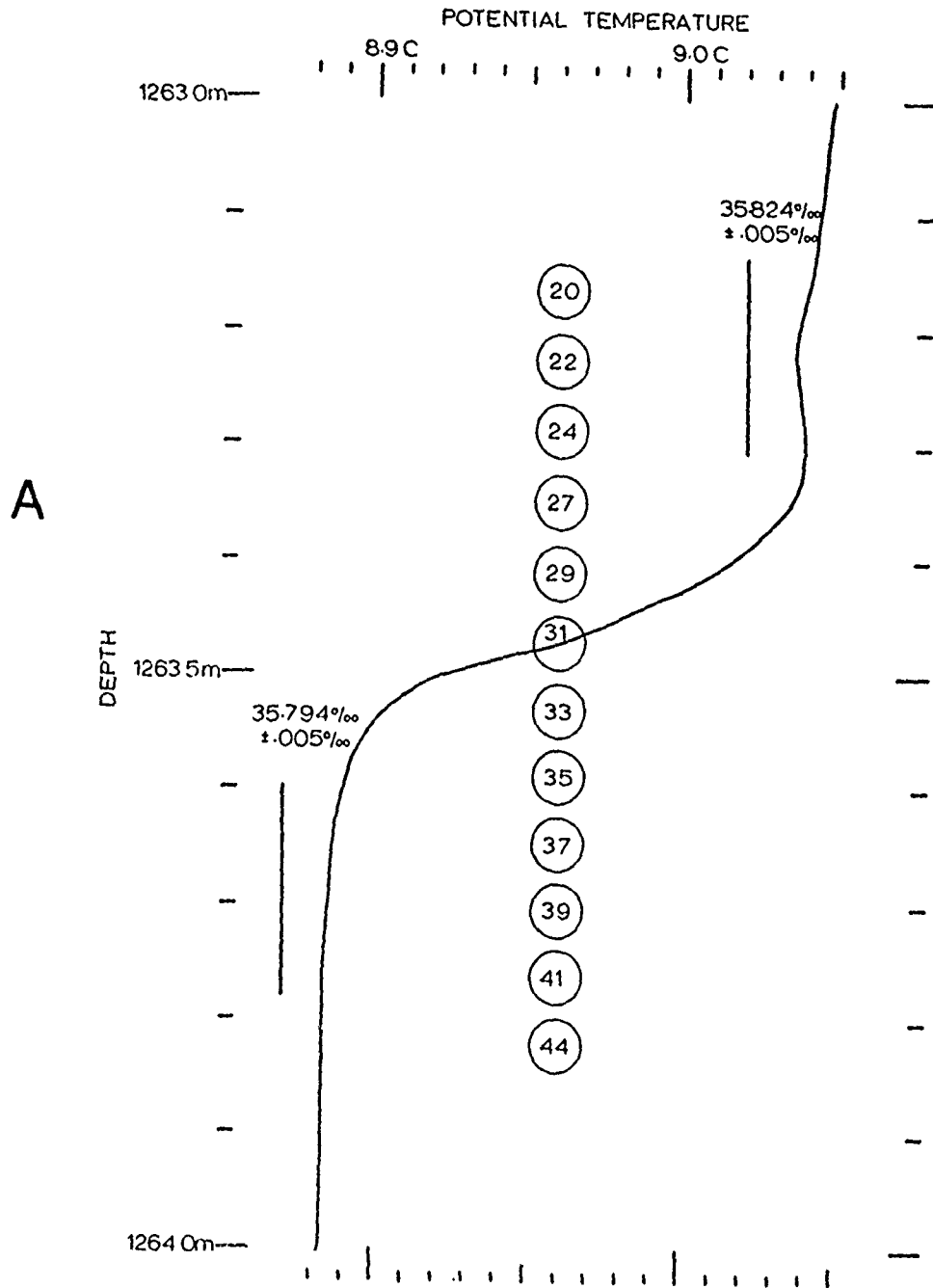
FIGURE B-1 Potential temperature profile of interface from SCIMP 1. This interface is also plotted in Figure 3.25. The circled numbers indicate the positions of shadowgraphs relative to the profile. This graph is an excerpt from Williams, 1974.
