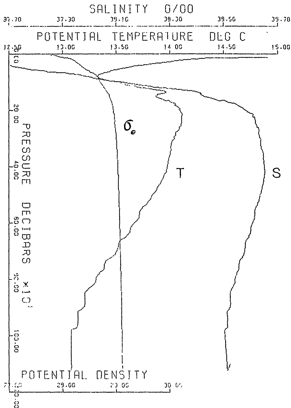
FIGURE 3.31 Profiles of temperature, salinity, and potential density from the Tyrrhenian Sea. The stepped structure is prominent below 700 decibars. The layer thickness increases with depth to more than 100 m.
