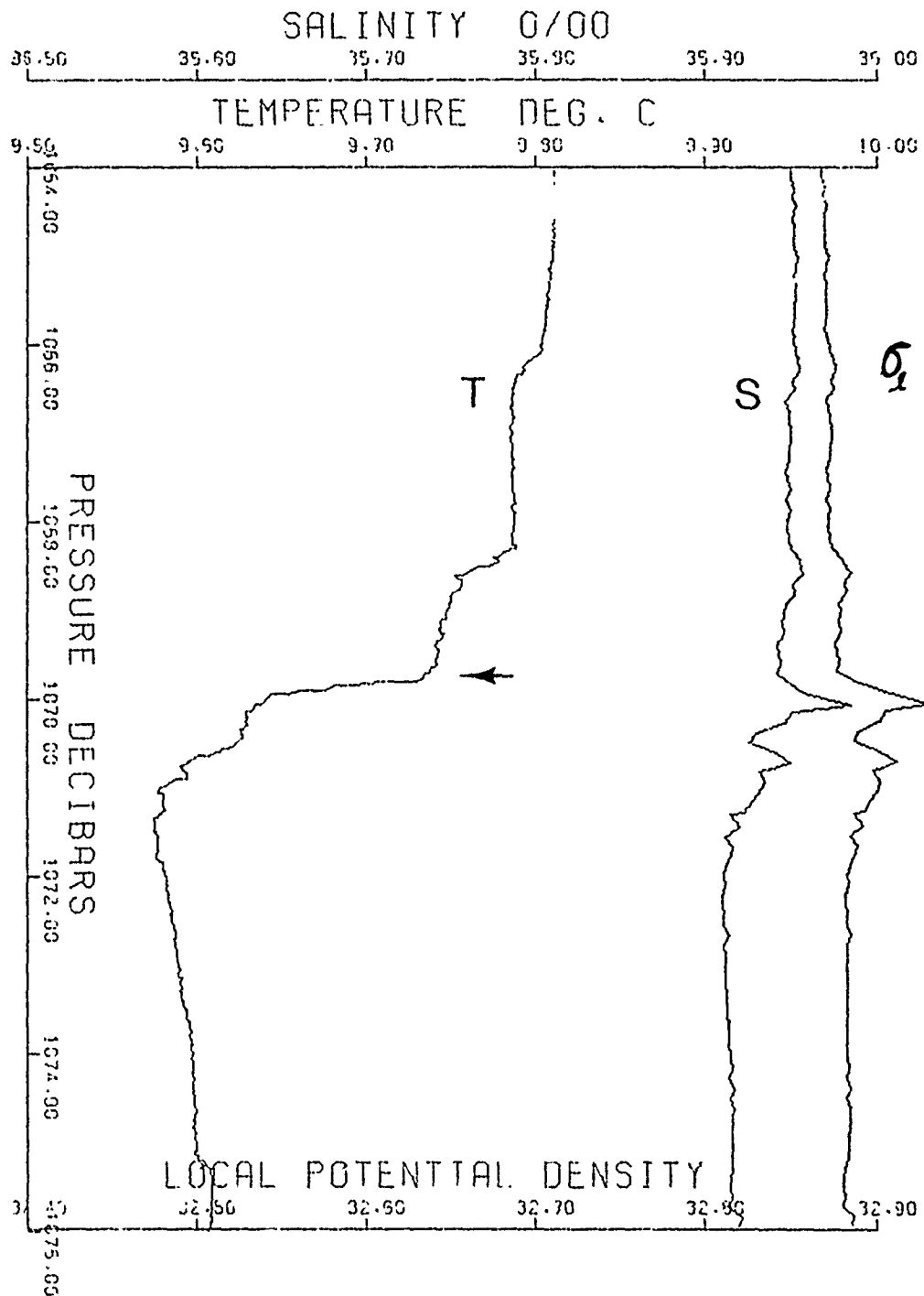
FIGURE 3.26 Interface just below deep salinity maximum from SCIMP 4. The arrow marks the point where the shadowgraph images have highest contrast.
