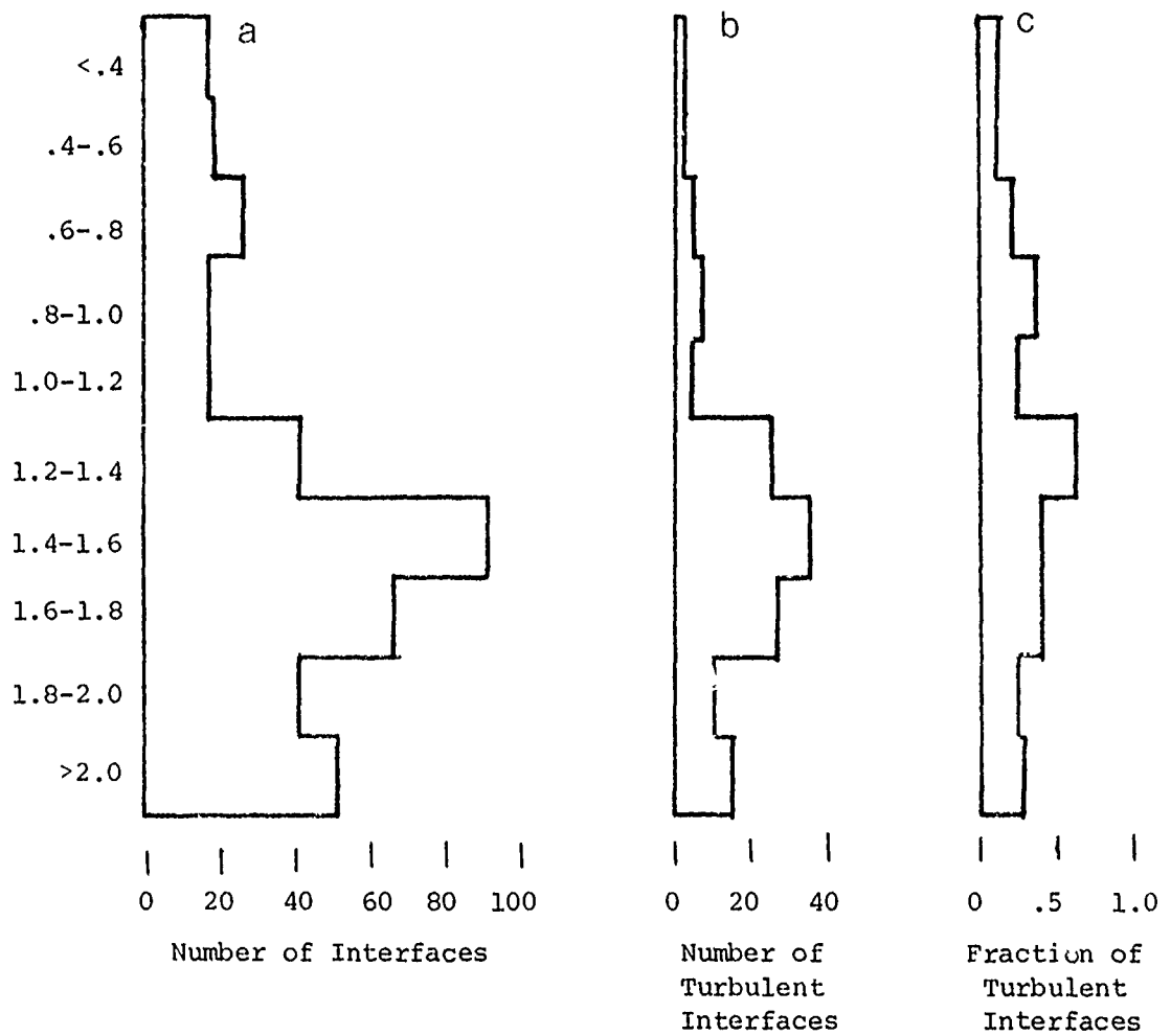
FIGURE 3.14 Distributions of interfaces and turbulent interfaces as a function of Turner Number, Tu = \alpha\Delta T/\beta\Delta S . The fraction of turbulent interfaces is shown on the right.
