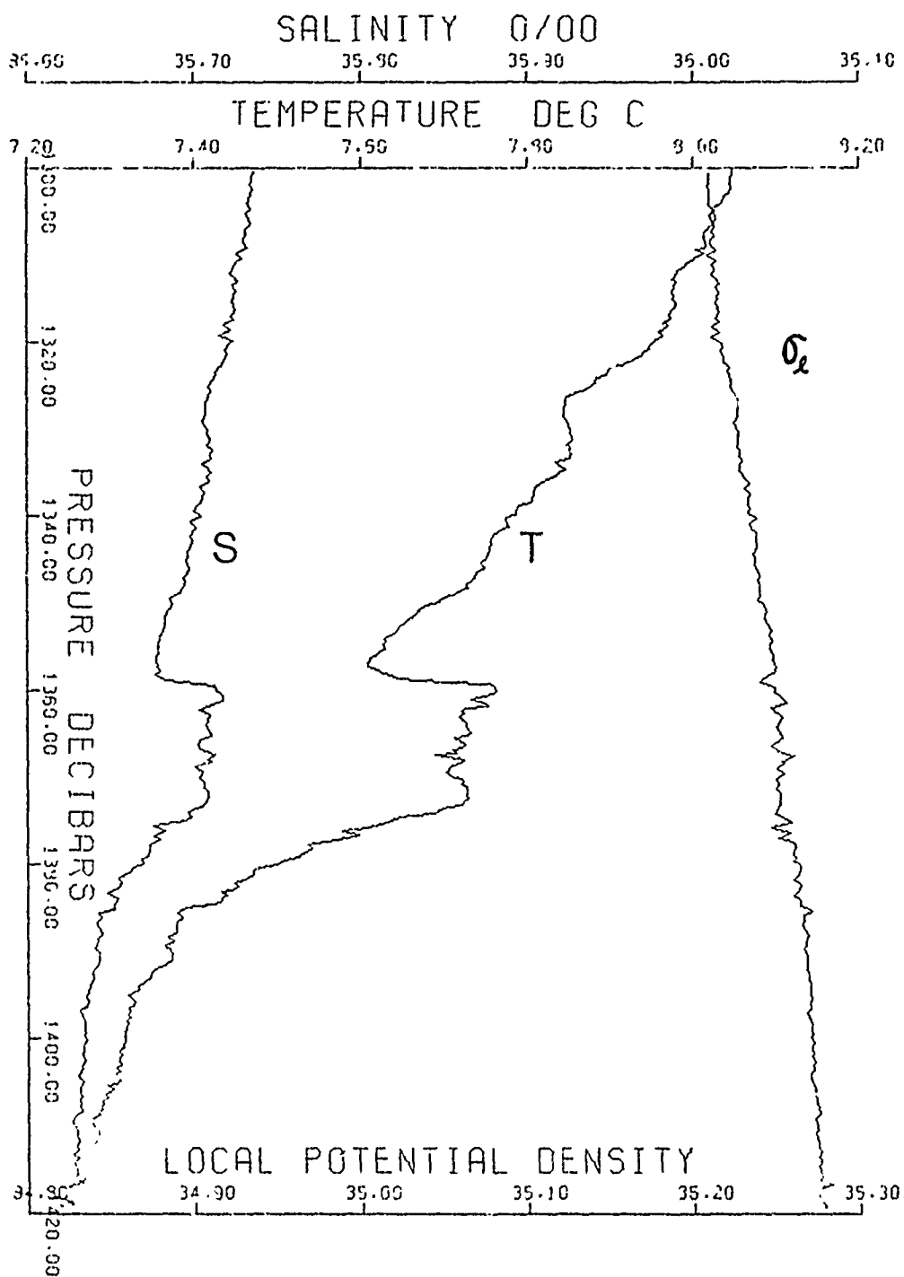
FIGURE 3.24 Warm, salty intrusion from the ascending portion of SCIMP 1. Although similar in many respects to the intrusion in Figure 3.23, there are several significant differences.
