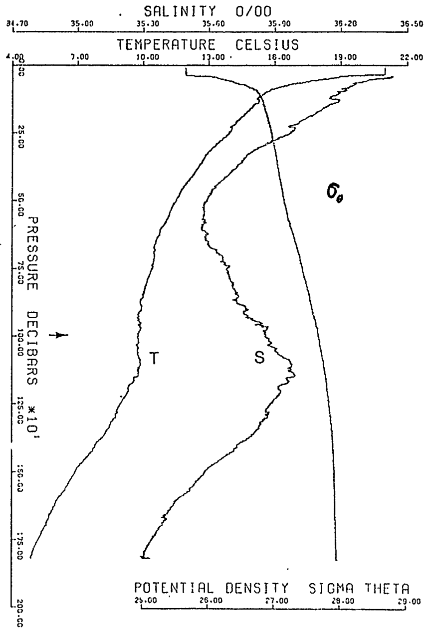
FIGURE 3.10 Profiles of temperature, salinity, and potential density for SCHIP 6. Launch at 0923Z, 21 July 1973; 34-15.0°N, 10-50.0°W. The arrow indicates where the CGFD was turned on.
