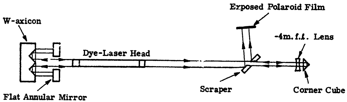
(a) Arrangement for Near-Field Observation
