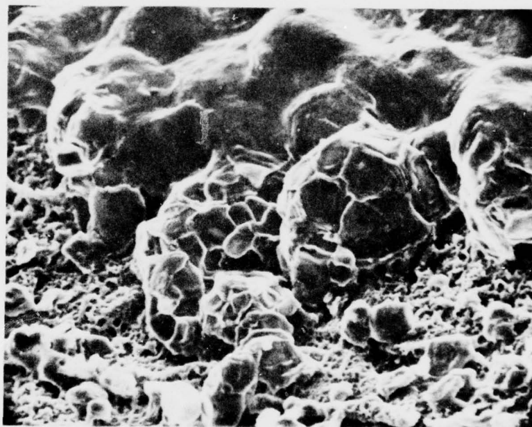
Figure 74. Surface Structure of Lithium When Stored in 1.0M \text{LiAlCl}_4 \cdot \text{SOCl}_2 at 165^\circ\text{F} for 11 Days
