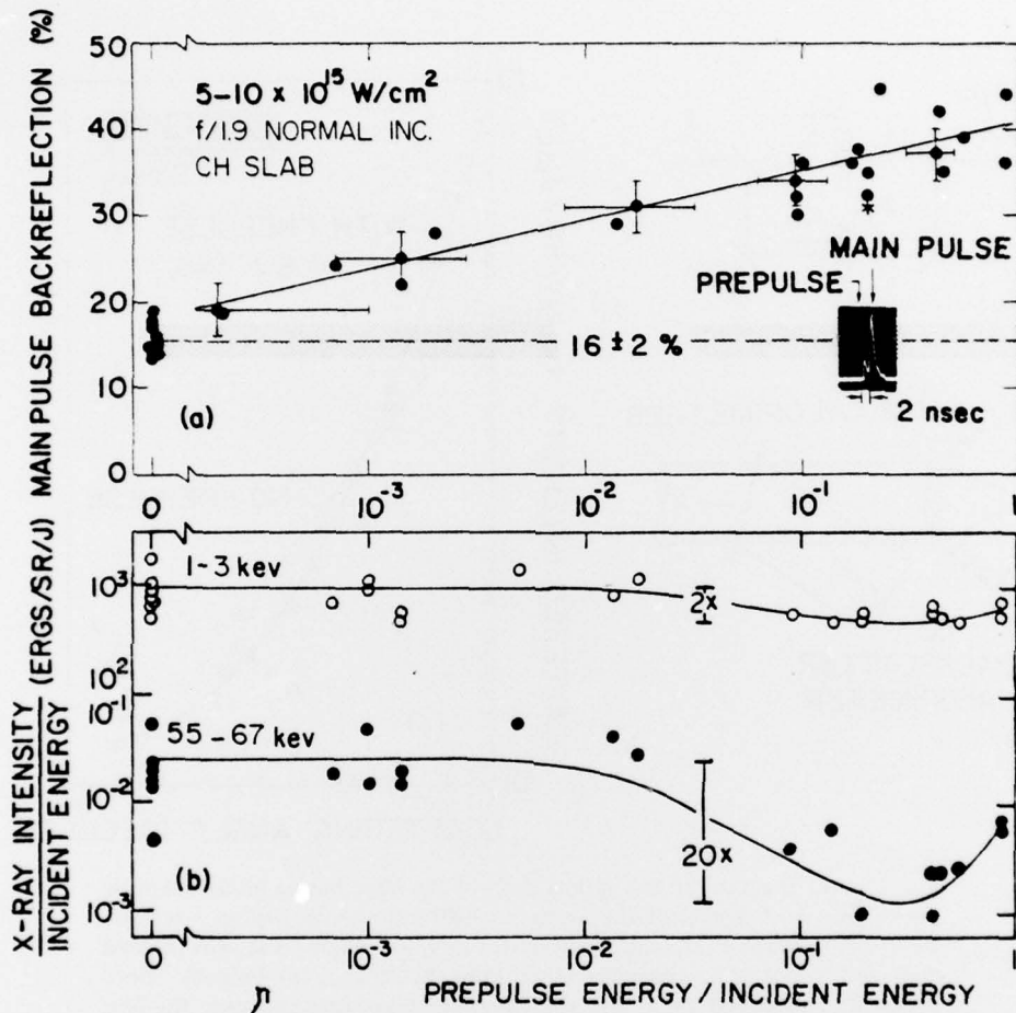
Fig. 2 - (a) Backreflections of the main pulse versus prepulse level showing enhanced backscatter for \eta \geq 10^{-4} . Hashed region is the single pulse backreflection. (b) X-ray intensities for 1-3 keV and 55-67 keV x-rays versus prepulse level illustrating the decrease in intensity and spectral hardness of x-rays with increasing \eta . (Increase in intensity for \eta approaching unity is due to x-ray emission induced by the prepulse itself.)
