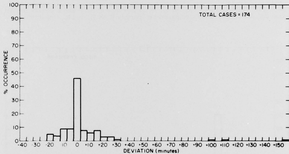
Figure A17. Histogram of Percentage of Occurrence of All Significant and Relevant Events for All Modes and All Experiments Compared Temporally With Q-Transition Occurrences
