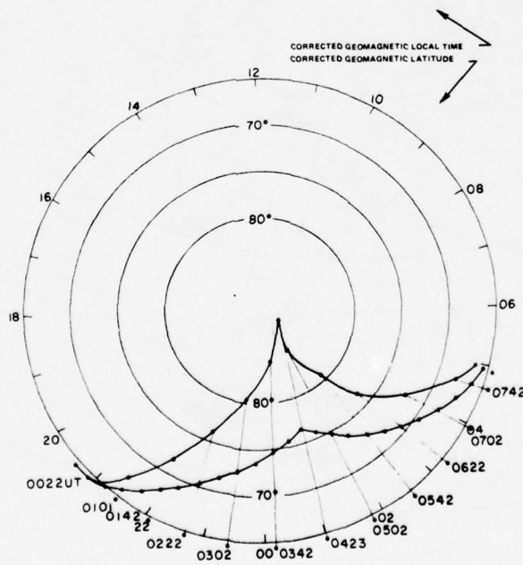
Figure 8. Flight Path of Experiment 60 in Corrected Geomagnetic Coordinates
