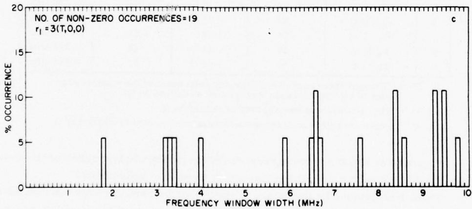
Figure 32. Histogram of the Frequency Window Widths for Each r_1 -Condition for the One-Hop E Mode for All Six Experiments
