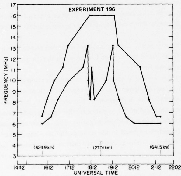
Figure A1. Elkins-Rush HF Polar Predictive Model, Service Probability = 0.70, 1-F Modes
