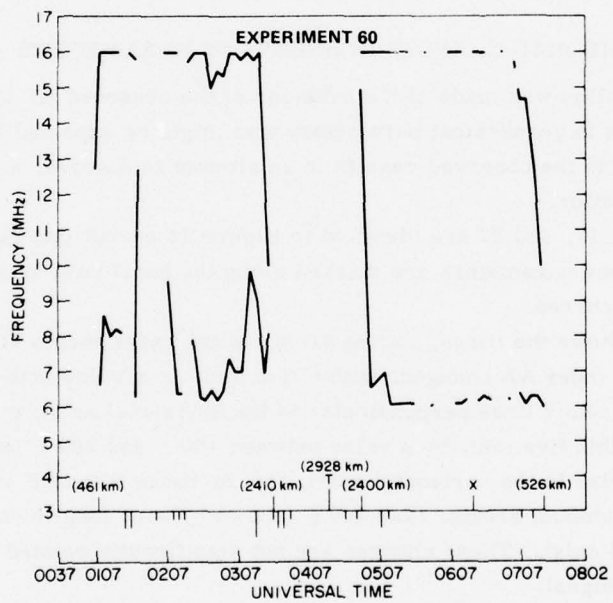
Figure 16. 1-E Modes Observed at Aircraft Showing Instantaneous Changes in the Index AE
