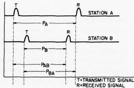
Figure 13. Timing Cycle
