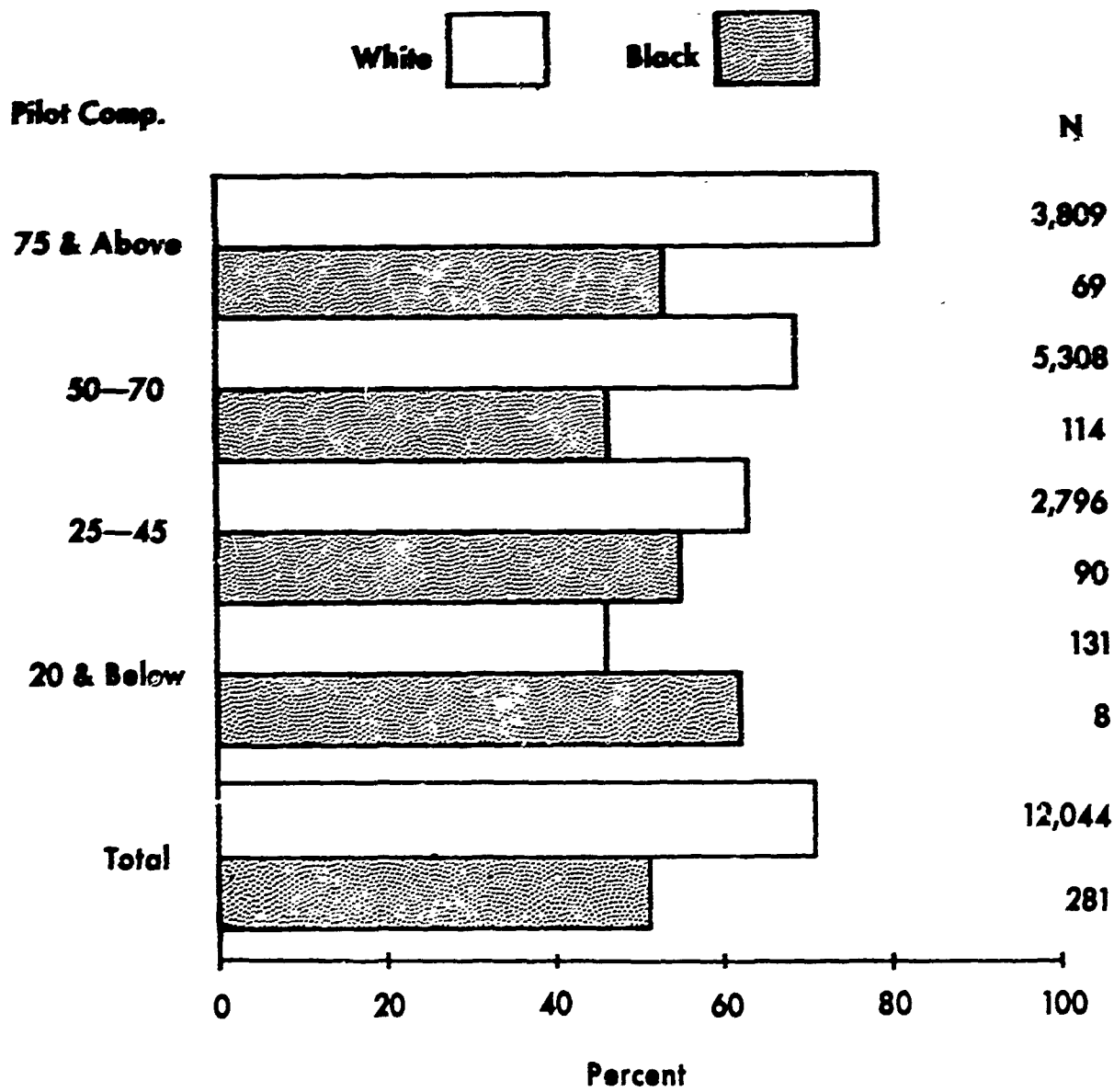
Figure 5. UPT graduation rates by levels of Pilot Composite scores.
