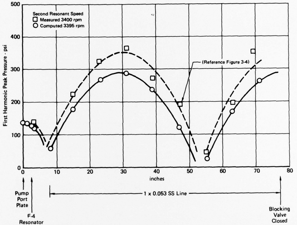
FIGURE 3-5 STANDING PRESSURE HALF WAVE, TEST STAND F-4 ABEX PUMP
