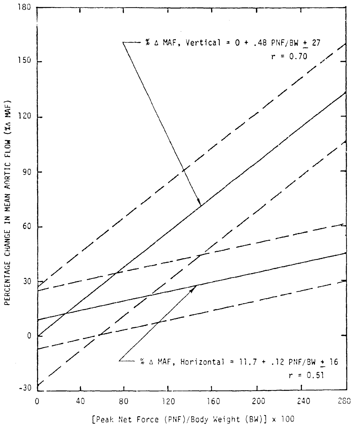
Fig. 4. Comparison of percentage change in mean aortic flow vs peak net force/body weight for animals restrained horizontally and vertically during g_2 vibration.
