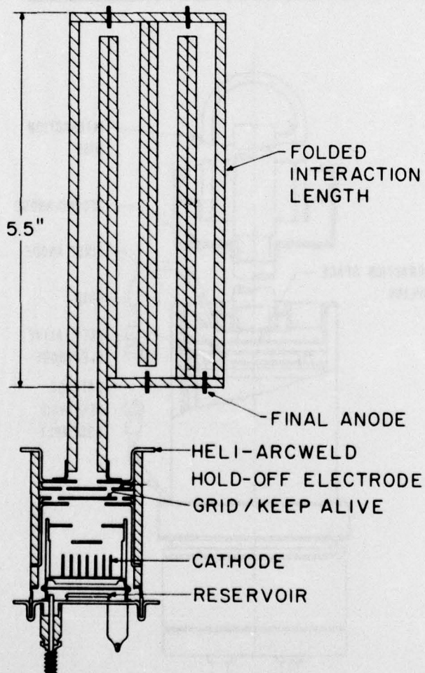
FIGURE 6. RSI DEVICE TYPE B
