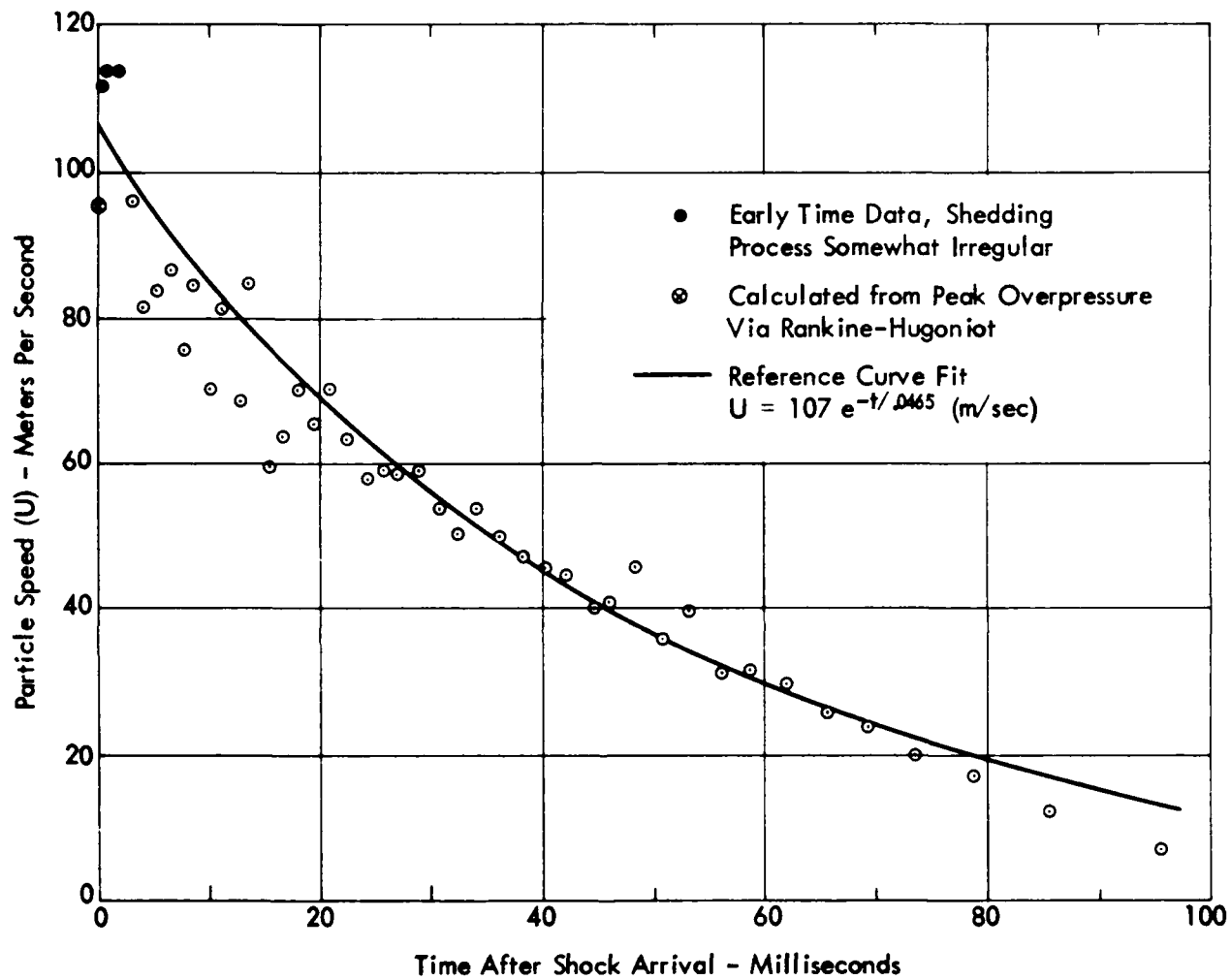
FIGURE 22 PARTICLE VELOCITY COMPUTED FROM VSA TRANSDUCER OUTPUT (20 TON TNT CHARGE, RANGE = 149 m)
