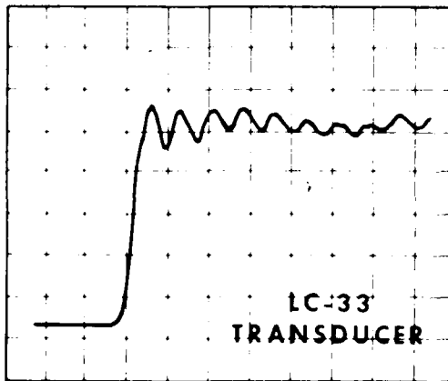
TYPICAL PRESSURE-TIME PROFILE
