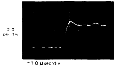
SHOCK TUBE End-On
