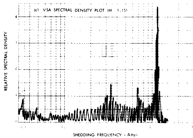
FIGURE 23 VSA SIGNAL SPECTRUM FOR VARIOUS MACH NUMBERS
