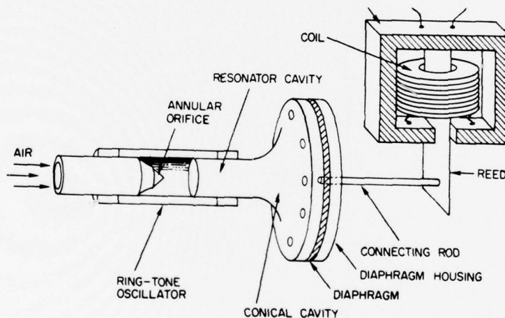
Figure 6. Fluidic generator with ring-tone oscillator.
