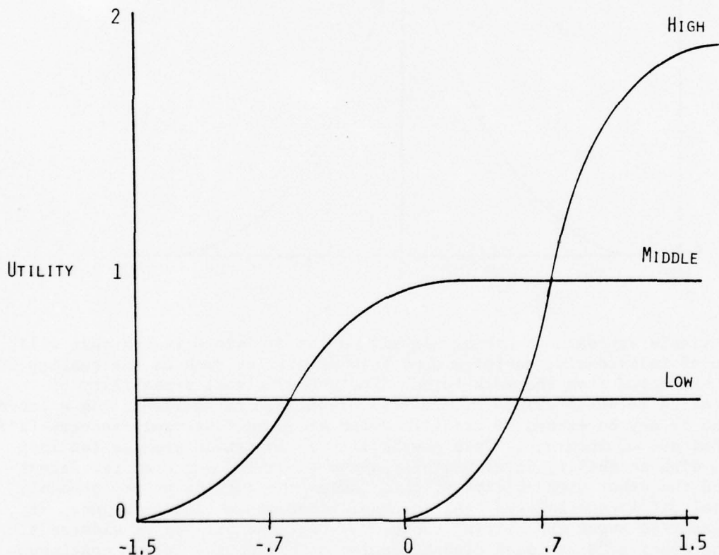
Figure 15 Conditional Utilities for each of Three Decisions
