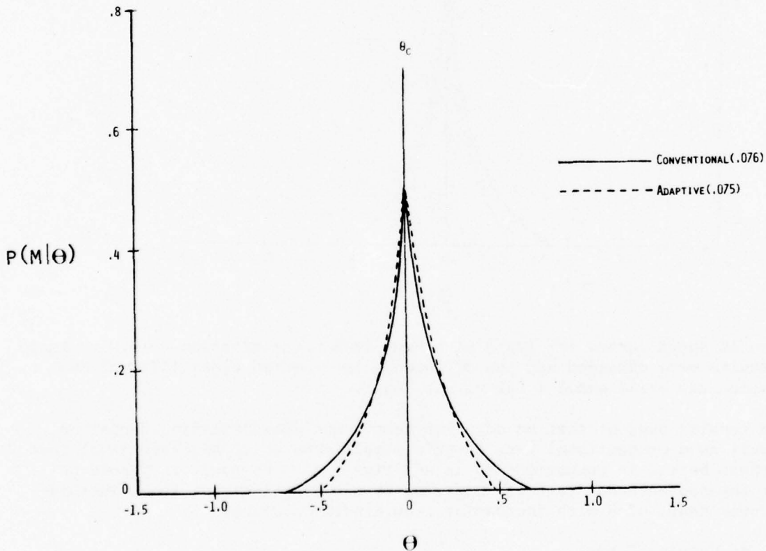
Figure 18 Conditional Probability of Misclassification, \alpha=2.0
