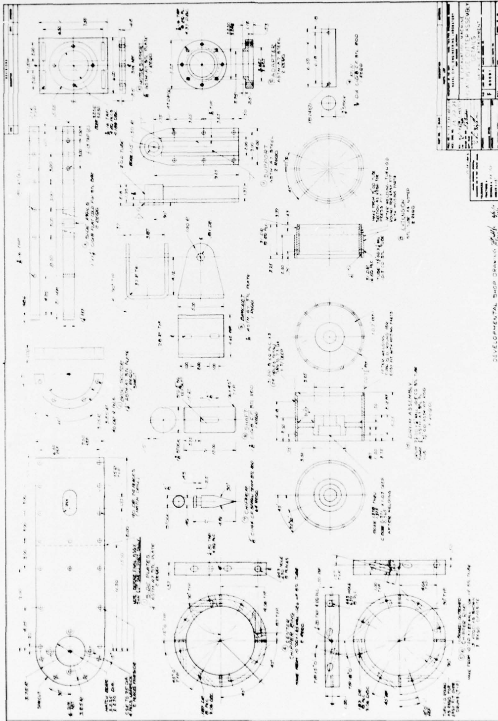
Figure 5. Fabrication Drawing 74-22-2F for rotating ice chipping drum assembly.
