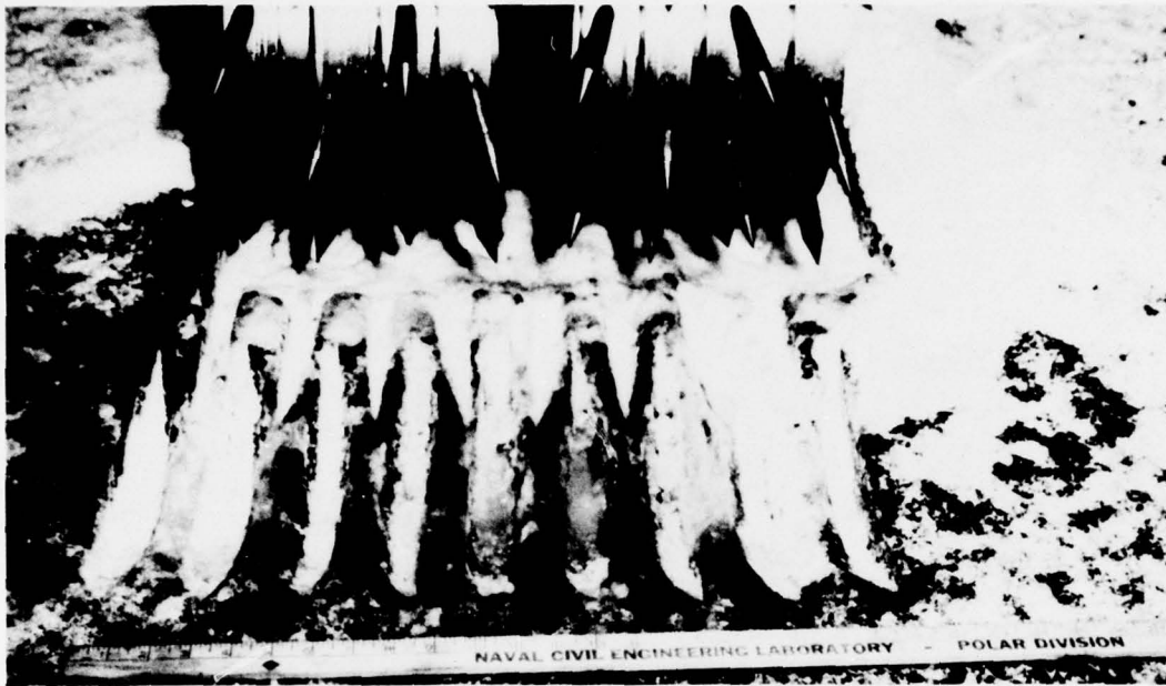
Figure 11. Chipping tests showing grooves left by 2-1/2-inch (6.4-cm) tooth spacing.
