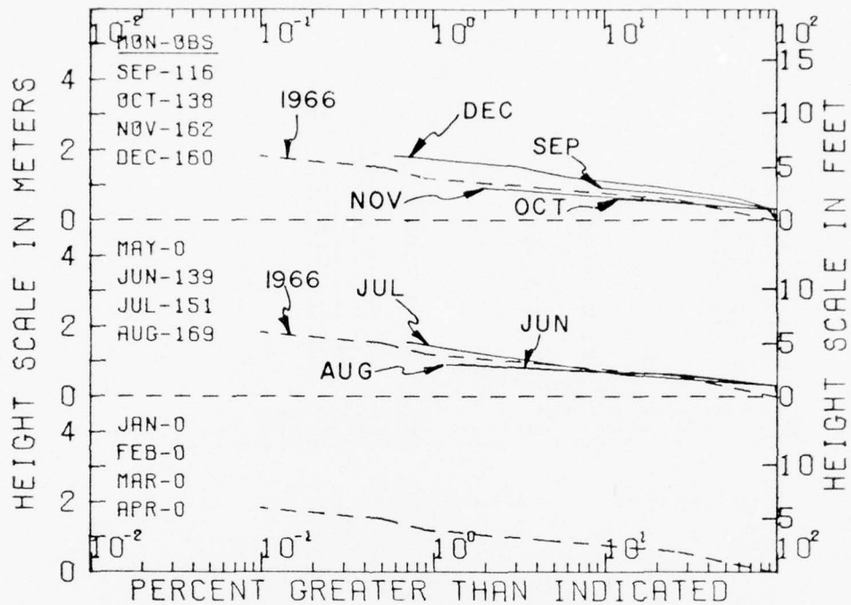
Figure A-S2. Seasonal summaries of cumulative height distributions from Pt. Conception, California. Determined from 7-minute pen and ink records taken six times daily. Wave heights may be low due to old gage design and maintenance difficulties.
