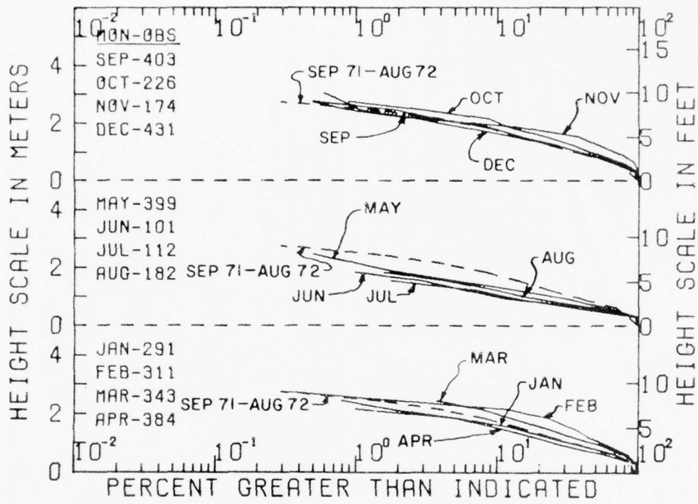
Figure A-32. Seasonal summaries of cumulative significant height distributions from Nags Head, North Carolina; computed from 1,024-second digital wave records taken four times daily.
