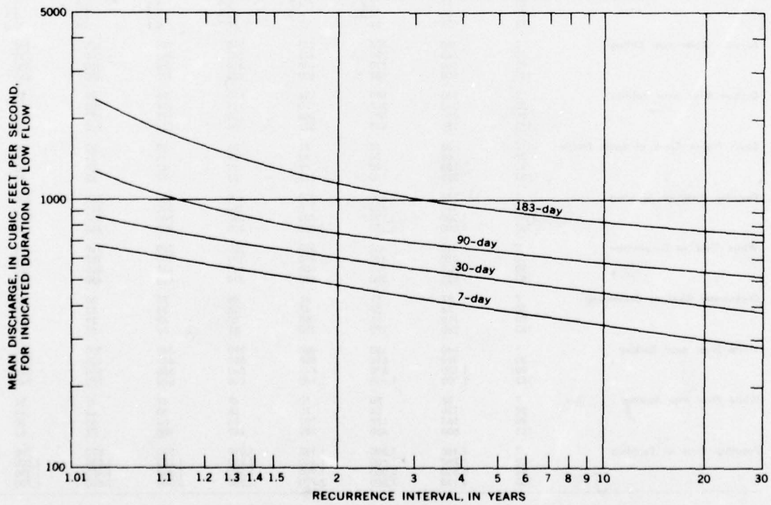
FIGURE 92.—Low-flow frequency, White River near Buckley, 1946-63.
