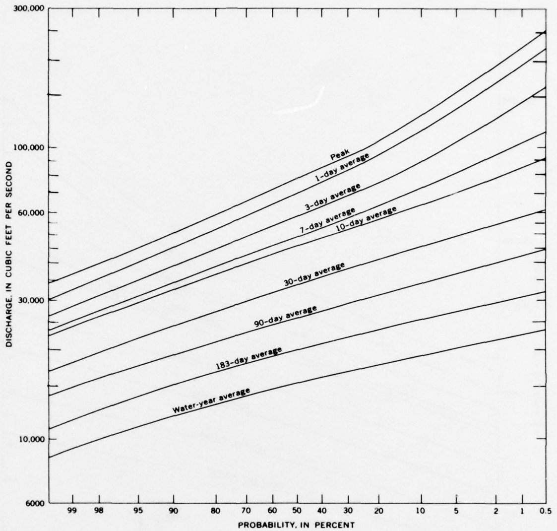
FIGURE 39.—Probability curves of annual maximum flows for specified time periods, Skagit River near Mount Vernon.
