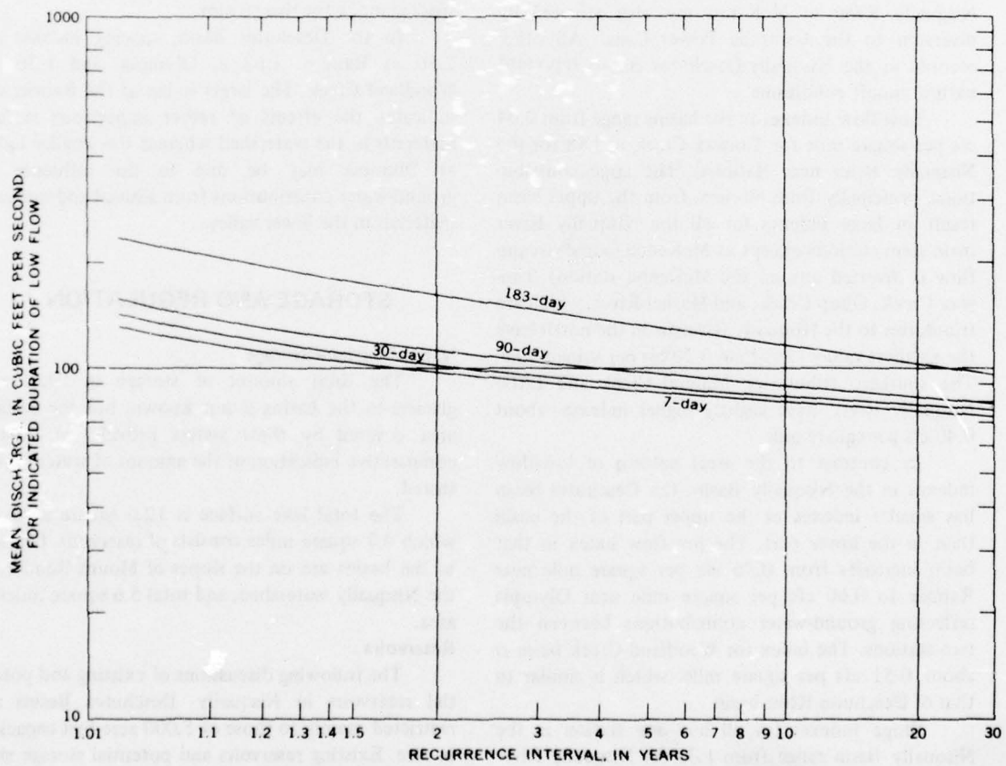
FIGURE 101.—Low-flow frequency, Deschutes River near Olympia, 1946-63.
