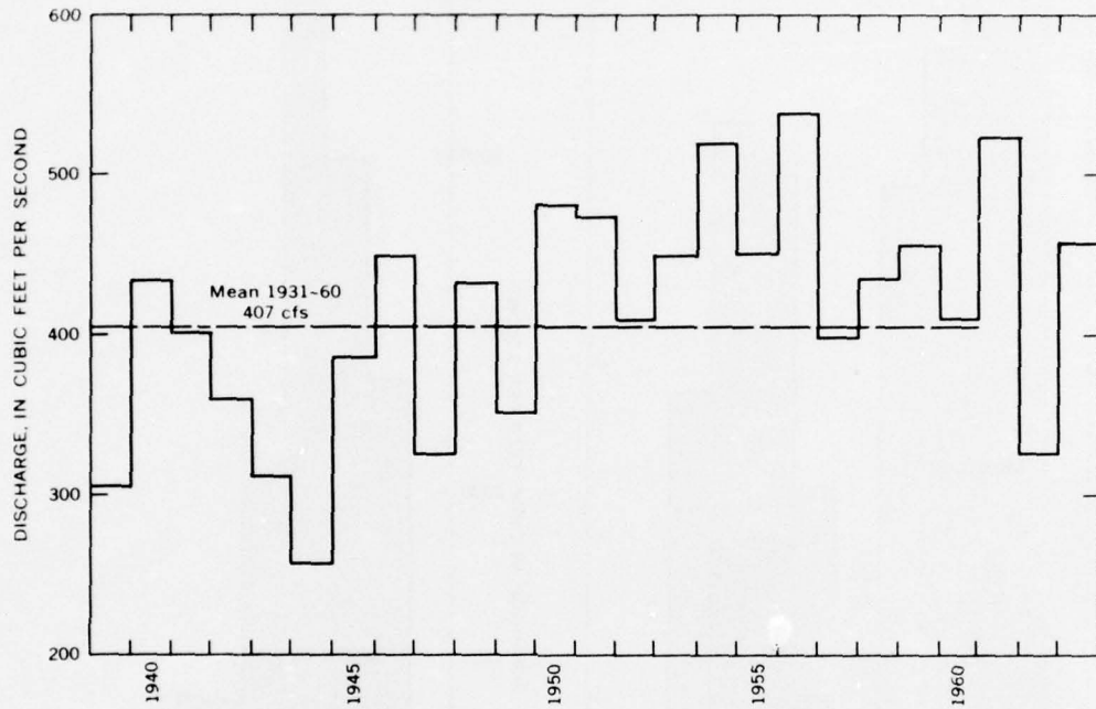
FIGURE 103.—Annual discharges, Duckabush River near Brinnon.
