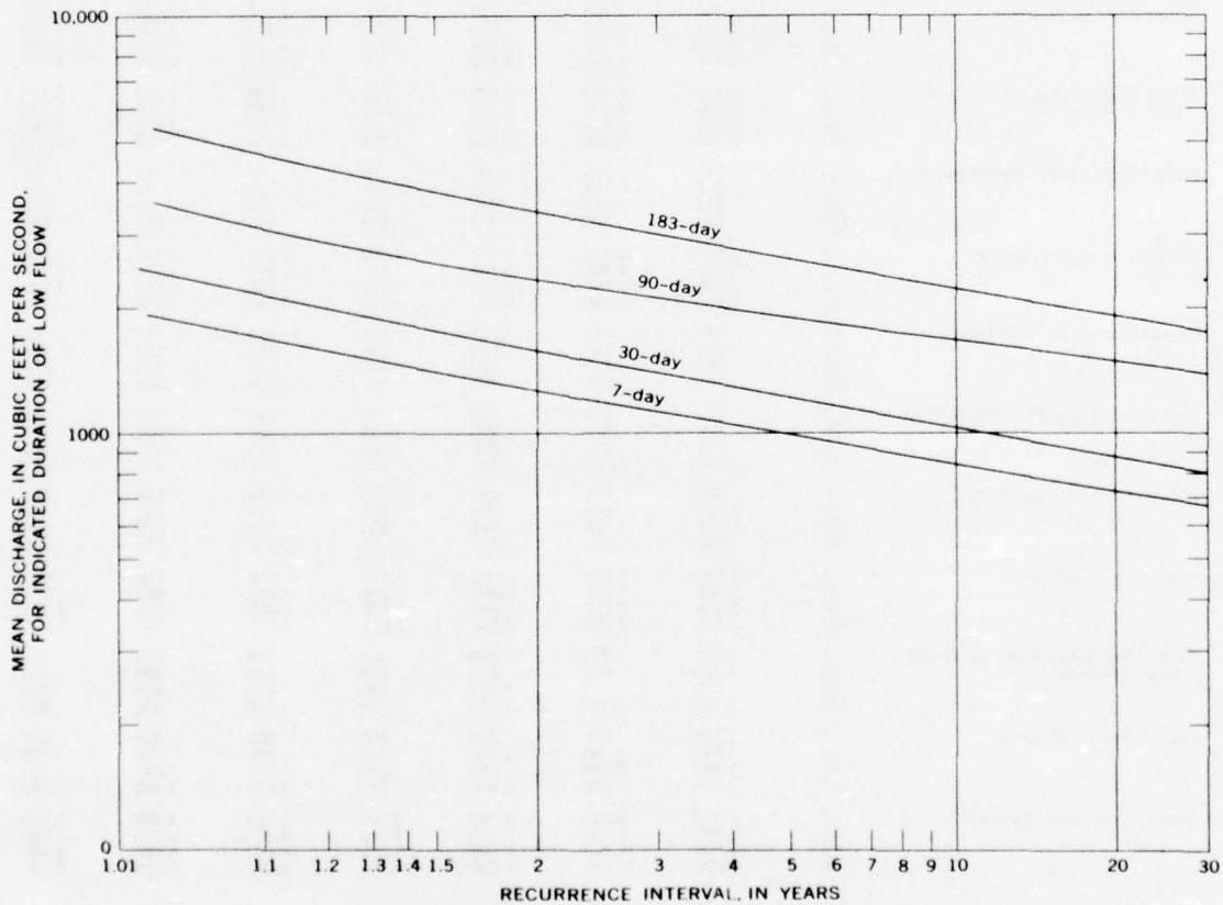
FIGURE 42.—Low-flow frequency, Sauk River near Sauk, 1946-63.
