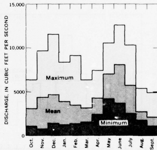
FIGURE 37.—Maximum, mean and minimum monthly discharges, Sauk River near Sauk, 1931-60.
