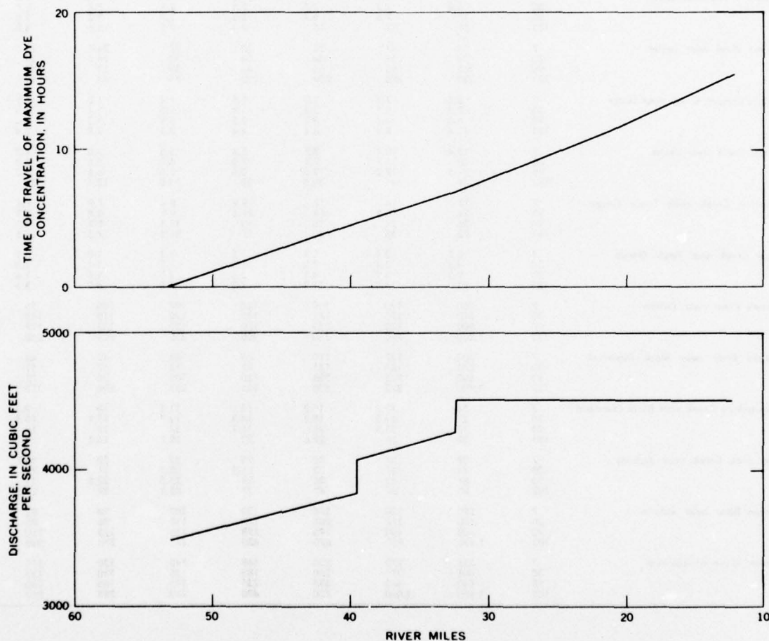
FIGURE 84.—Water discharge and time of travel of dye, Green River, April 20, 1965.
