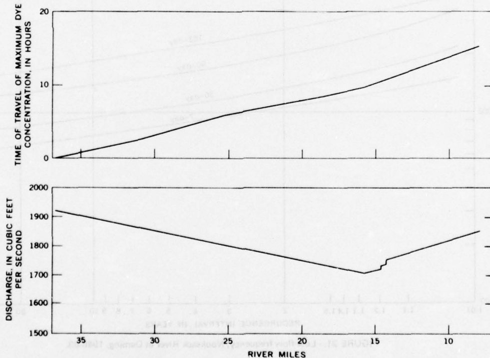
FIGURE 32.—Water discharge and time of travel of dye, Nooksack River, October 26-27, 1965.
