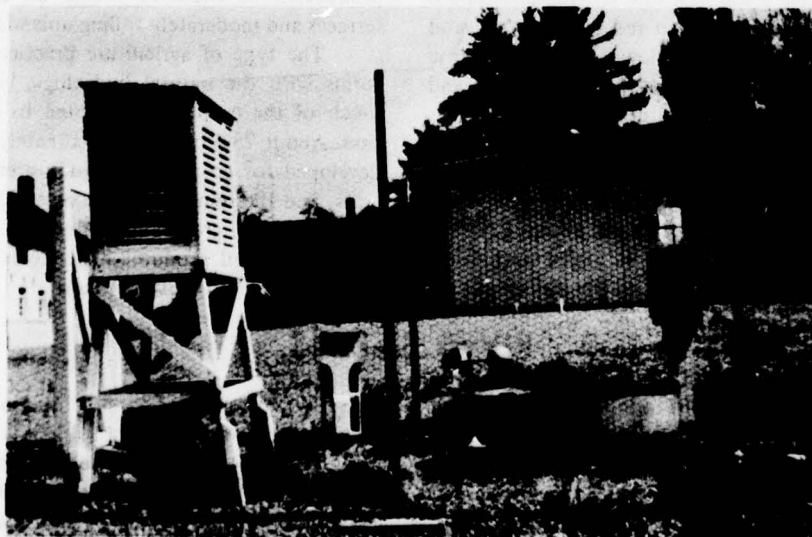
Weather Observing Station includes rain gage, evaporation pan, anemometer and instrument shelter for exposing thermometers.
