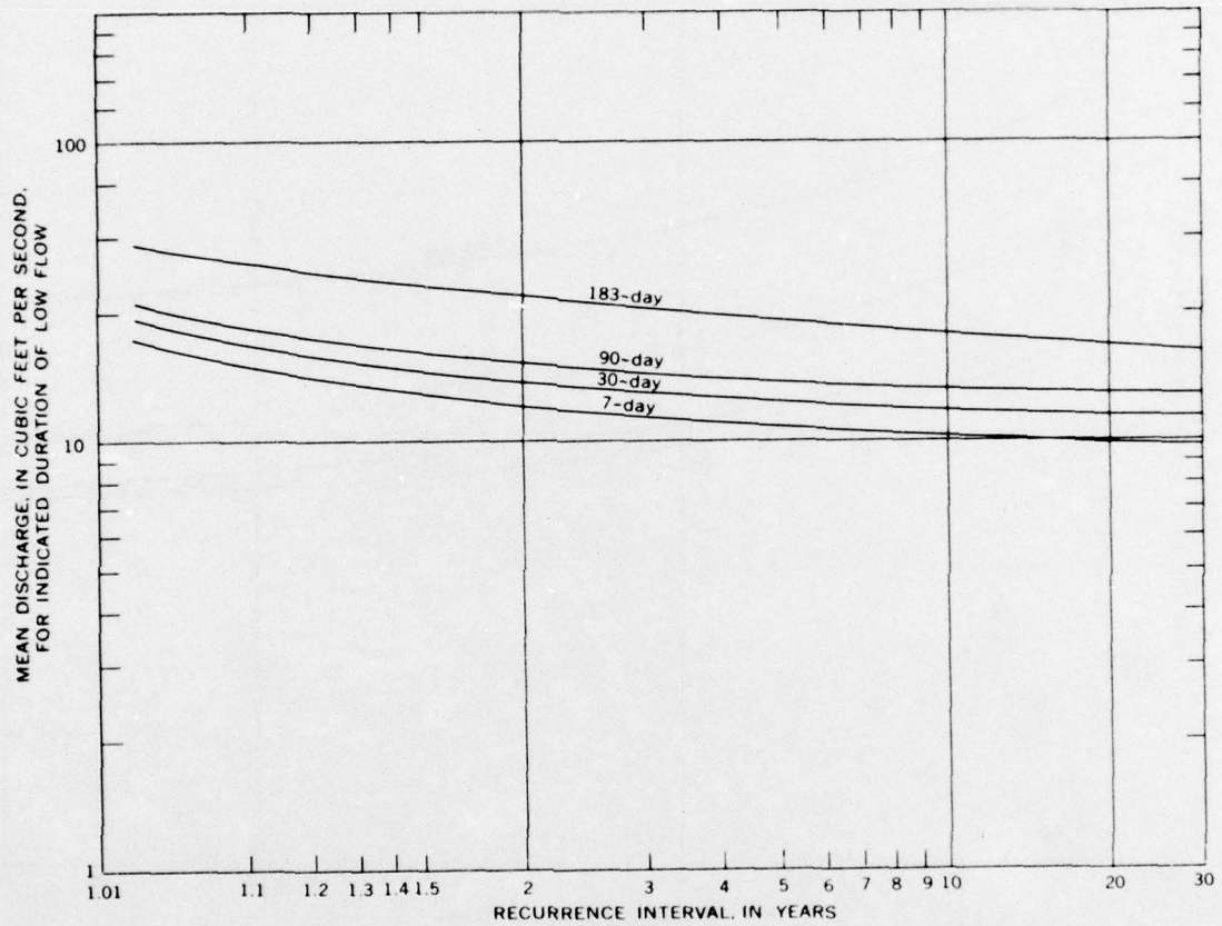
FIGURE 112.—Low-flow frequency, Dewatto River near Dewatto, 1946-63.
