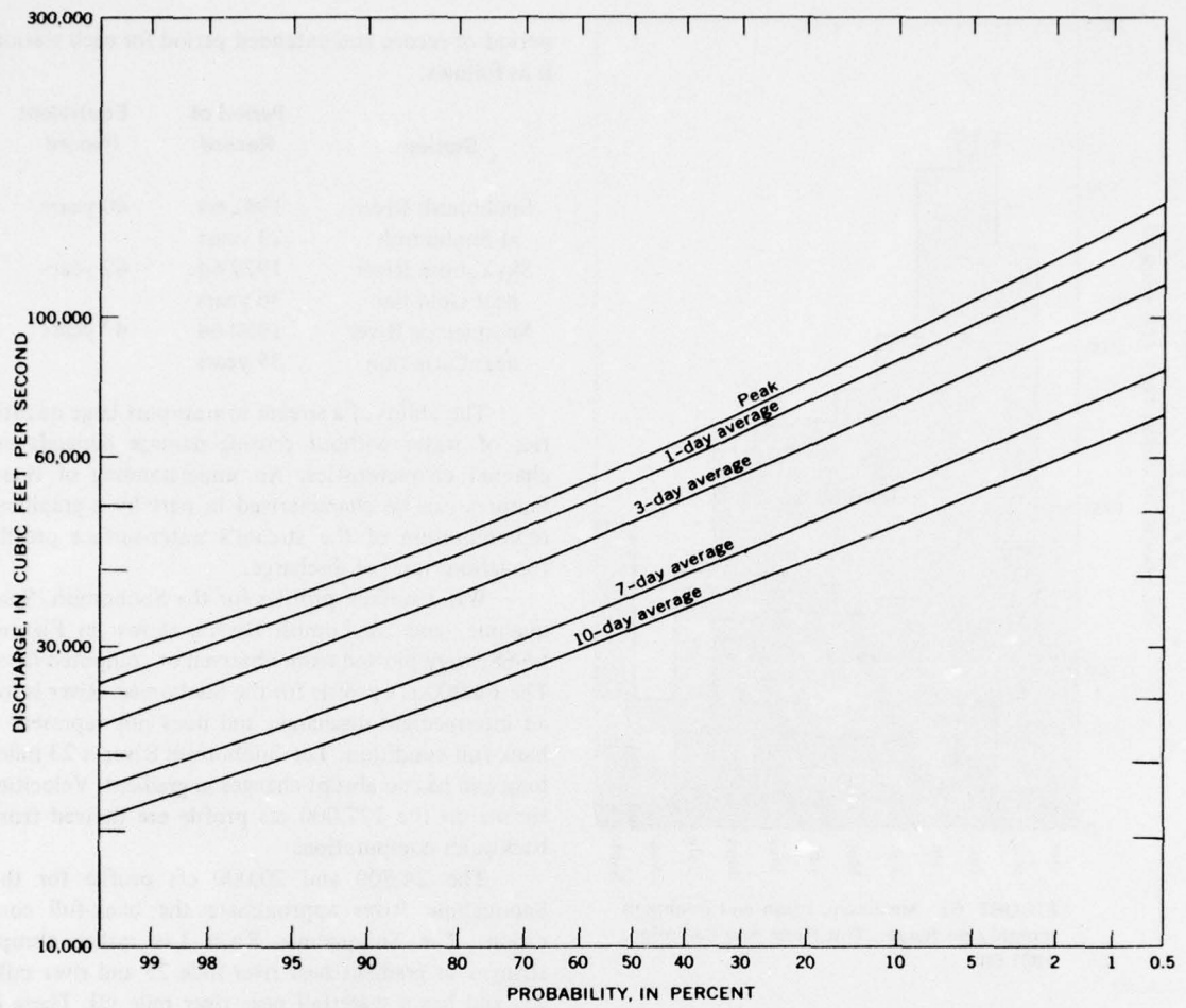
FIGURE 63.—Probability curves of annual maximum flows for specified time periods, Snohomish River at Snohomish.
