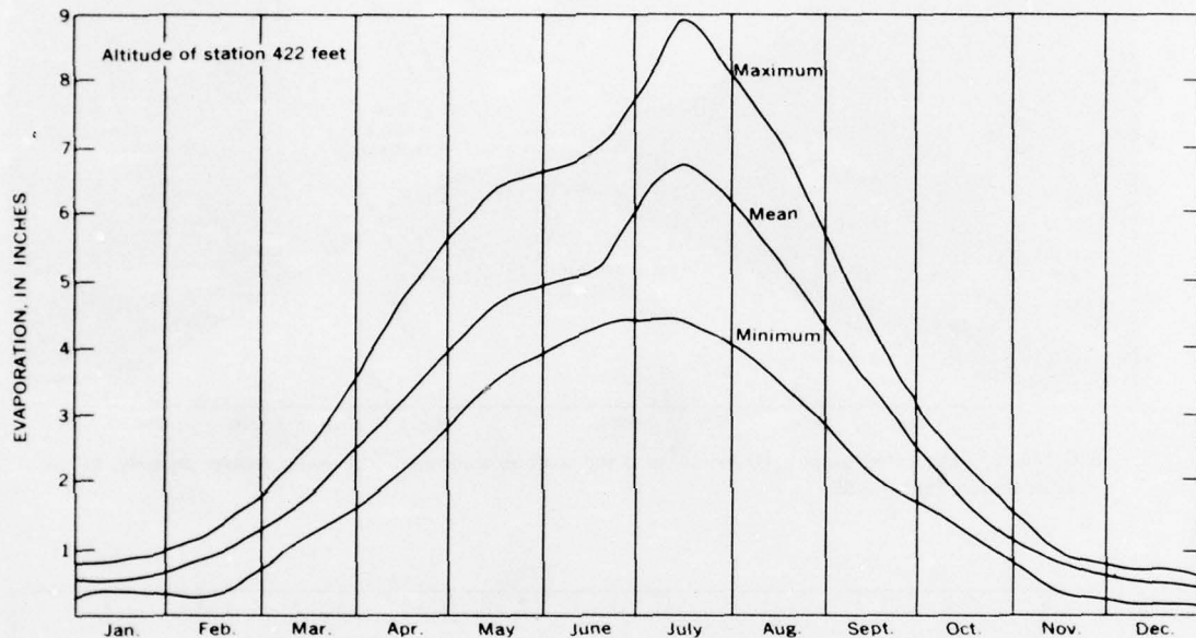
FIGURE 16.—Monthly class-A pan evaporation, in inches, at Seattle Maple Leaf Reservoir, 1941-60.
