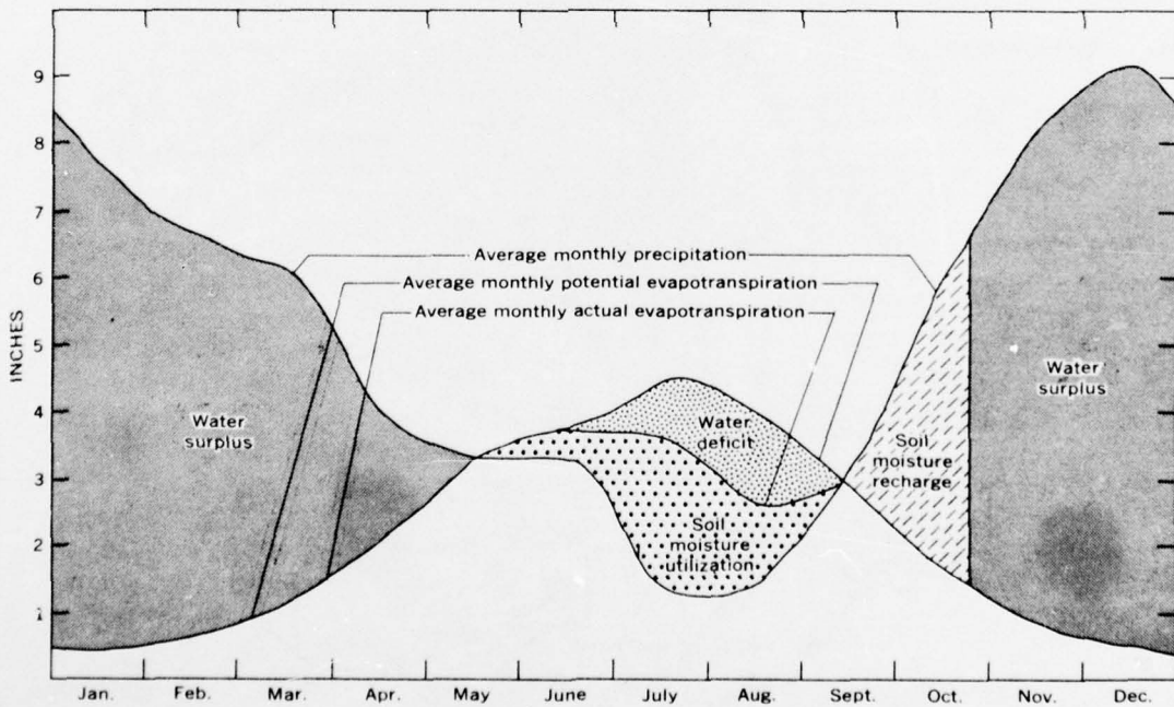
FIGURE 20.—Estimated evapotranspiration of a soil with an assumed 6-inch water-storage capacity, at Snoqualmie Falls.
