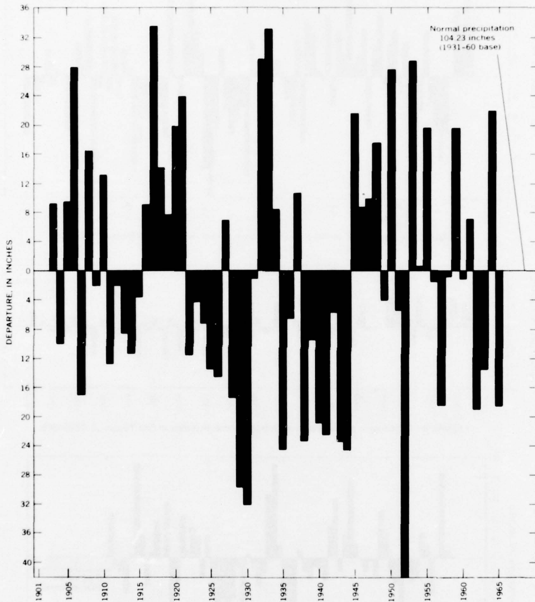
FIGURE 6.—Departure of annual precipitation from normal, in inches, at Cedar Lake, 1903-65.
