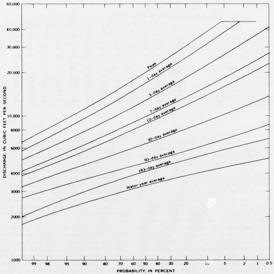
FIGURE 90.—Probability curves of annual maximum flows for specified time periods, Puyallup River at Puyallup.
