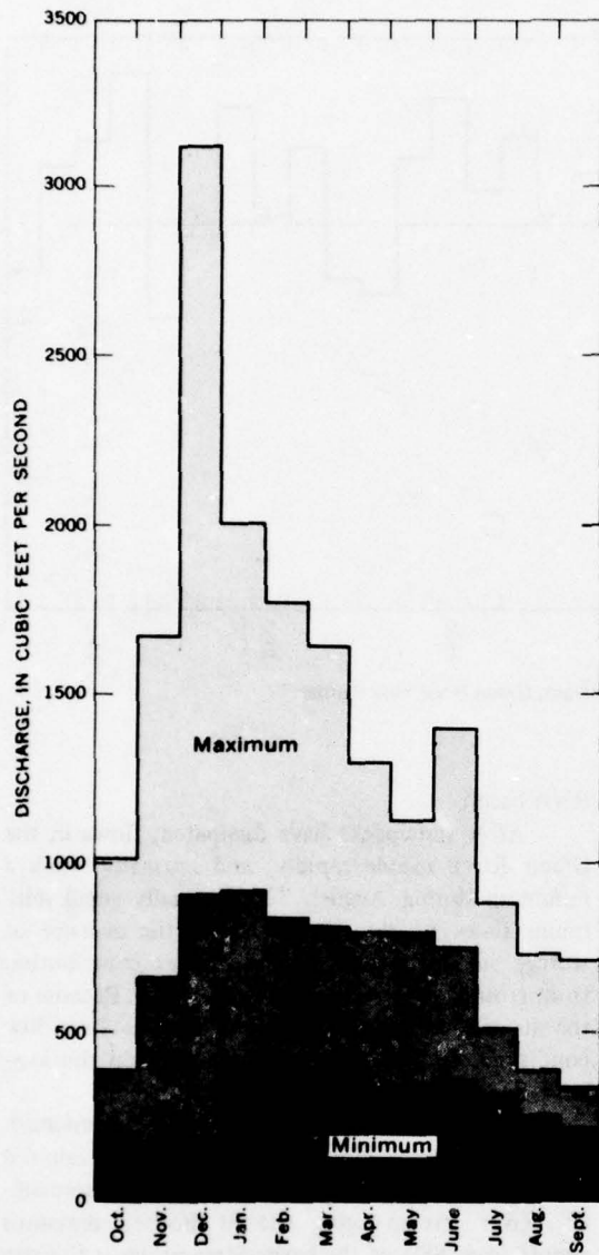
FIGURE 75.—Maximum, mean and minimum monthly discharges, Cedar River near Landsburg, 1931-60.
