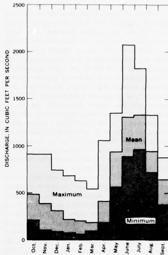
FIGURE 36.—Maximum, mean and minimum monthly discharges, Thunder Creek near Newhalem, 1931-60.
