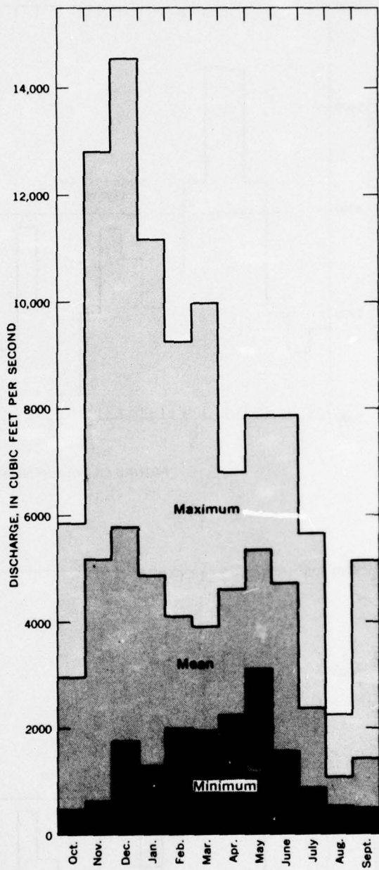
FIGURE 59.—Maximum, mean and minimum monthly discharges, Snoqualmie River near Carnation, 1931-60.
