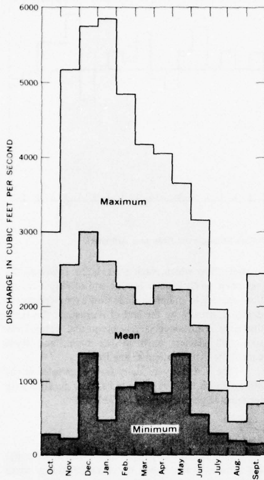
FIGURE 47.—Maximum, mean and minimum monthly discharges, North Fork Stillaguamish River near Arlington, 1931-60.
