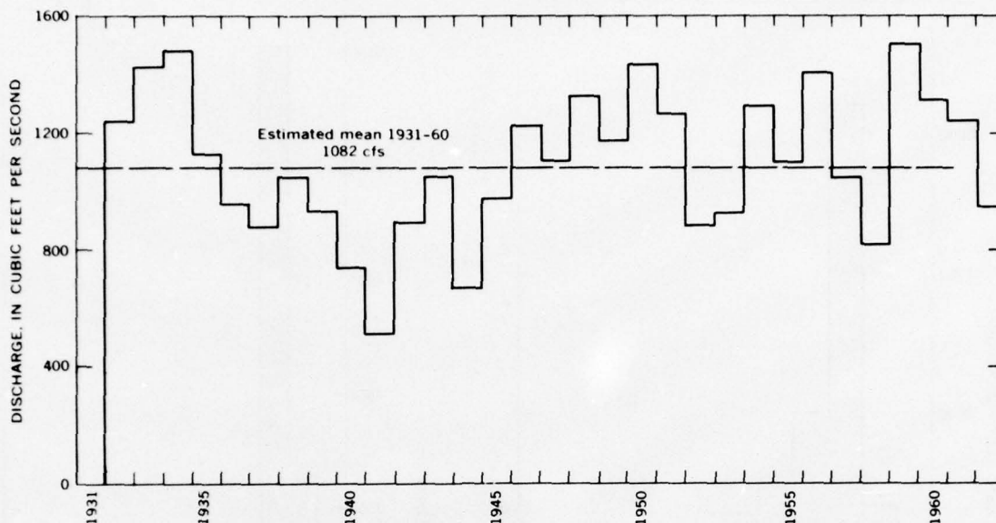
FIGURE 74.—Annual discharges, Green River near Palmer.
