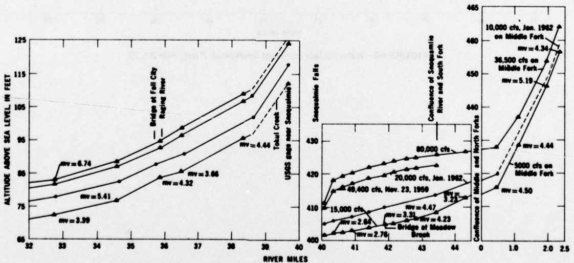
FIGURE 67.—Water-surface profiles of Snoqualmie River, mile 0-43.
