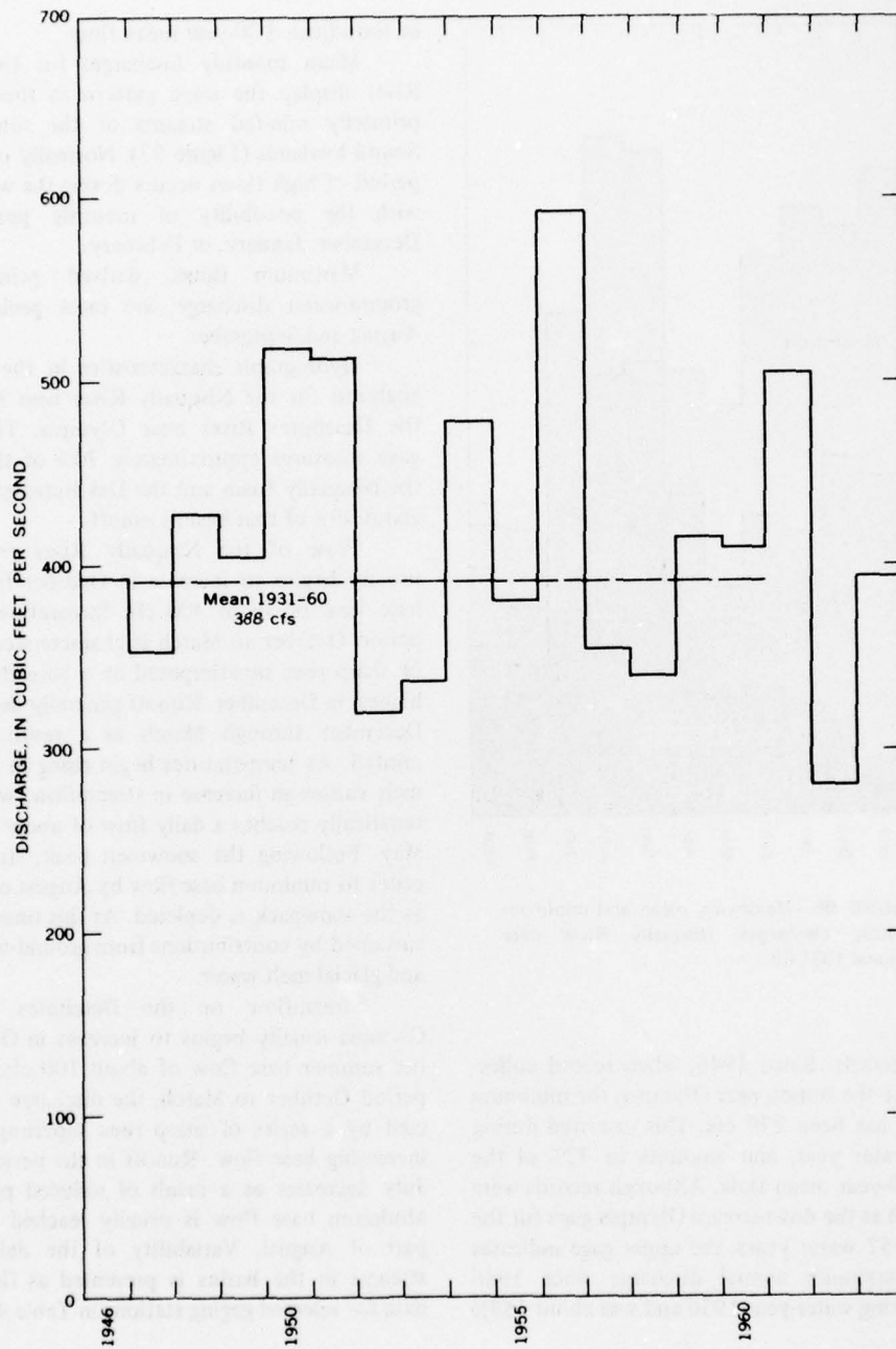
FIGURE 96.—Annual discharges, Deschutes River near Olympia.
