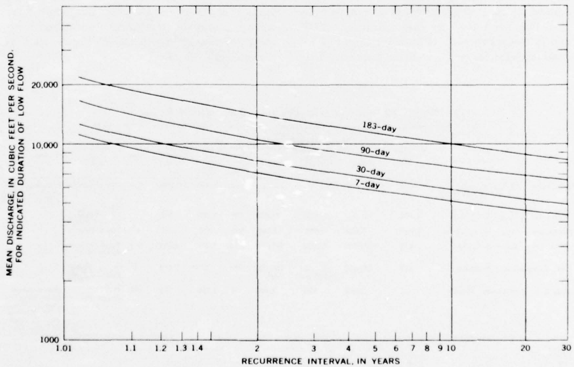
FIGURE 44.—Low-flow frequency, Skagit River near Mount Vernon, 1946-63.
