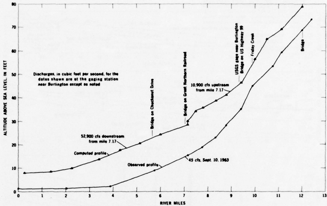
FIGURE 41.—Water-surface profile of Samish River, mile 0-12.
