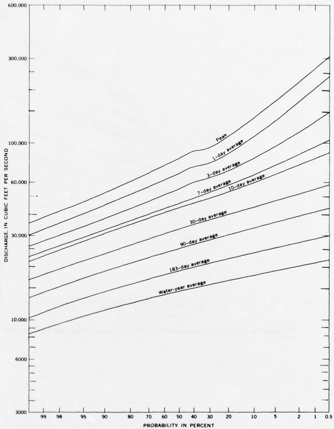
FIGURE 38.—Probability curves of annual maximum flows for specified time periods, Skagit River near Concrete.
