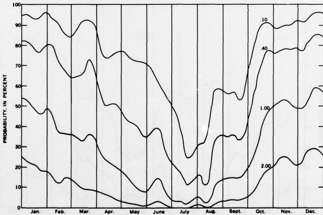
FIGURE 11.—Probability of various amounts of precipitation (inches) in 7 days at Puyallup Experiment station (based on 1931-60 data).
