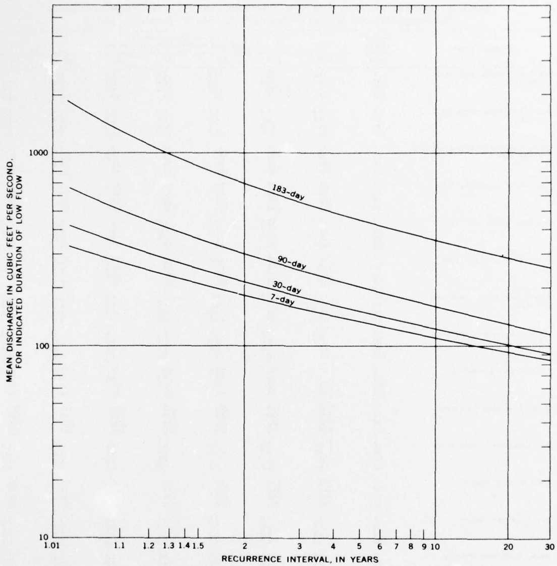
FIGURE 83.—Low-flow frequency, Green River near Auburn, 1946-63.
