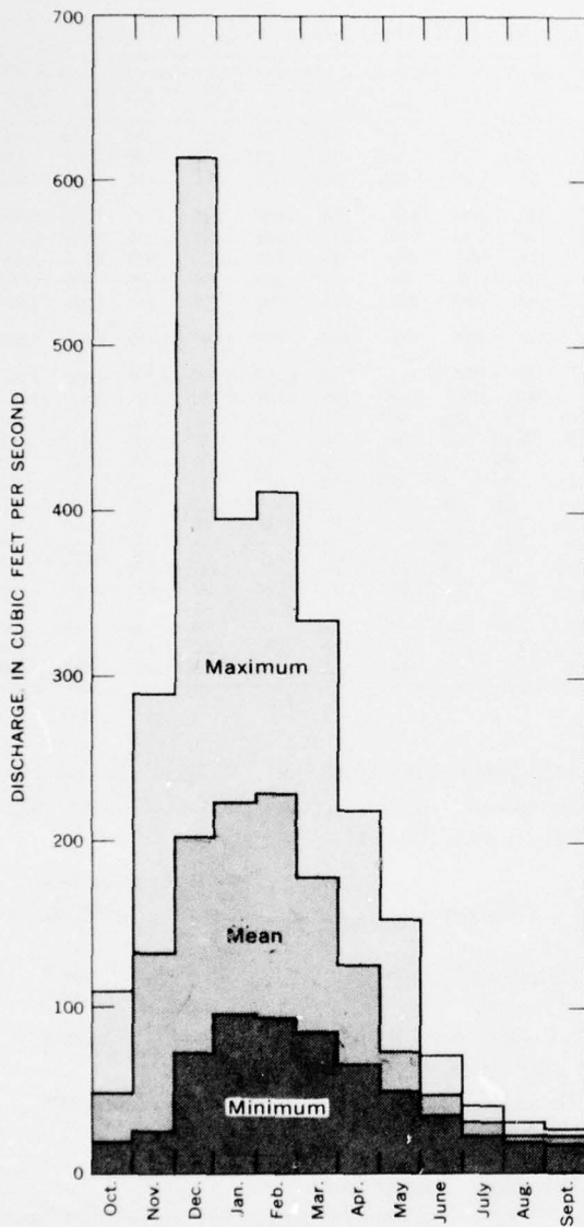
FIGURE 107.—Maximum, mean and minimum monthly discharges, Goldsborough Creek near Shelton, 1931-60.
