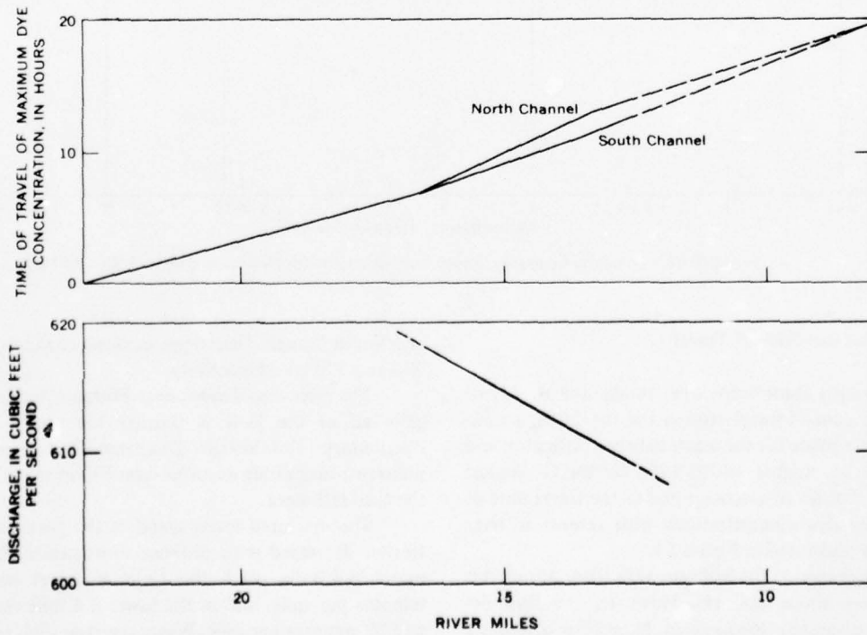
FIGURE 54.—Water discharge and time of travel of dye, Stillaguamish River, August 24-25, 1966.
