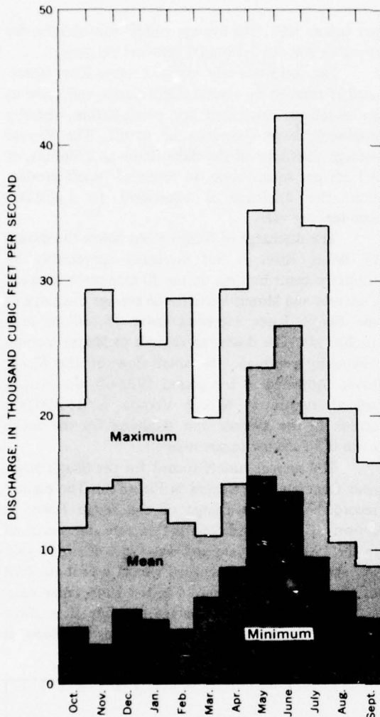
FIGURE 35.—Maximum, mean and minimum monthly discharges, Skagit River near Concrete, 1931-60.
