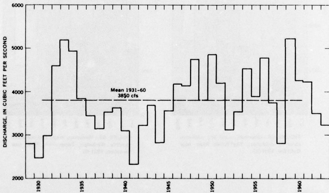
FIGURE 57.—Annual discharges, Snoqualmie River near Carnation.
