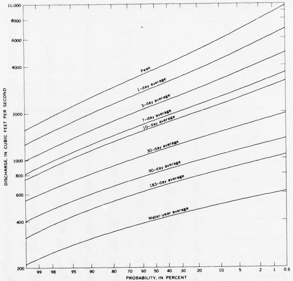
FIGURE 99.—Probability curves of annual maximum flows for specified time periods, Deschutes River near Olympia.
