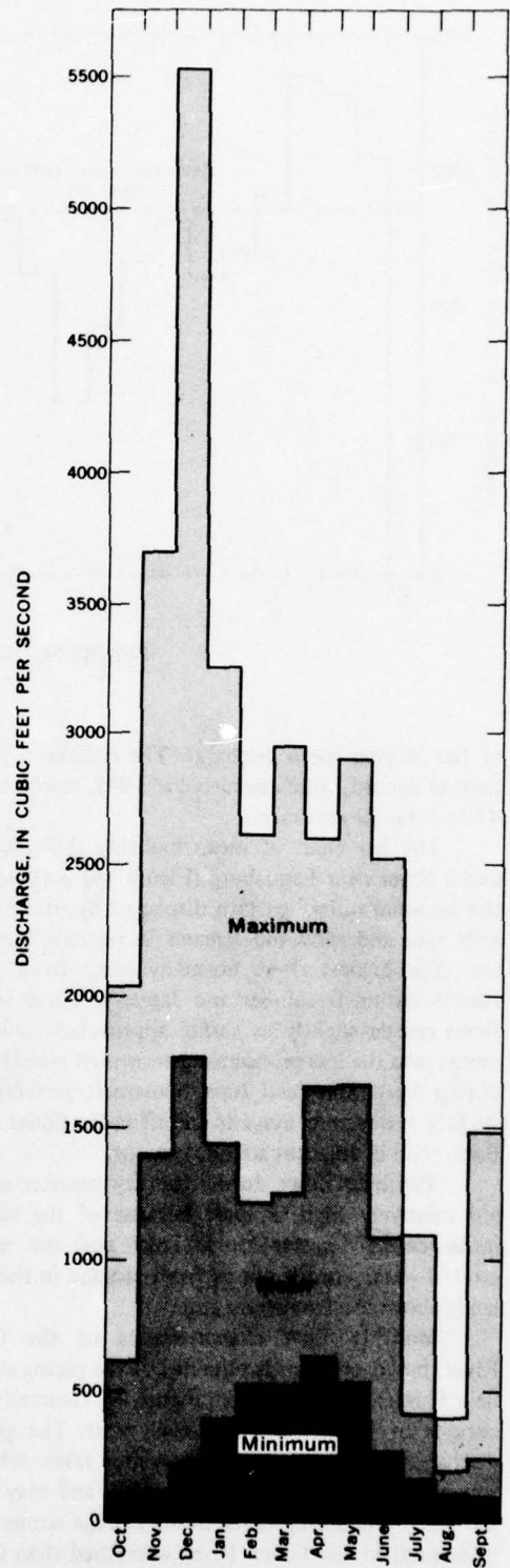
FIGURE 76.—Maximum, mean and minimum monthly discharges, Green River near Palmer, 1931-60.
