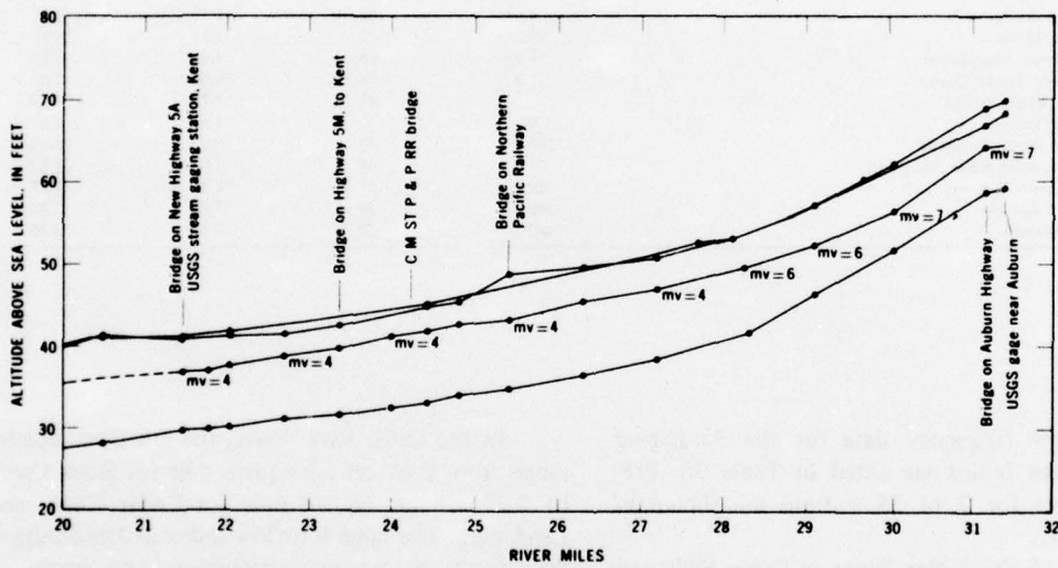
FIGURE 80.—Water-surface profile of Green-Duwamish River, mile 6.55-32.
