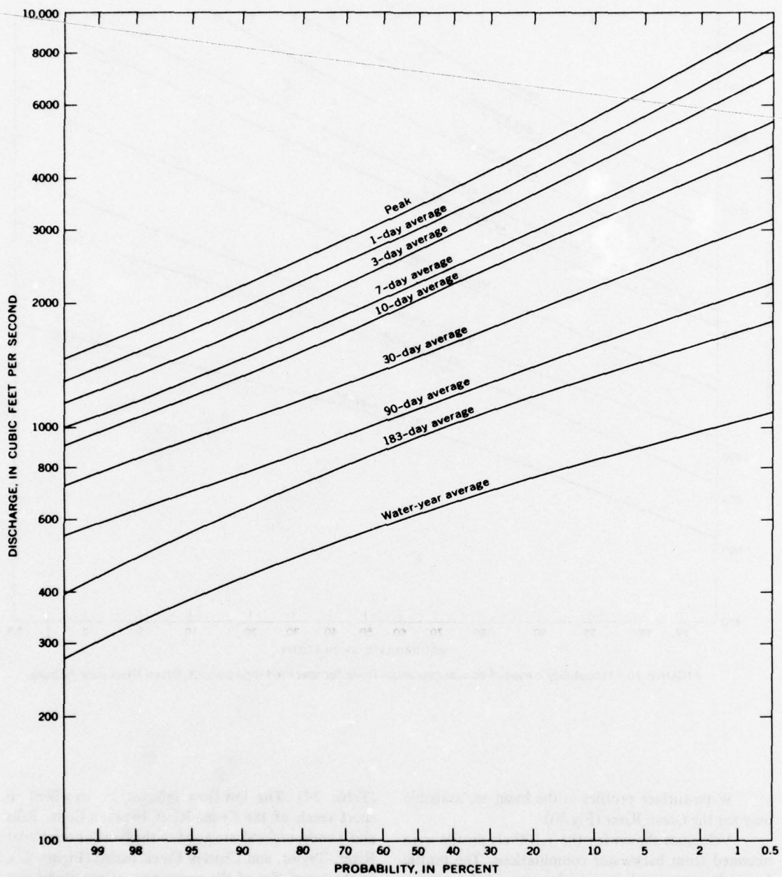
FIGURE 78.—Probability curves of annual maximum flows for specified time periods, Cedar River at Renton.
