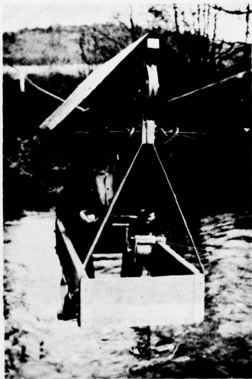
STREAM GAUGING STATION. Stream discharges are measured by a current meter suspended from a cable car. Automatic recording water level gauge on shore is calibrated to measured discharges.
