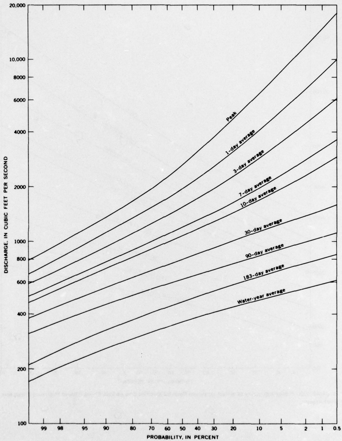
FIGURE 119.—Probability curves of annual maximum flows for specified time periods, Dungeness River near Sequim.
