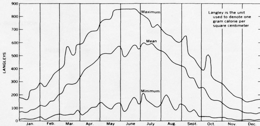
FIGURE 14.—Average daily solar radiation and extremes, in langleys, by weekly periods at Seattle-Tacoma Airport, 1950-59.
