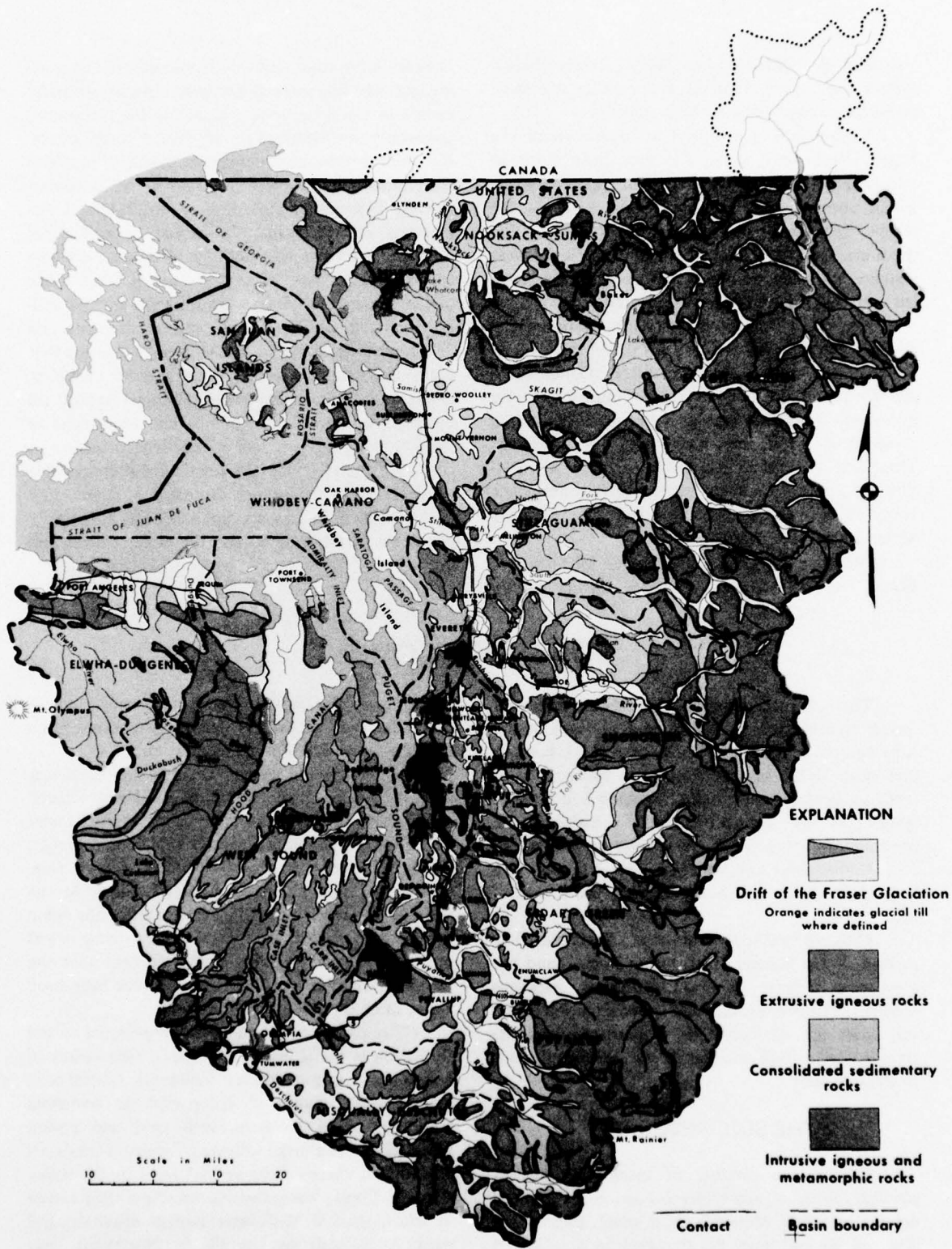
FIGURE 2. Generalized geologic map of the Puget Sound Study Area
