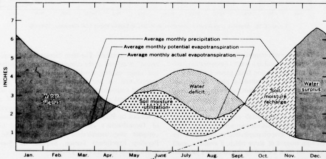
FIGURE 18.—Estimated evapotranspiration of a soil with an assumed 6-inch water storage capacity, at the Puyallup Experiment Station.
