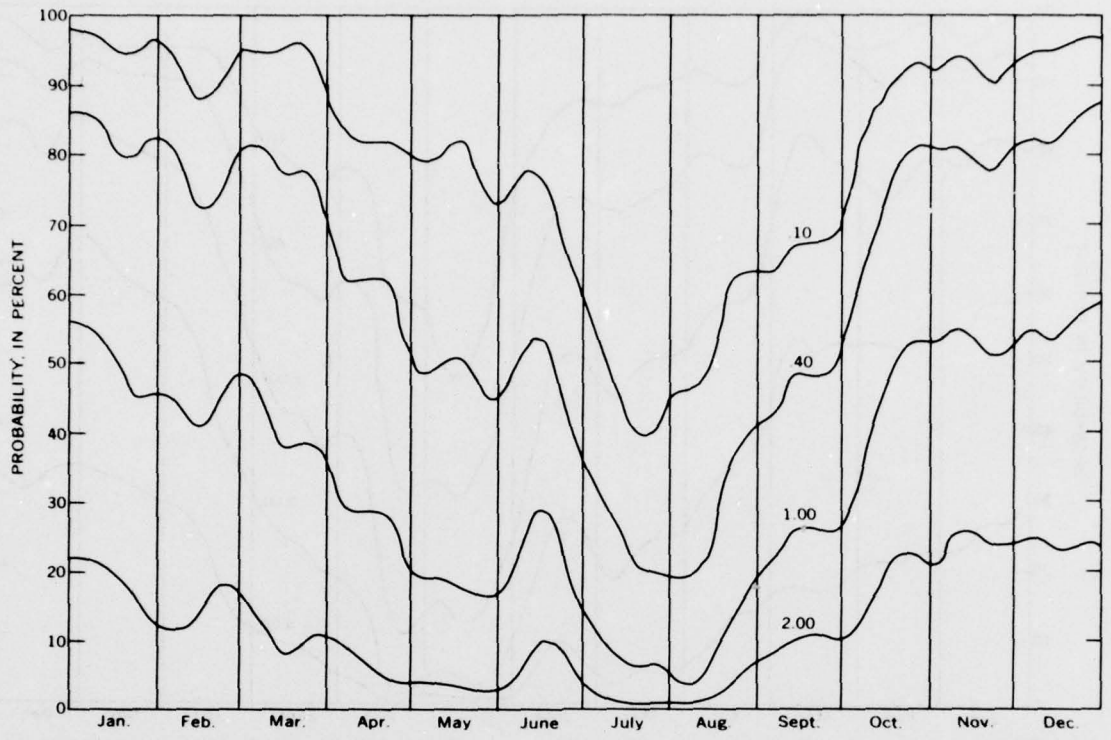
FIGURE 12.—Probability of various amounts of precipitation (inches) in 7 days at Sedro Woolley (based on 1931-60 data).
