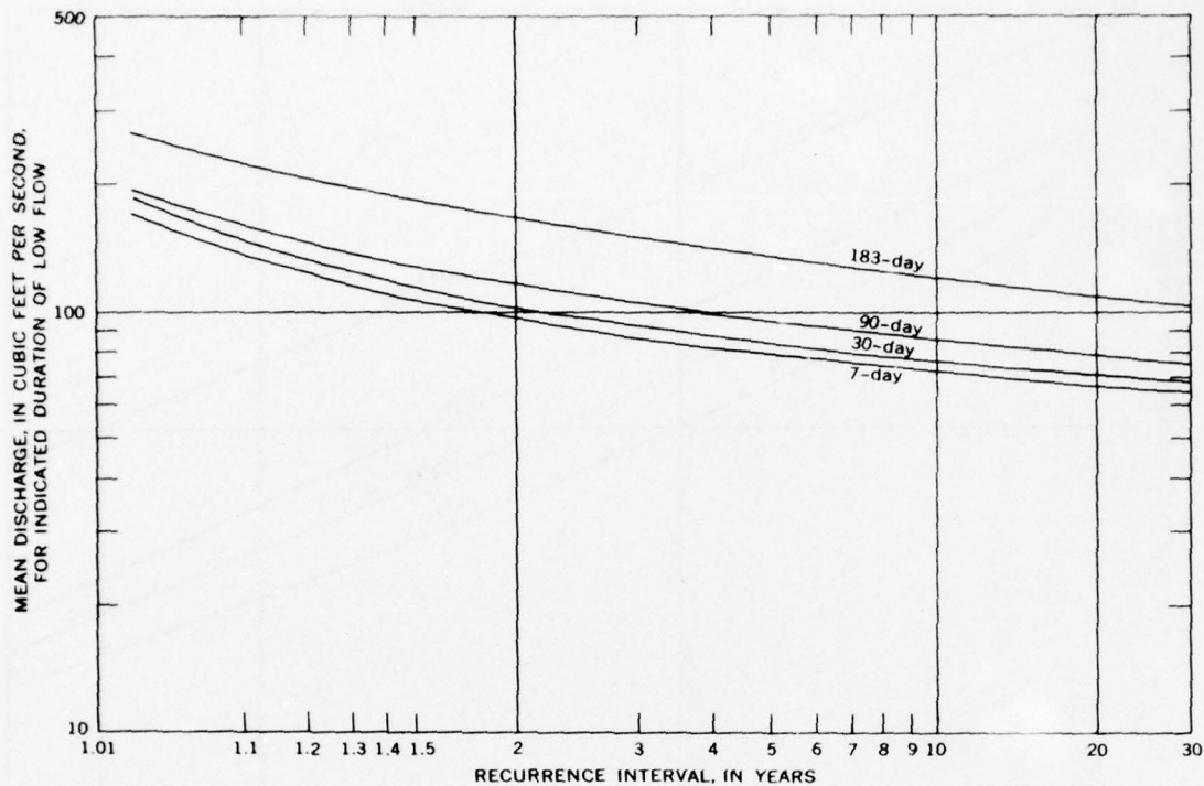
FIGURE 82.—Low-flow frequency, Sammamish River at Bothell, 1946-63.
