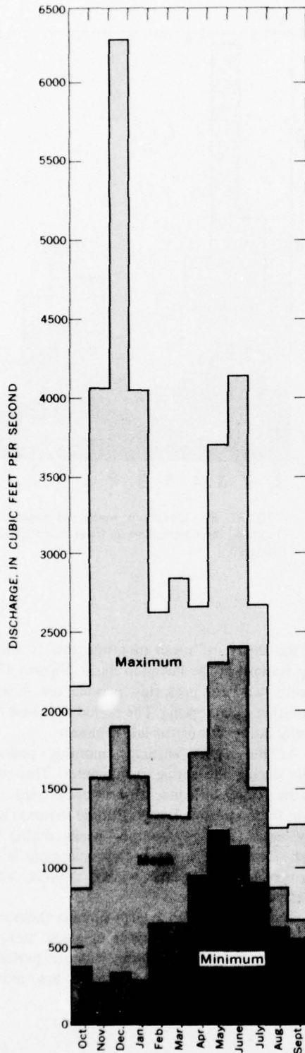
FIGURE 89.—Maximum, mean and minimum monthly discharges, White River near Buckley, 1931-60.
