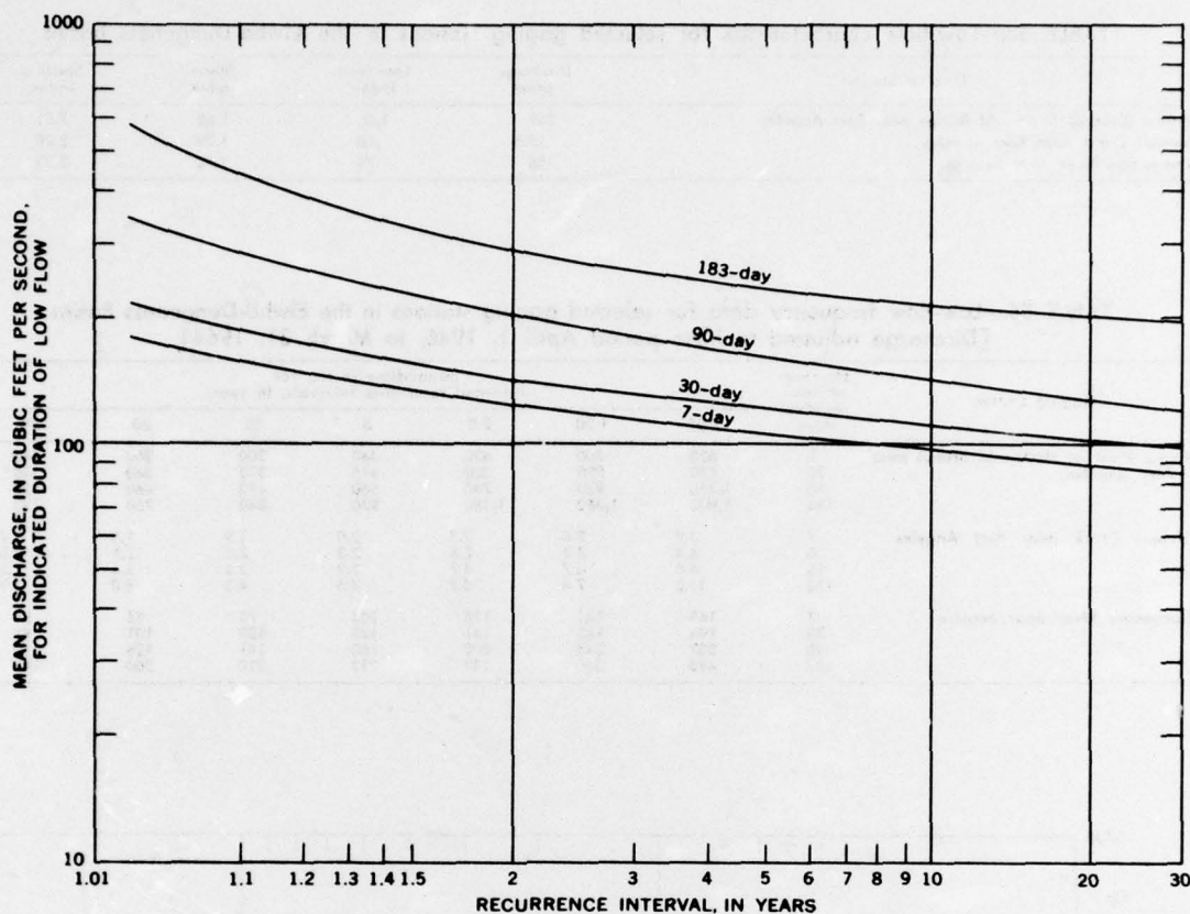
FIGURE 122.—Low-flow frequency, Dungeness River near Sequim, 1946-63.
