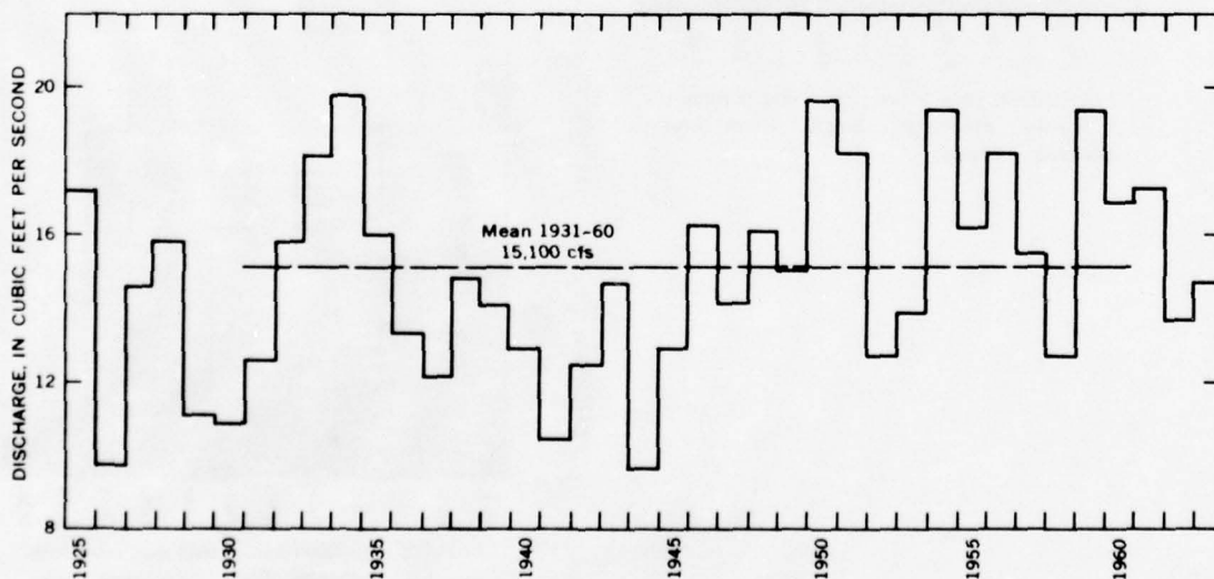
FIGURE 34.—Annual discharges, Skagit River, near Concrete.
