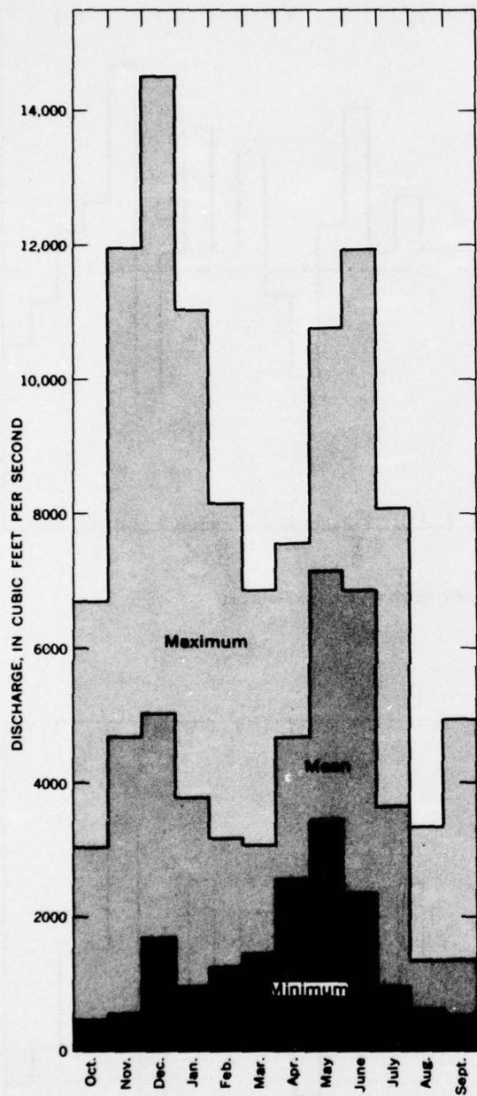
FIGURE 58.—Maximum, mean and minimum monthly discharges, Skykomish River near Gold Bar, 1931-60.
