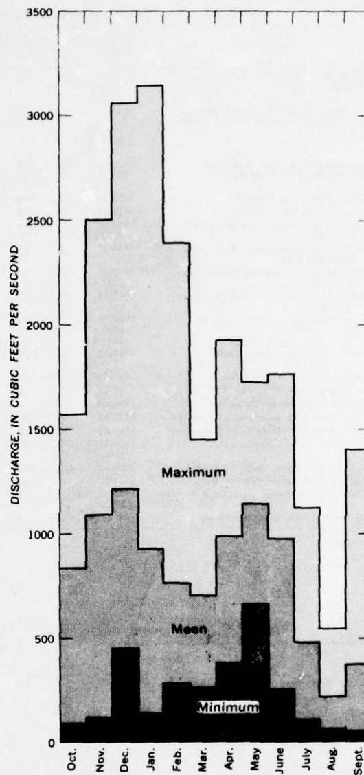
FIGURE 61.—Maximum, mean and minimum monthly discharges, Sultan River near Startup, 1931-60.
