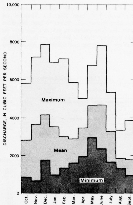
FIGURE 27.—Maximum, mean and minimum monthly discharges, Nooksack River at Deming, 1931-60.
