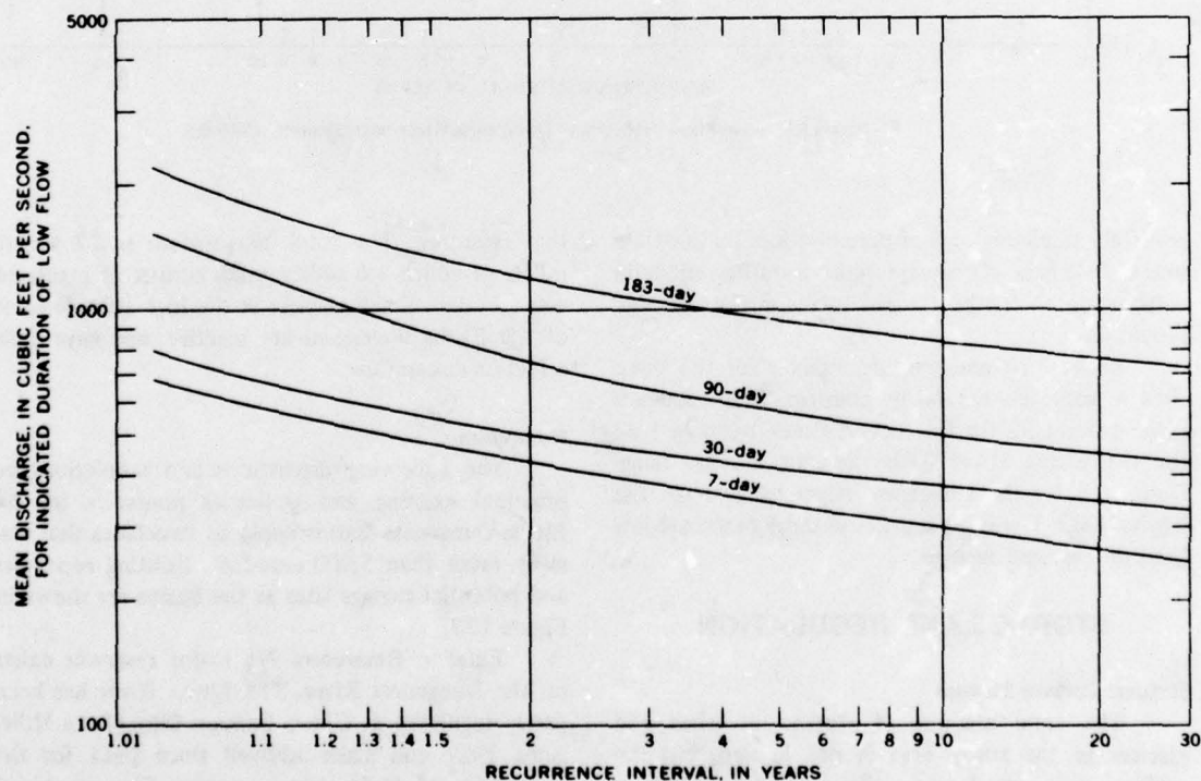
FIGURE 121.—Low-flow frequency, Elwha River at McDonald Bridge near Port Angeles, 1946-63.
