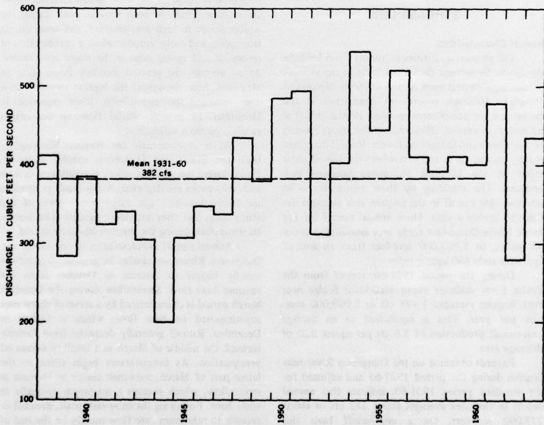
FIGURE 116.—Annual discharges, Dungeness River near Sequim.
