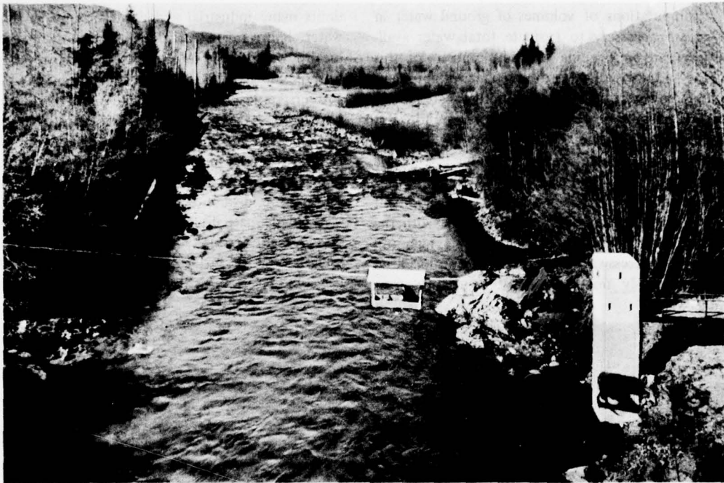
STREAM GAUGING STATION. Stream discharges are measured by a current meter suspended from a cable car. Automatic recording water level gauge on shore is calibrated to measured discharges.
