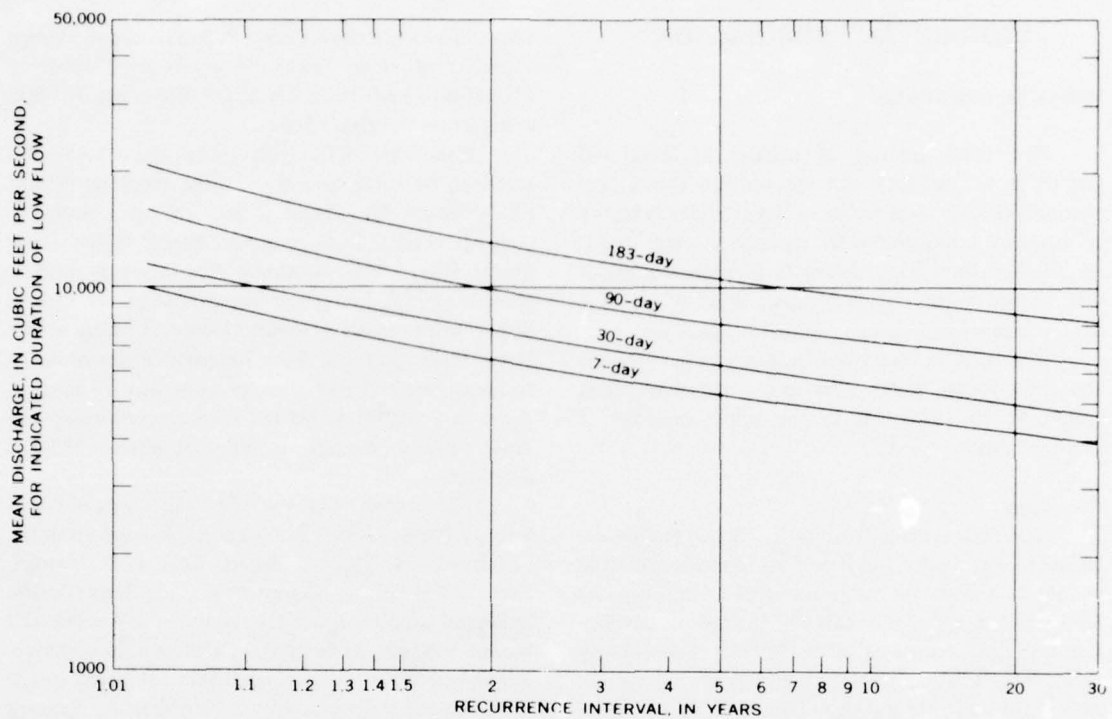
FIGURE 43.—Low-flow frequency, Skagit River near Concrete, 1946-63.
