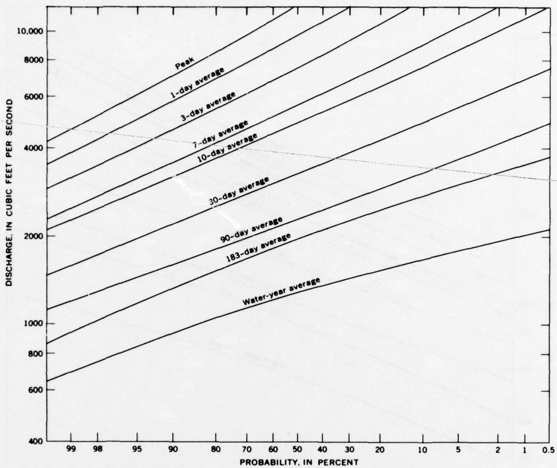
FIGURE 79.—Probability curves of annual maximum flows for specified time periods, Green River near Auburn.
