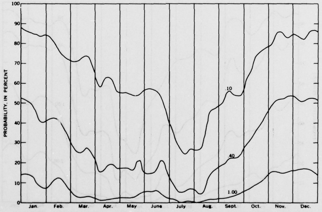
FIGURE 13.—Probability of various amounts of precipitation (inches) in 7 days at Sequim (based on 1931-60 data).
