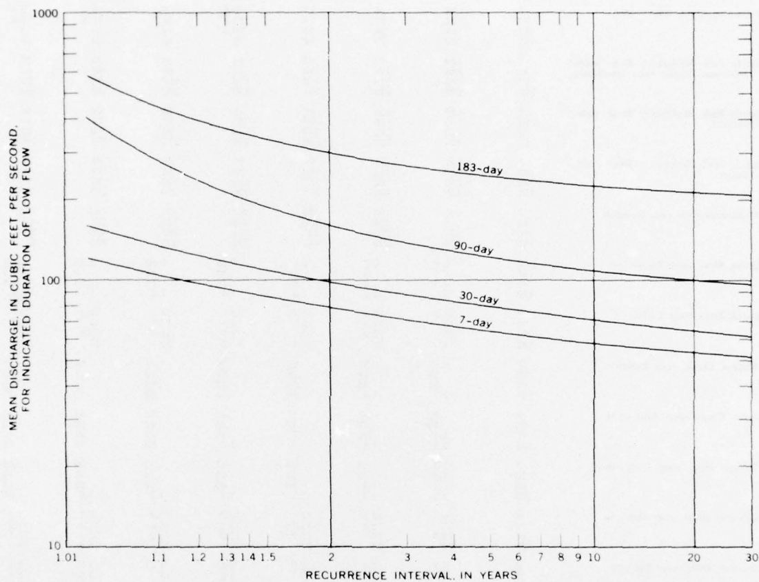
FIGURE 111.—Low-flow frequency, Duckabush River near Brinnon, 1946-63.
