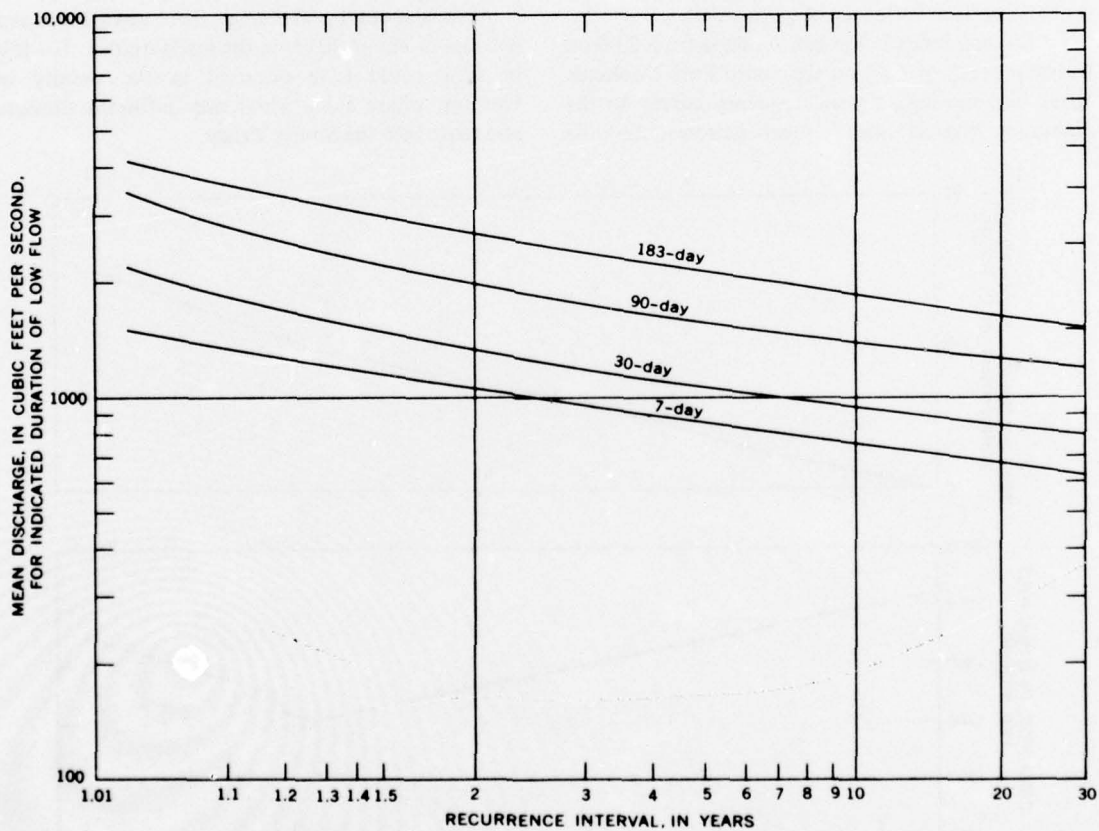
FIGURE 31.—Low-flow frequency, Nooksack River at Deming, 1946-63.
