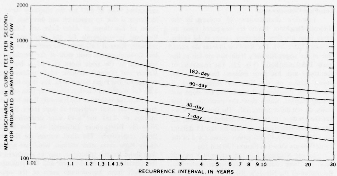
FIGURE 100.—Low-flow frequency, Nisqually River near National, 1946-63.
