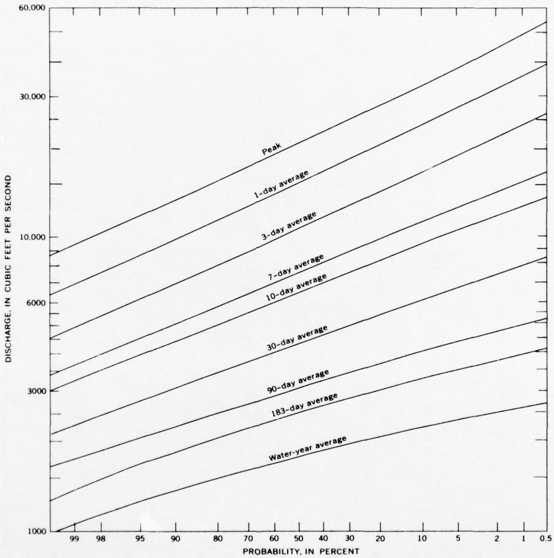
FIGURE 49.—Probability curves of annual maximum flows for specified time periods, North Fork Stillaguamish River near Arlington.
