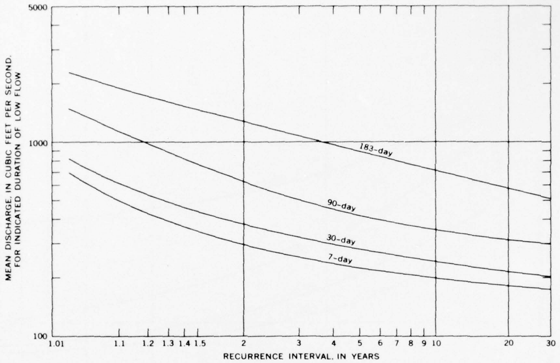
FIGURE 53.—Low-flow frequency, North Fork Stillaguamish River near Arlington, 1946-63.
