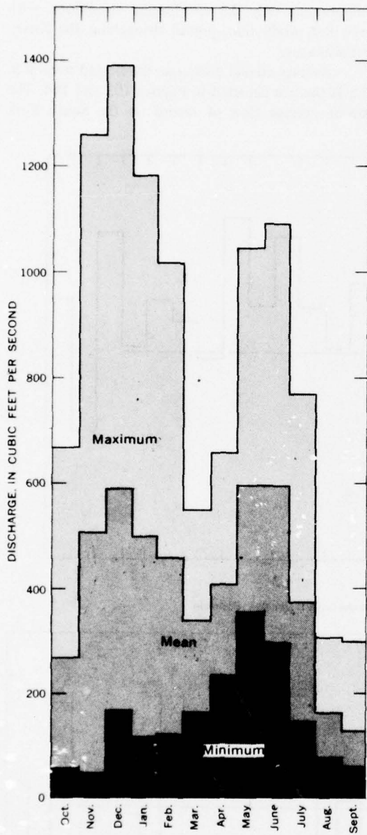
FIGURE 105.—Maximum, mean and minimum monthly discharges, Duckabush River near Brinnon, 1931-60.
