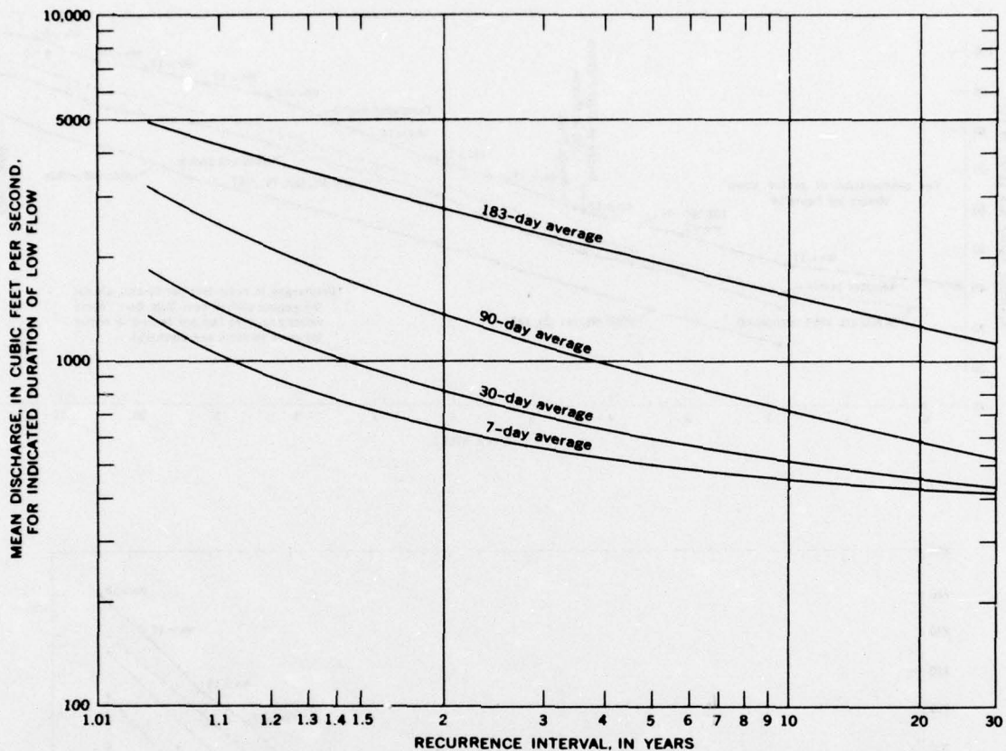
FIGURE 69.—Low-flow frequency, Snoqualmie River near Carnation, 1946-63.
