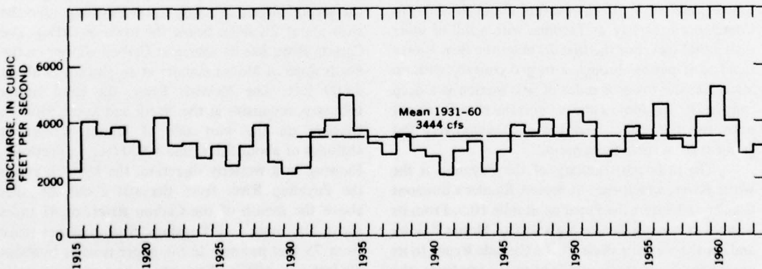
FIGURE 86.—Annual discharges, Puyallup River at Puyallup.
