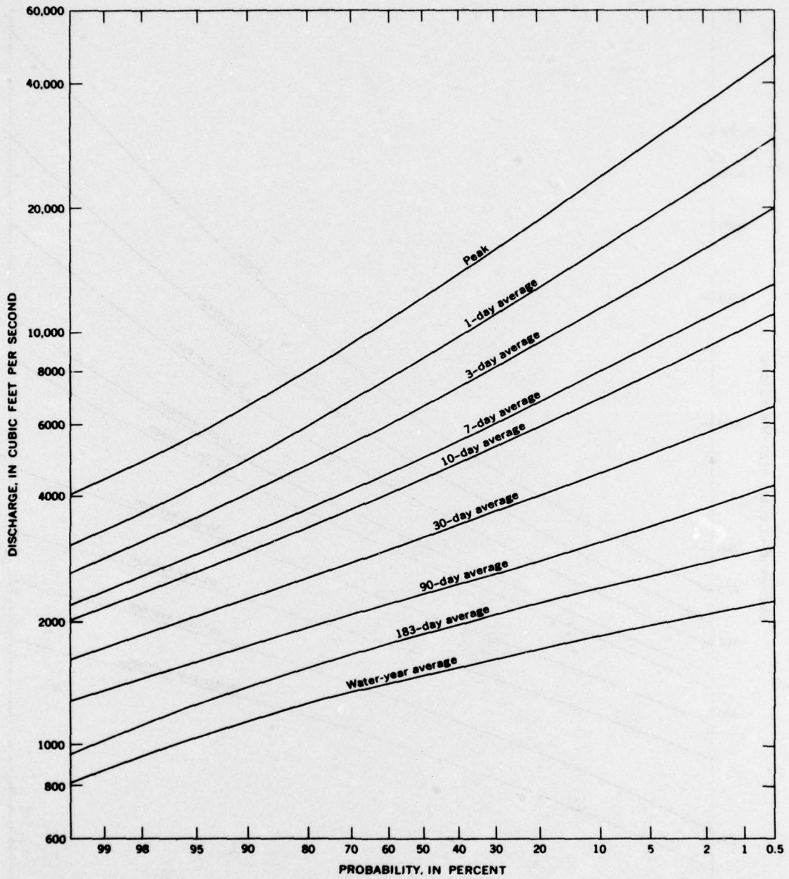
FIGURE 120.—Probability curves of annual maximum flows for specified time periods, Elwha River at McDonald Bridge near Port Angeles.
