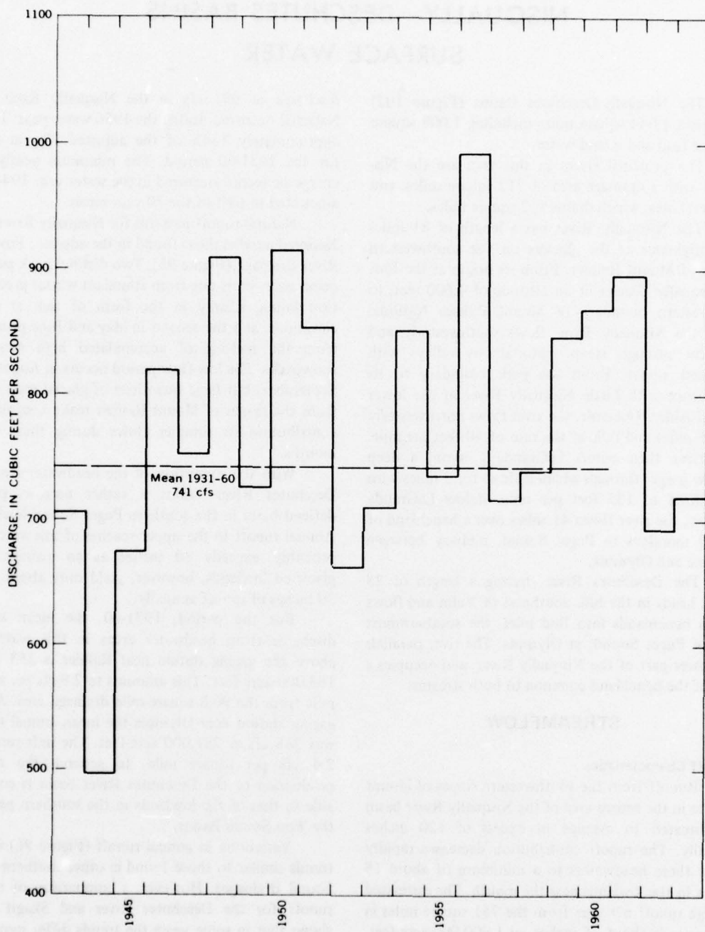
FIGURE 94.—Annual discharges, Nisqually River near National.
