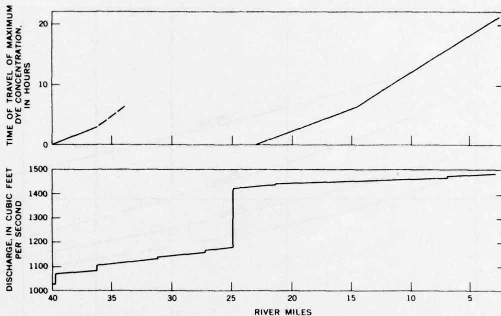
FIGURE 71.—Water discharge and time of travel of dye, Snoqualmie River, August 2-3, 1966.
