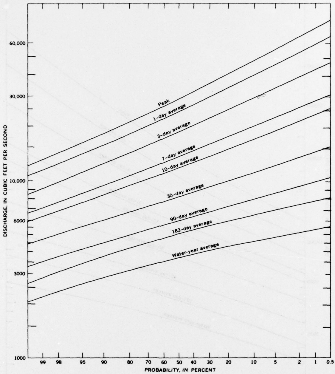
FIGURE 65.—Probability curves of annual maximum flows for specified time periods, Snoqualmie River near Carnation.
