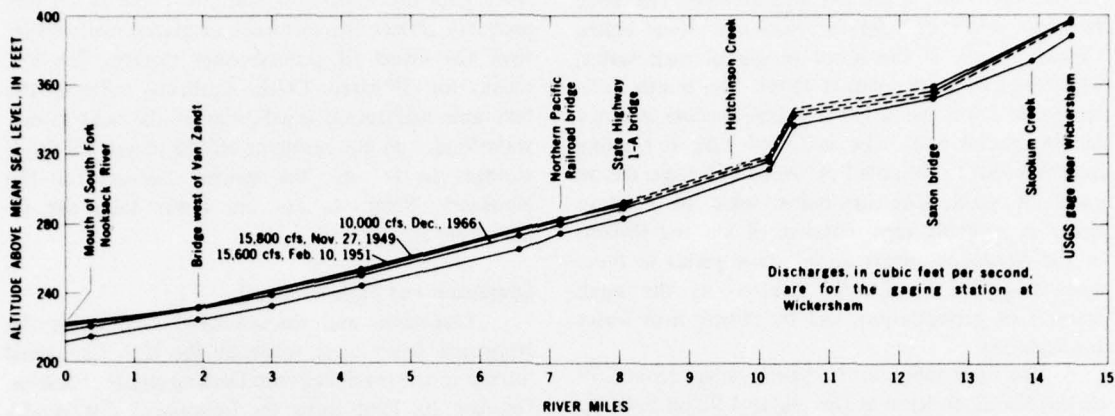
FIGURE 30.—Water-surface profile of South Fork Nooksack River, mile 0-14.
