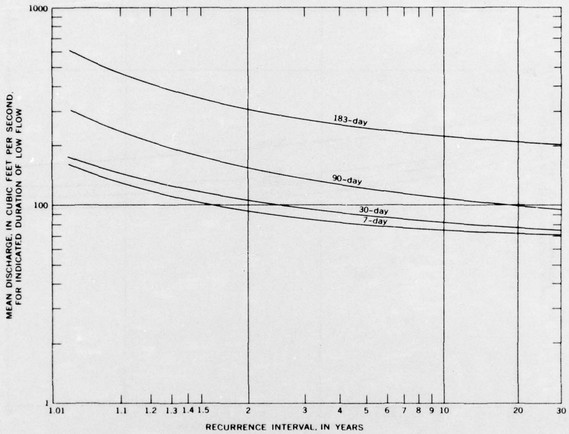
FIGURE 113.—Low-flow frequency, South Fork Skokomish River near Union, 1946-63.
