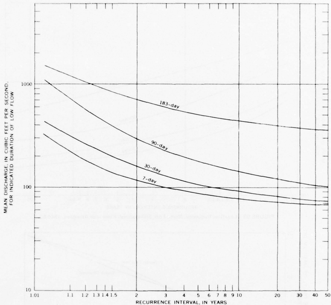
FIGURE 52.—Low-flow frequency, South Fork Stillaguamish River near Granite Falls, 1931-60.
