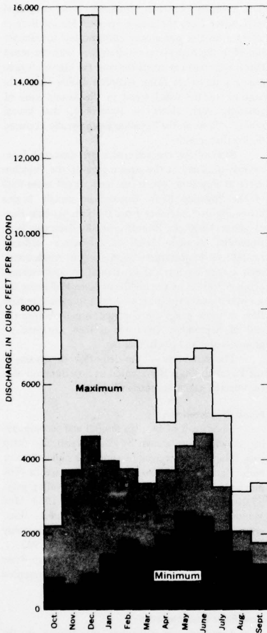
FIGURE 87.—Maximum, mean and minimum monthly discharges, Puyallup River at Puyallup, 1931-60.
