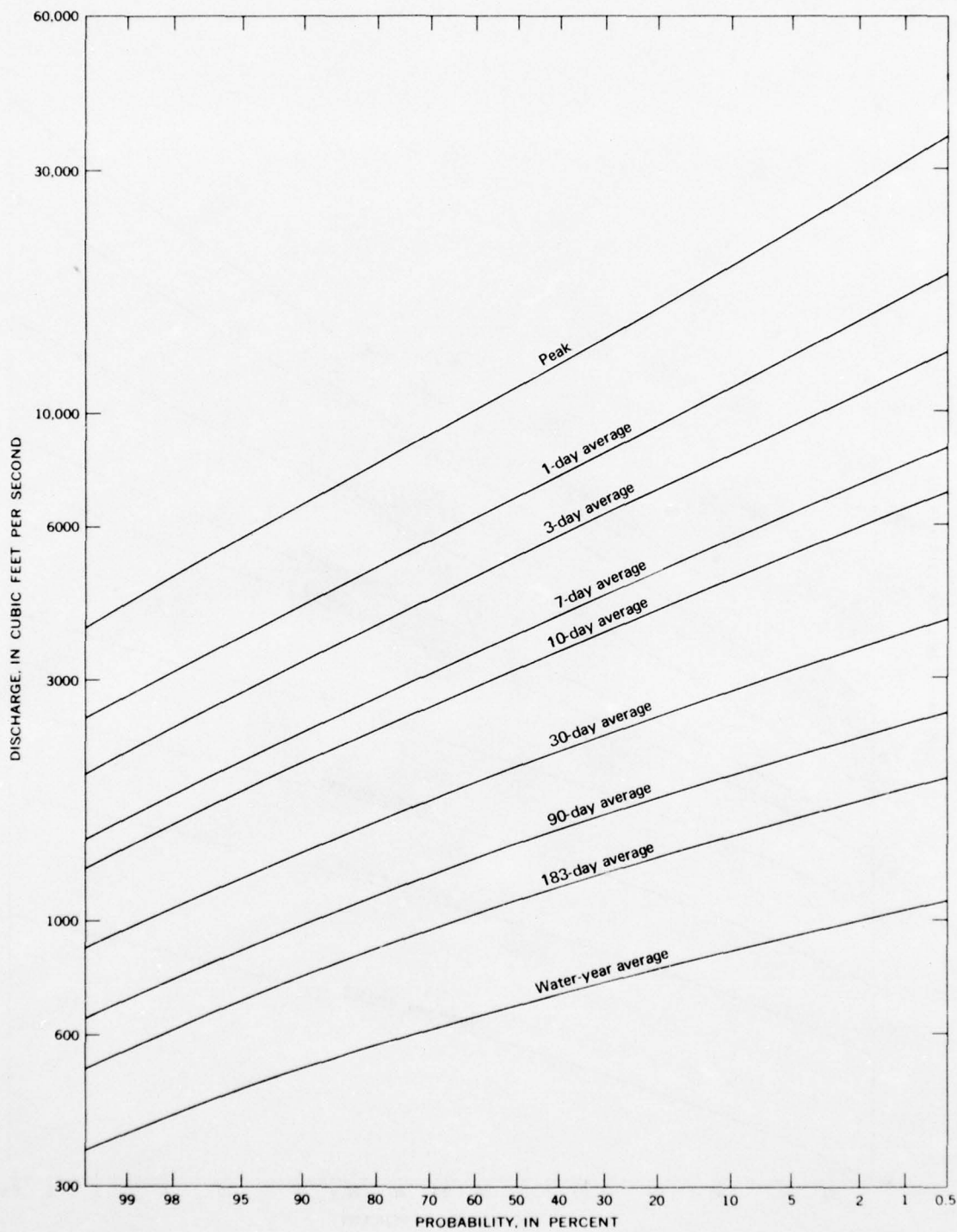
FIGURE 109.—Probability curves of annual maximum flows for specified time periods, South Fork Skokomish River near Union.
