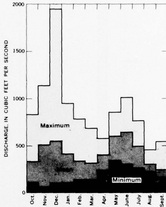
FIGURE 88.—Maximum, mean and minimum monthly discharges, Carbon River near Fairfax, 1931-60.
