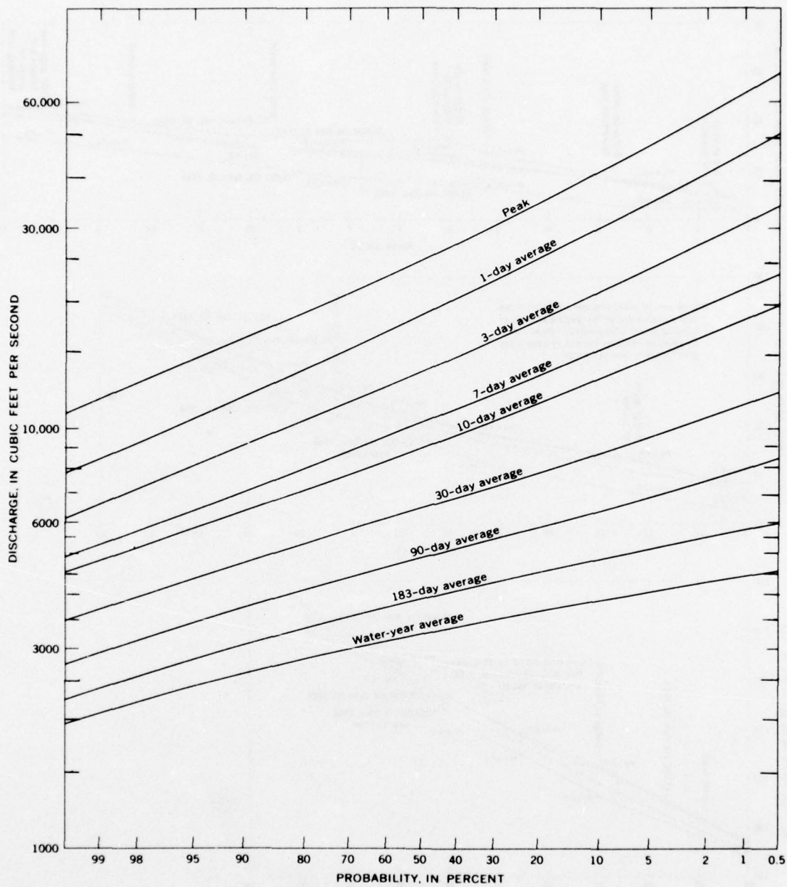
FIGURE 28.—Probability curves of annual maximum flows for specified time periods, Nooksack River at Deming.
