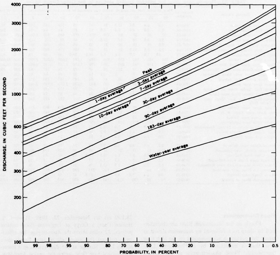
FIGURE 77.—Probability curves of annual maximum flows for specified time periods, Sammamish River at Bothell.
