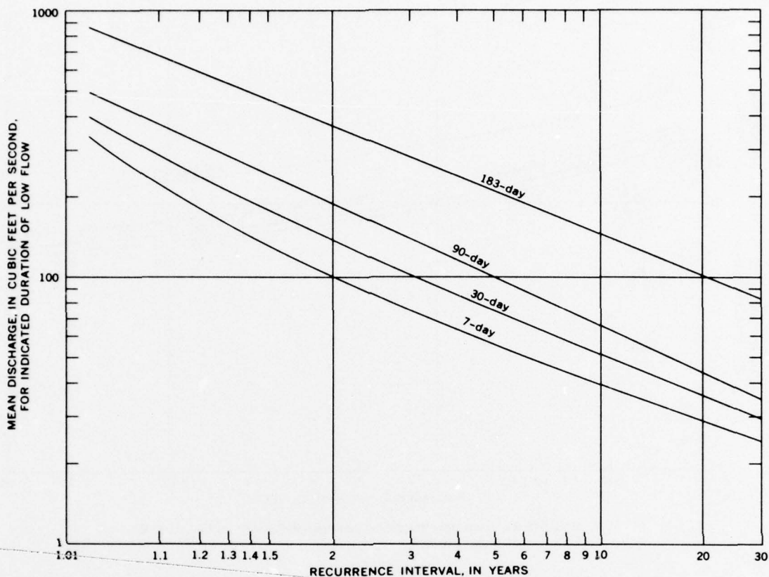
FIGURE 81.—Low-flow frequency, Cedar River at Renton, 1946-63.
