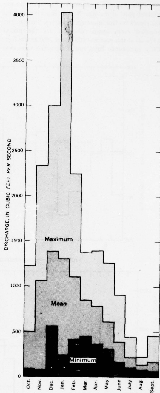
FIGURE 106.—Maximum, mean and minimum monthly discharges, South Fork Skokomish River near Union, 1931-60.
