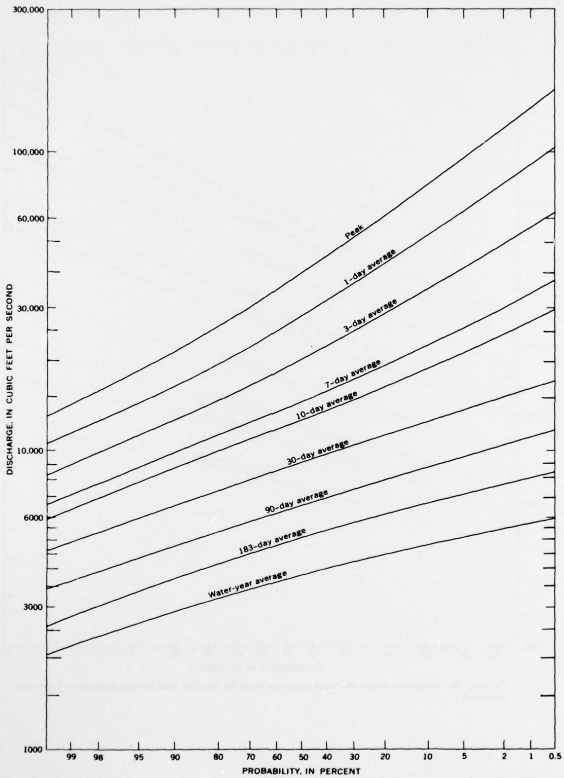
FIGURE 64.—Probability curves of annual maximum flows for specified time periods, Skykomish River near Gold Bar.
