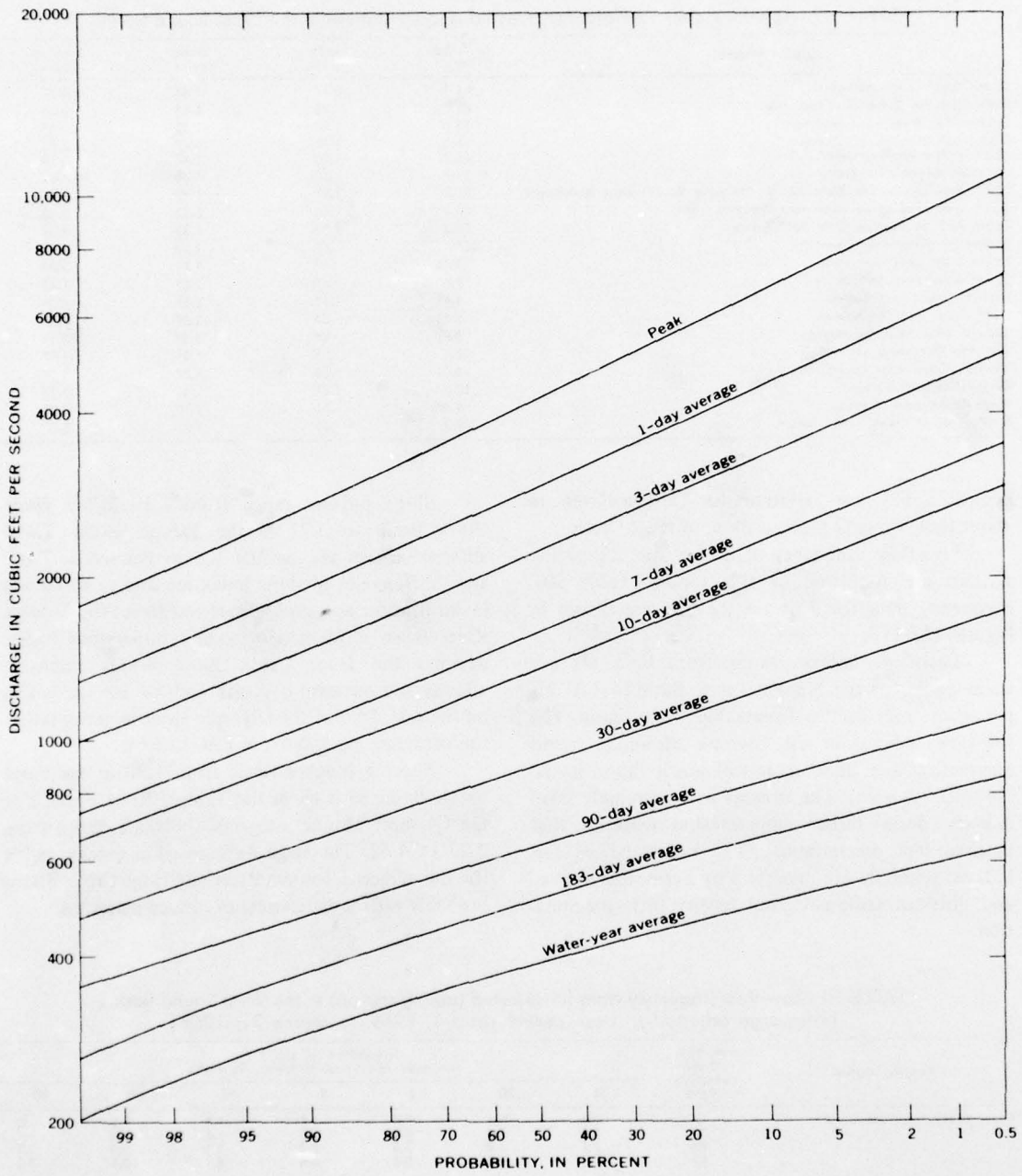
FIGURE 110.—Probability curves of annual maximum flows for specified time periods, Duckabush River near Brannon.
