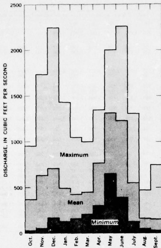
FIGURE 60.—Maximum, mean and minimum monthly discharges, Beckler River near Skykomish, 1931-60.
