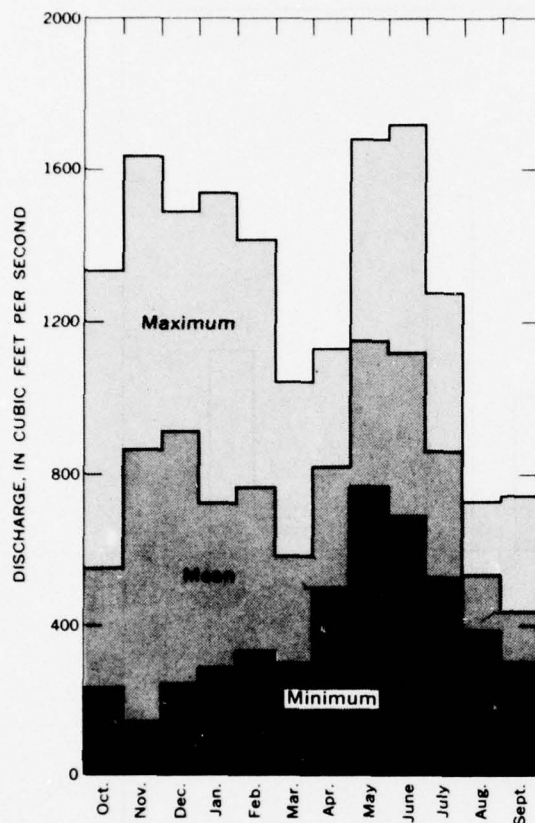
FIGURE 95.—Maximum, mean and minimum monthly discharges, Nisqually River near National 1931-60.
