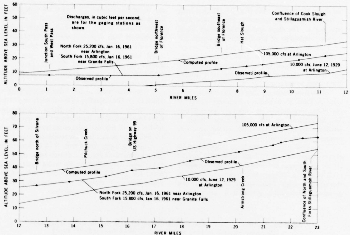
FIGURE 51.—Water-surface profile of Stillaguamish River, mile 0-23.
