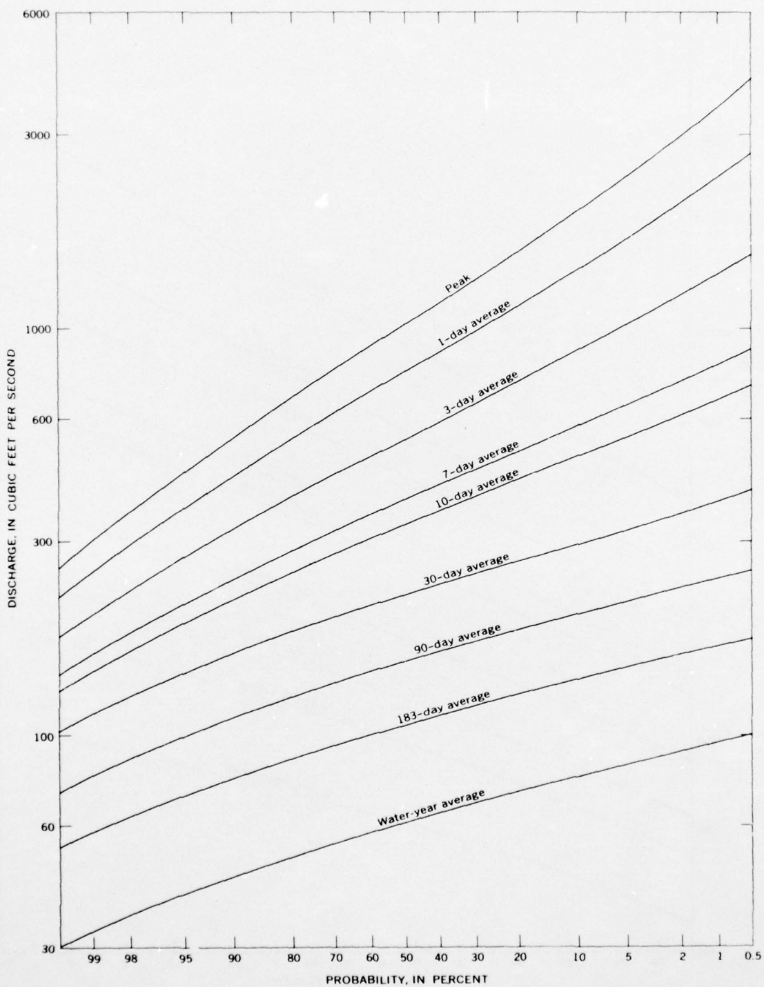
FIGURE 108. Probability curves of annual maximum flows for specified time periods, Dewatto River near Dewatto.
