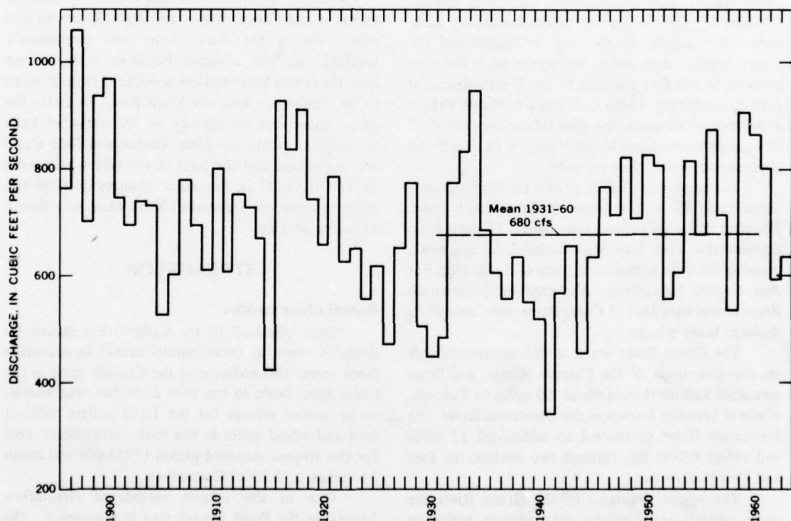
FIGURE 73.—Annual discharges, Cedar River near Landsburg.
