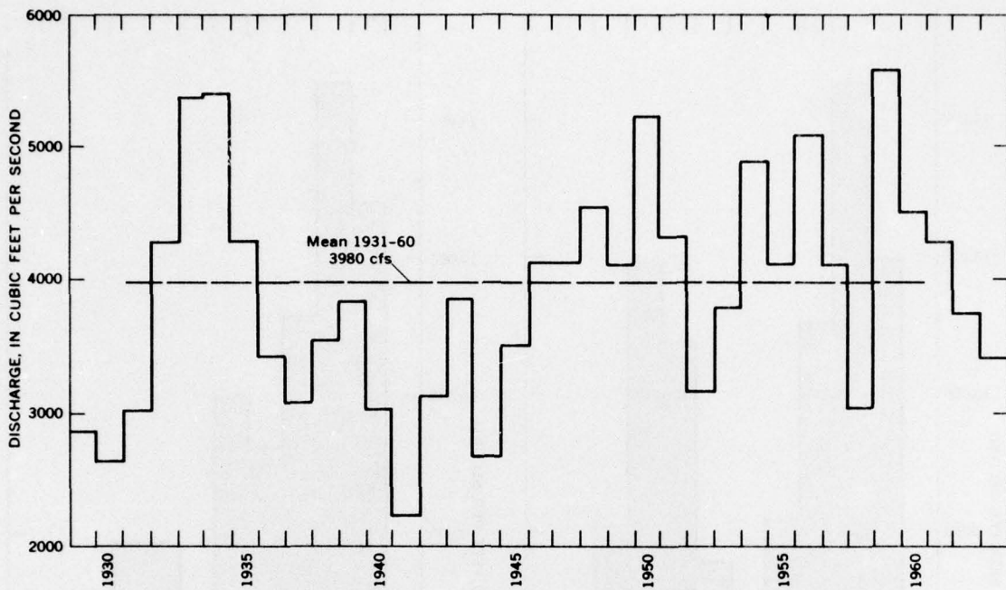
FIGURE 56.—Annual discharges, Skykomish River near Gold Bar.
