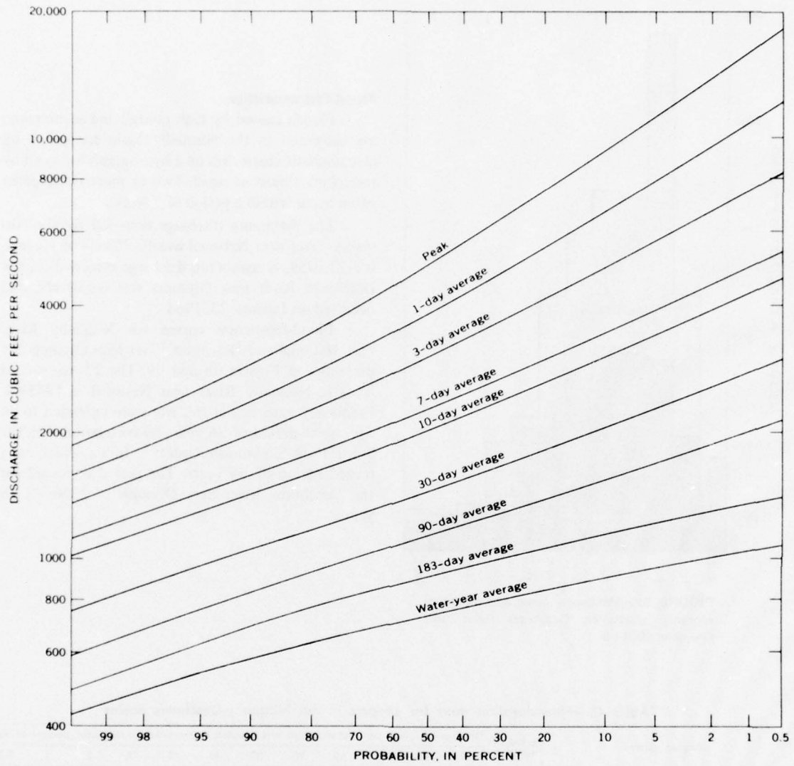
FIGURE 98.—Probability curves of annual maximum flows for specified time periods, Nisqually River near National.
