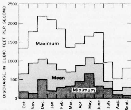
FIGURE 26.—Maximum, mean and minimum monthly discharges, South Fork Nooksack River near Wickersham, 1931-60.
