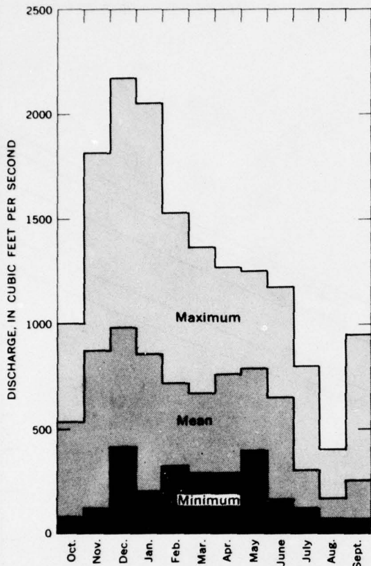
FIGURE 62.—Maximum, mean and minimum monthly discharges, Tolt River near Carnation, 1931-60.
