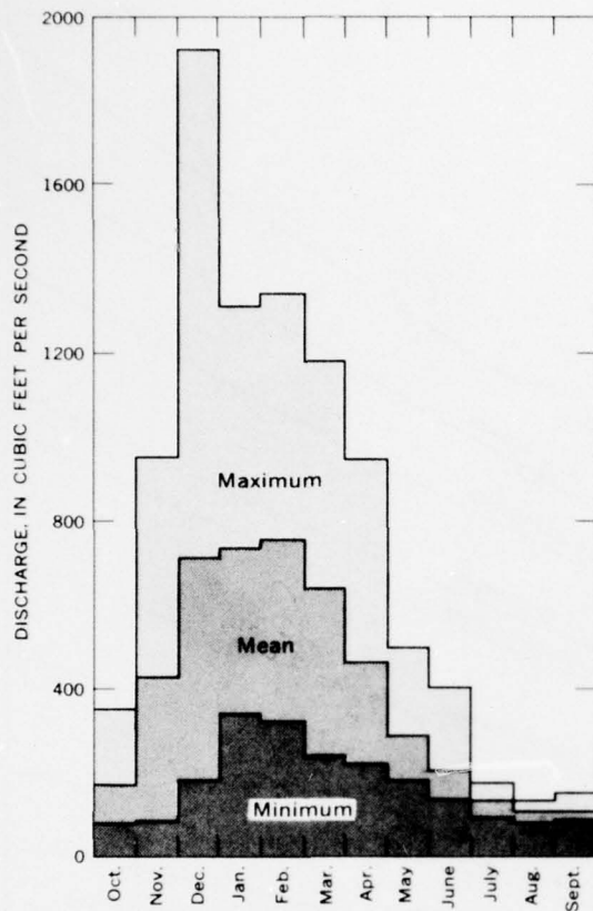
FIGURE 97.—Maximum, mean and minimum monthly discharges, Deschutes River near Olympia, 1931-60.
