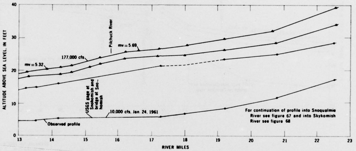
FIGURE 66.—Water-surface profile of Snohomish River, mile 3.5-23.
