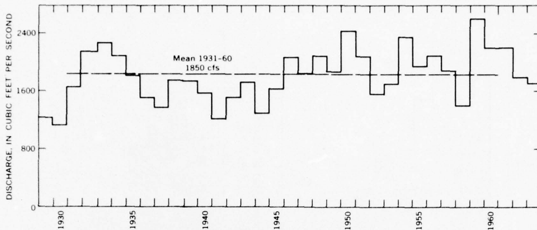
FIGURE 46.—Annual discharges, North Fork Stillaguamish River near Arlington.
