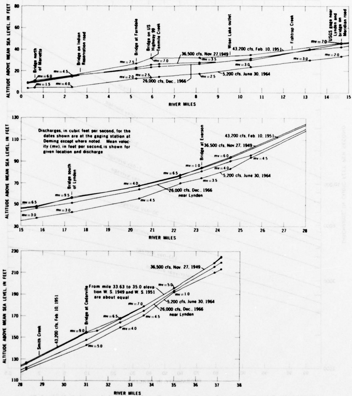
FIGURE 29.—Water-surface profile of Nooksack River, mile 0-37.
