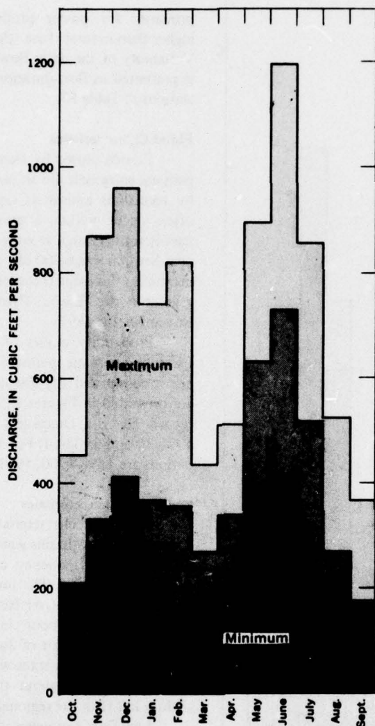
FIGURE 118.—Maximum, mean and minimum monthly discharges, Dungeness River near Sequim, 1931-60.
