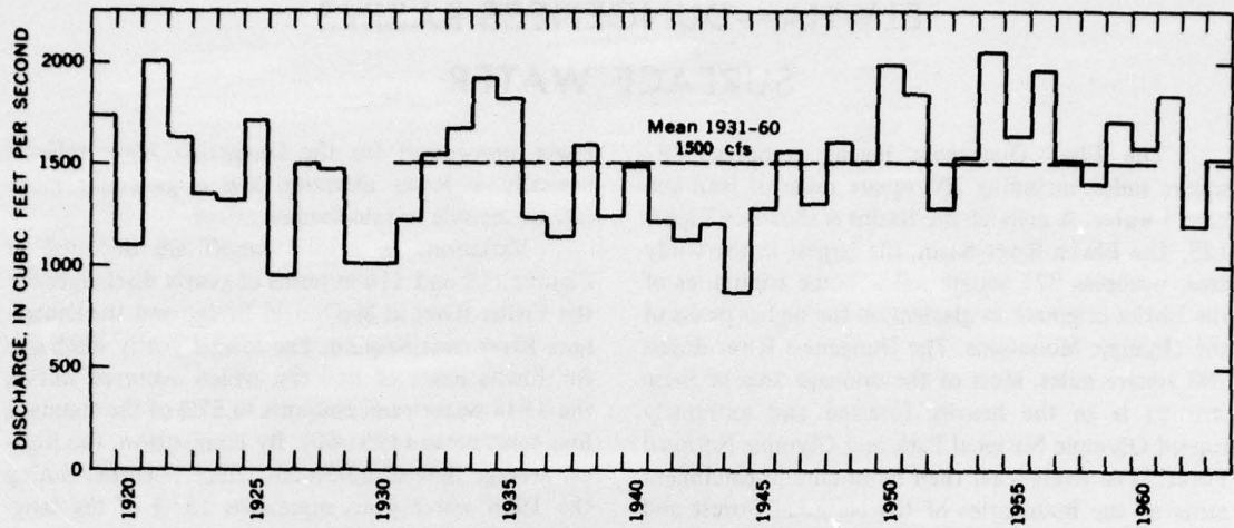
FIGURE 115.—Annual discharges, Elwha River at McDonald Bridge near Port Angeles.
