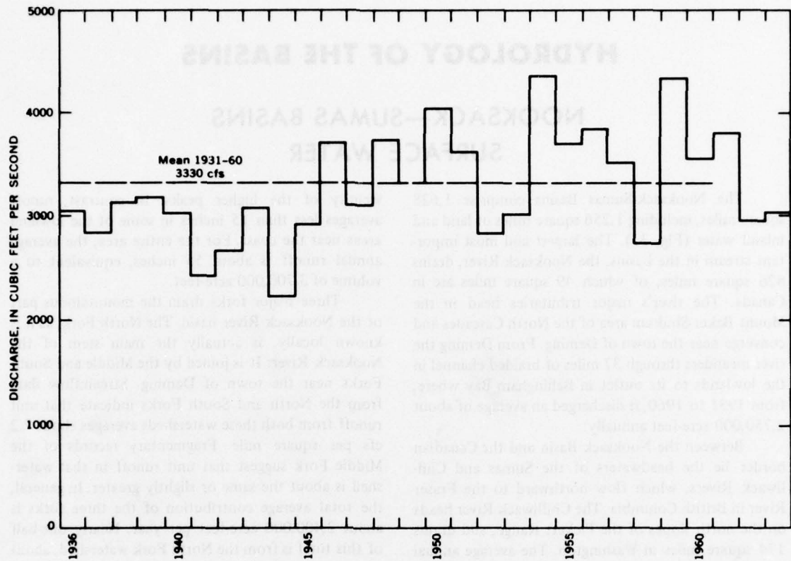
FIGURE 24.—Annual discharges, Nooksack River at Deming.
