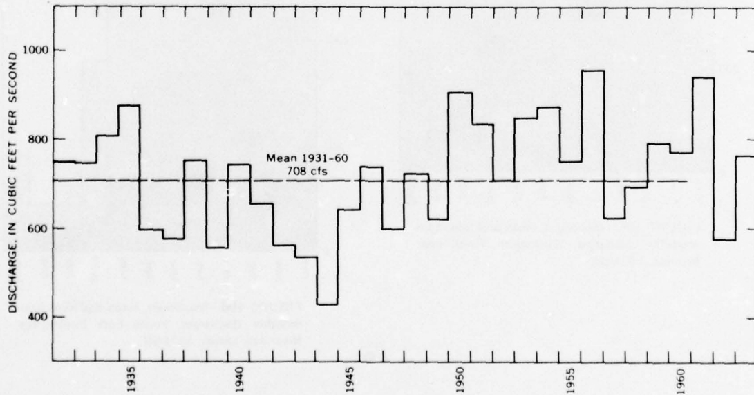
FIGURE 104.—Annual discharges, South Fork Skokomish River near Union.
