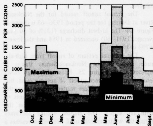
FIGURE 25.—Maximum, mean and minimum monthly discharges, Nooksack River below Cascade Creek near Glacier, 1931-60.
