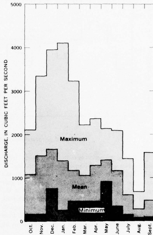
FIGURE 48.—Maximum, mean and minimum monthly discharges, South Fork Stillaguamish River near Granite Falls, 1931-60.
