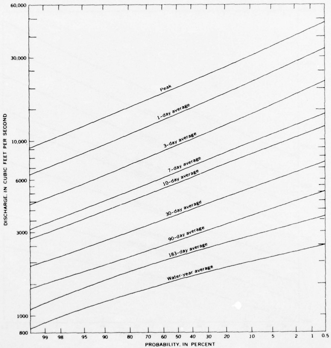
FIGURE 50.—Probability curves of annual maximum flows for specified time periods, South Fork Stillaguamish River above Jim Creek near Arlington.
