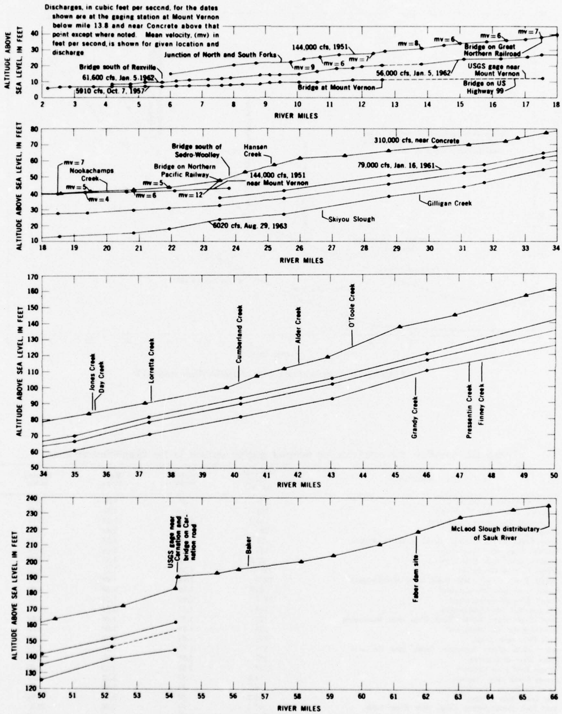
FIGURE 40.—Water-surface profile of Skagit River, via North Fork, mile 2-66.
