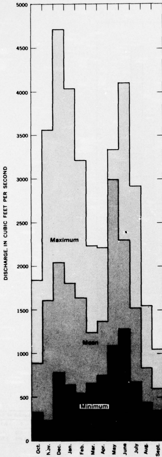
FIGURE 117.—Maximum, mean and minimum monthly discharges, Elwha River near Port Angeles, 1931-60.
