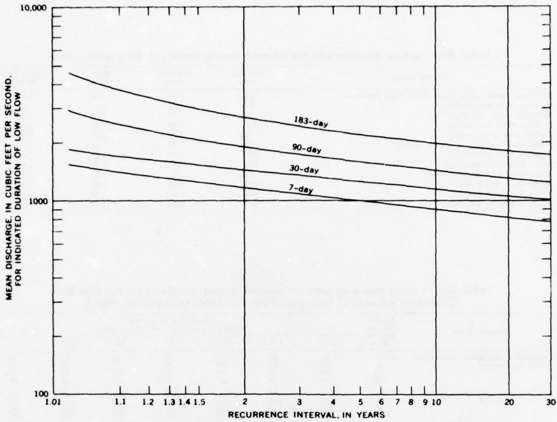
FIGURE 91.—Low-flow frequency, Puyallup River at Puyallup, 1946-63.
