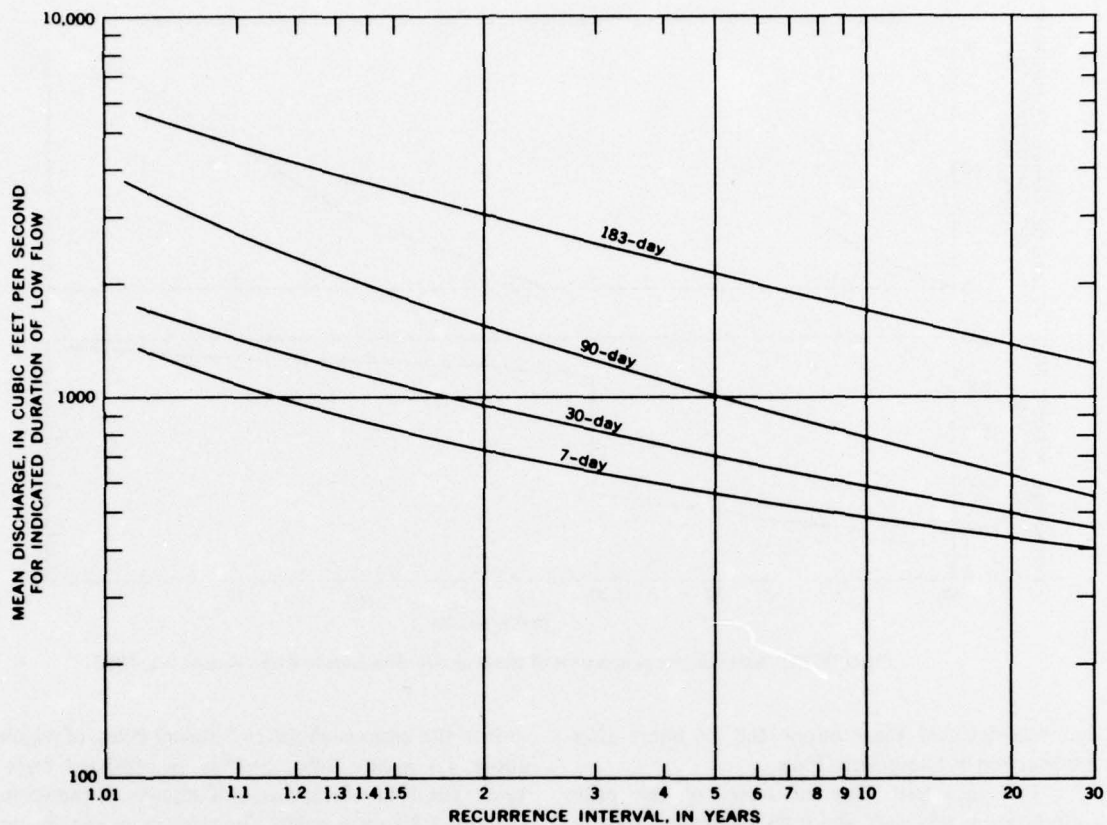
FIGURE 70.—Low-flow frequency, Skykomish River near Gold Bar, 1946-63.
