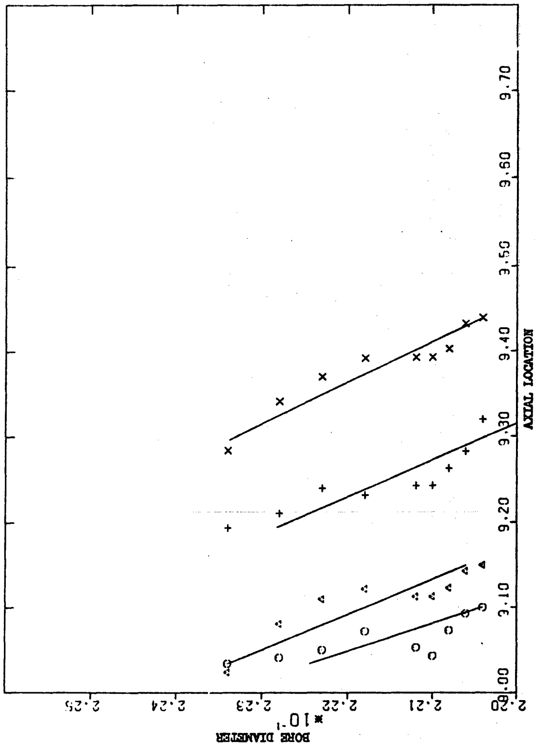
FIGURE 74 - Variation of Bore Shape for Gun Number 19
