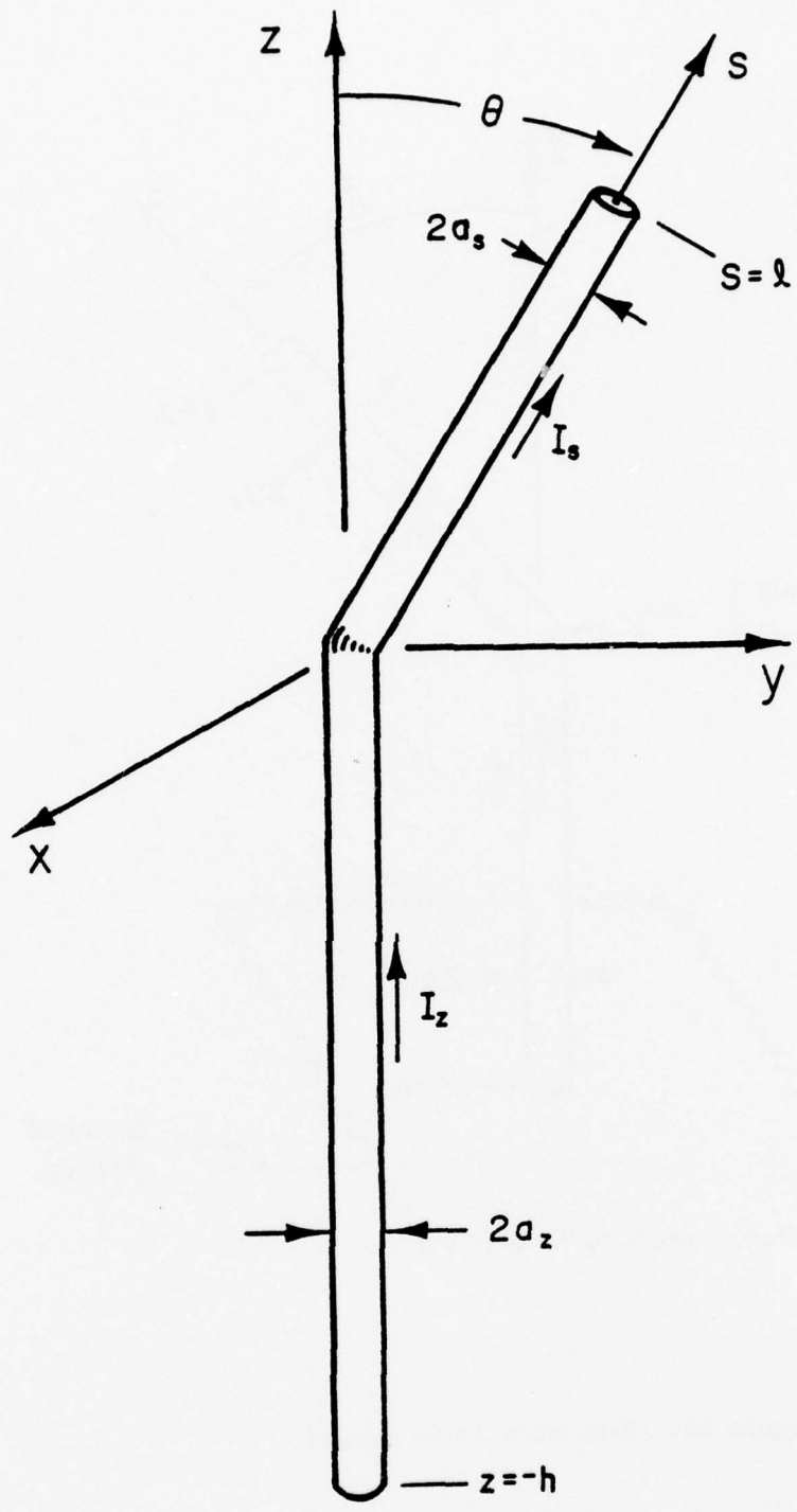
Figure 25. Bent Wire
