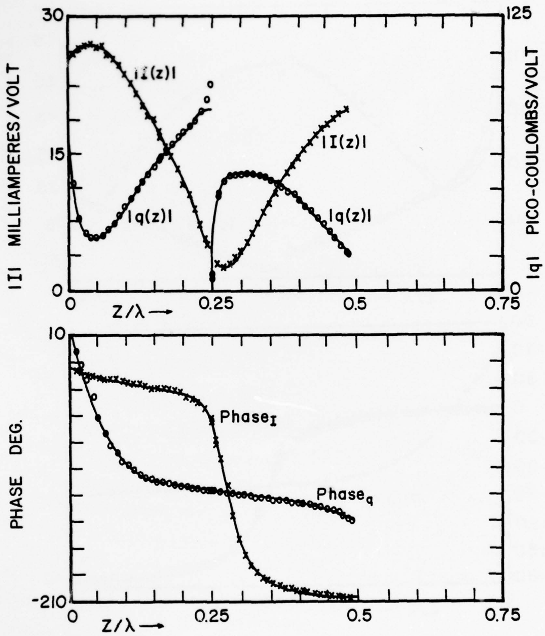
Figure 42. Stepped-Radius Antenna, h_1 = \lambda/4 , h_2 = \lambda/2 Current and Charge
