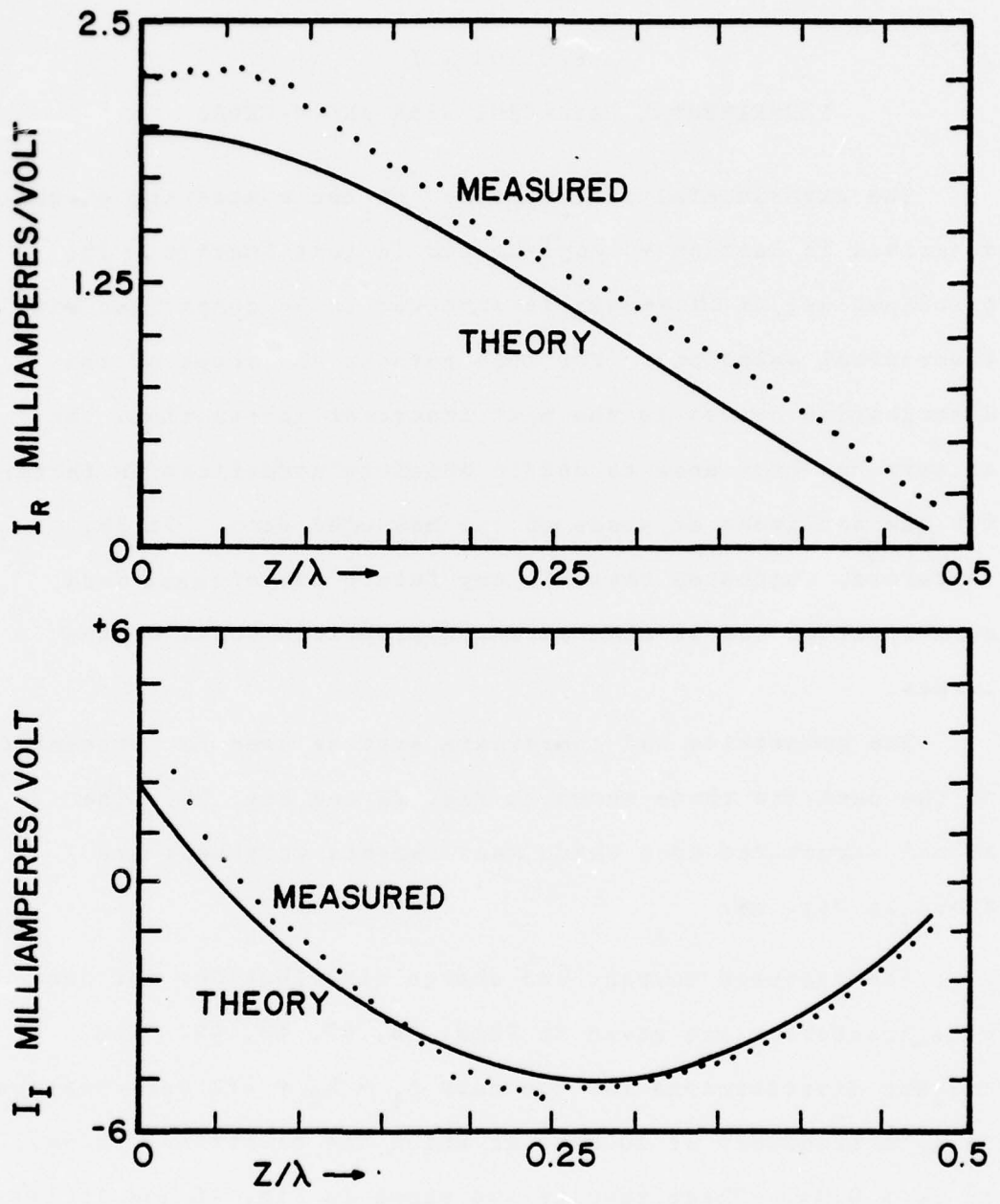
Figure 44. Stepped-Radius Antenna, h_1 = \lambda/4 , h_2 = \lambda/4 I_R, I_I Theory vs. Experiment
