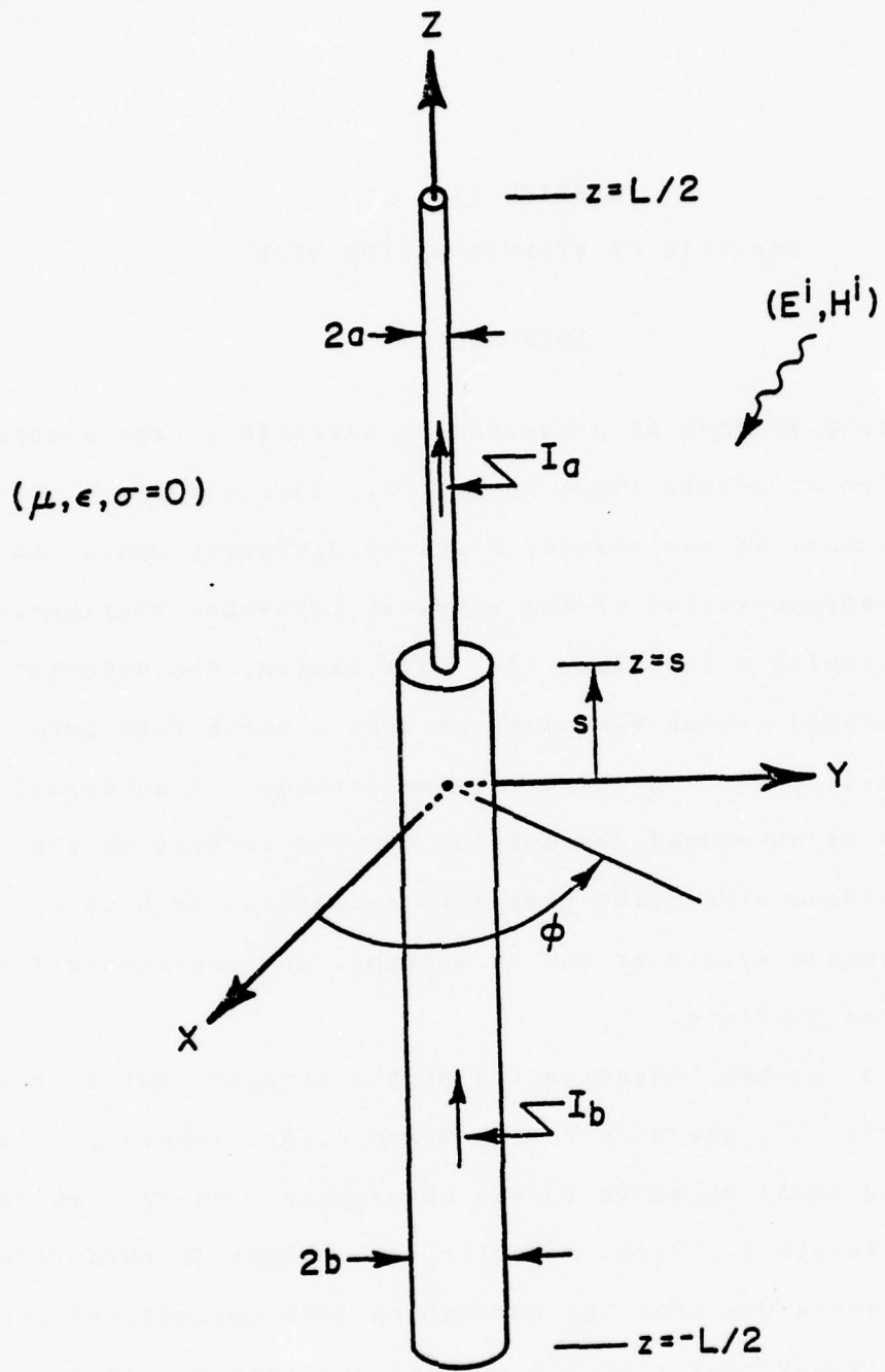
Figure 7. Stepped-Radius Wire
