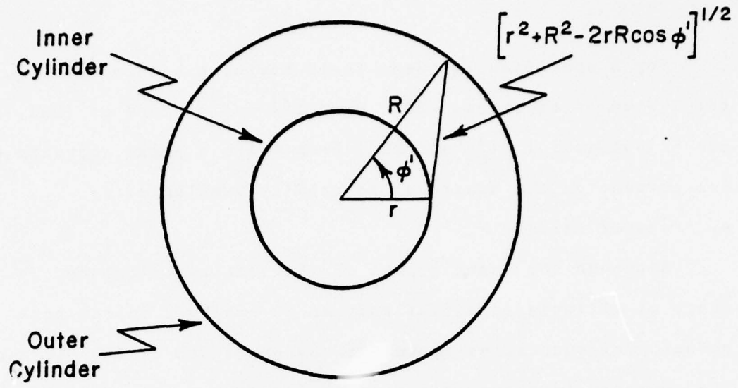
Figure 11. Distance in Transverse Plane between Points on Coaxial Cylinders
