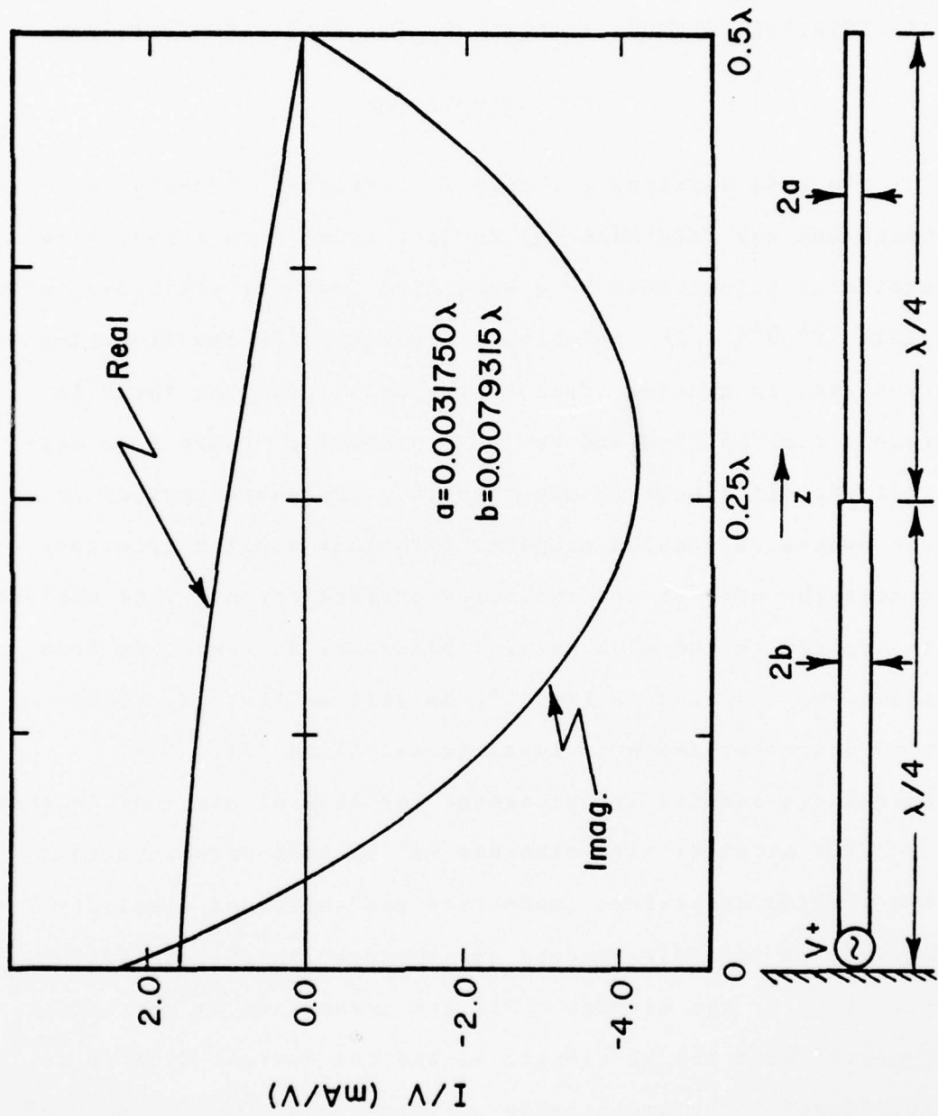
Figure 24. Current on Half-Wavelength Stepped-Radius Monopole above Ground
