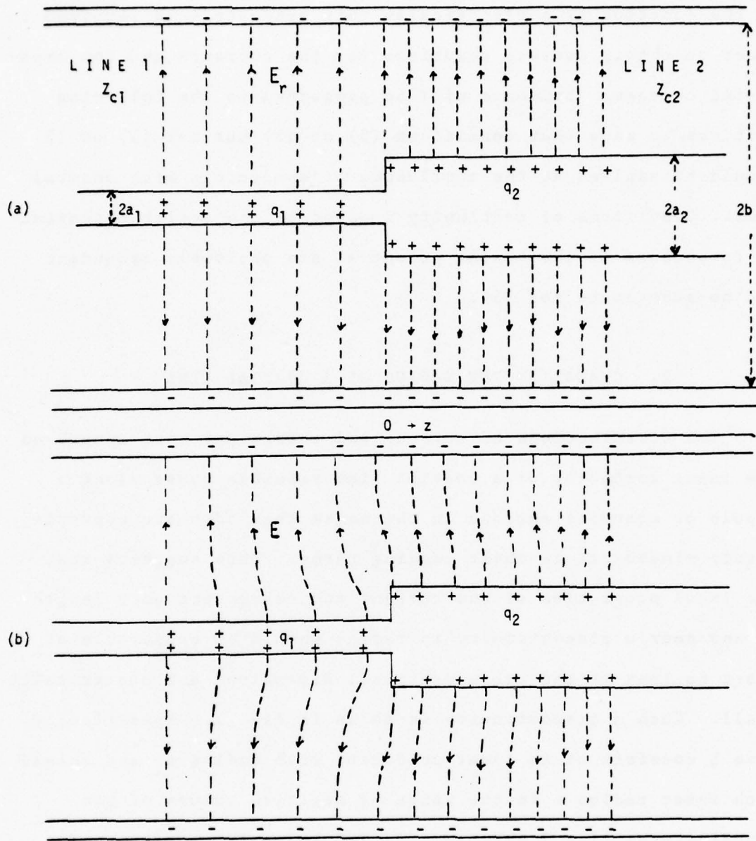
Figure 1. (a) Zero-Order, (b) Approximate Actual Distributions of Charge per Unit Length and Radial Electric Field in a Coaxial Line.
