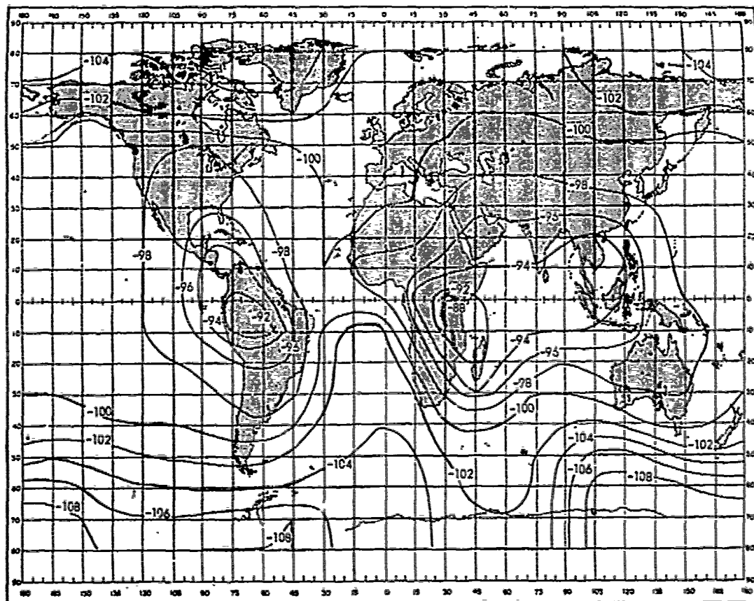
Fig. 24 — Expected atmospheric noise at 10 kc/s in decibels relative to 1 \text{ v/m}/\sqrt{\text{c/s}} (data from CCIR 322)
