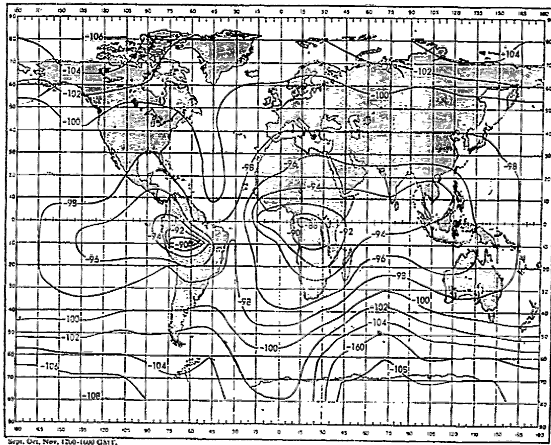
Fig. 25 — Expected atmospheric noise at 10 kc/s in decibels relative to 1 \text{ v/m}/\sqrt{\text{c/s}} (data from CCIR 322)
