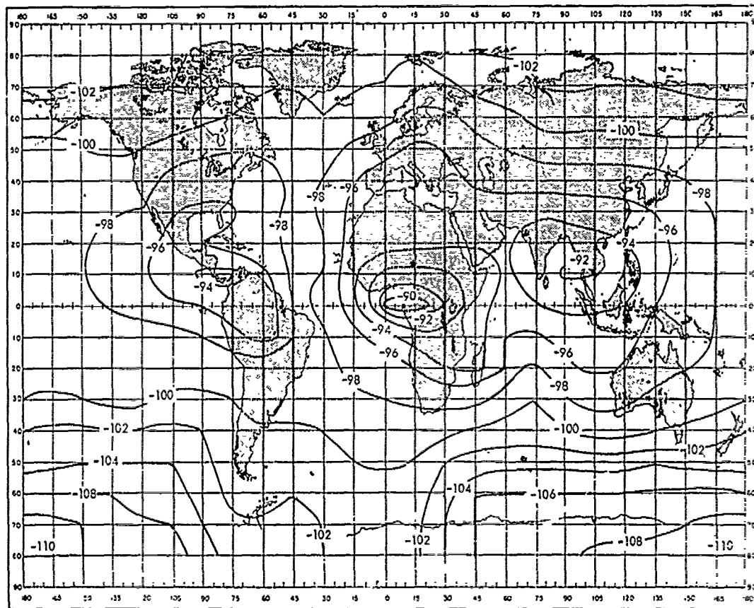
Fig. 13 — Expected atmospheric noise at 10 kc/s in decibels relative to 1 \text{ v/m}/\sqrt{\text{c/s}} (data from CCIR 322)
