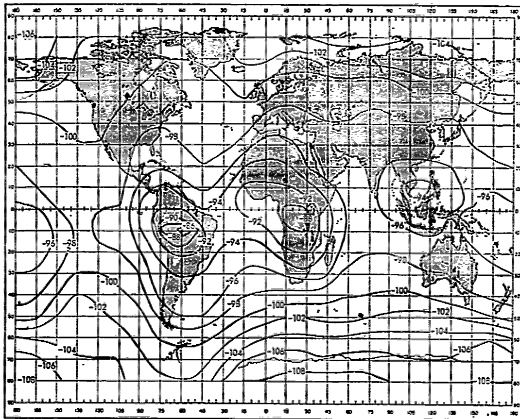
Fig. 26 — Expected atmospheric noise at 10 kc/s in decibels relative to 1 v/m/kc/s (data from CCIR 322)
