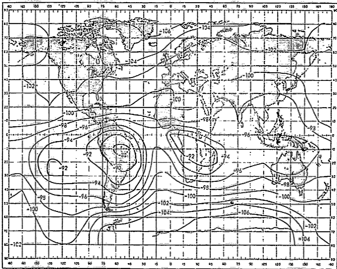
Fig. 9 — Expected atmospheric noise at 10 kc/s in decibels relative to 1 \text{ v/m}/\sqrt{c/s} (data from CCIR 322)
