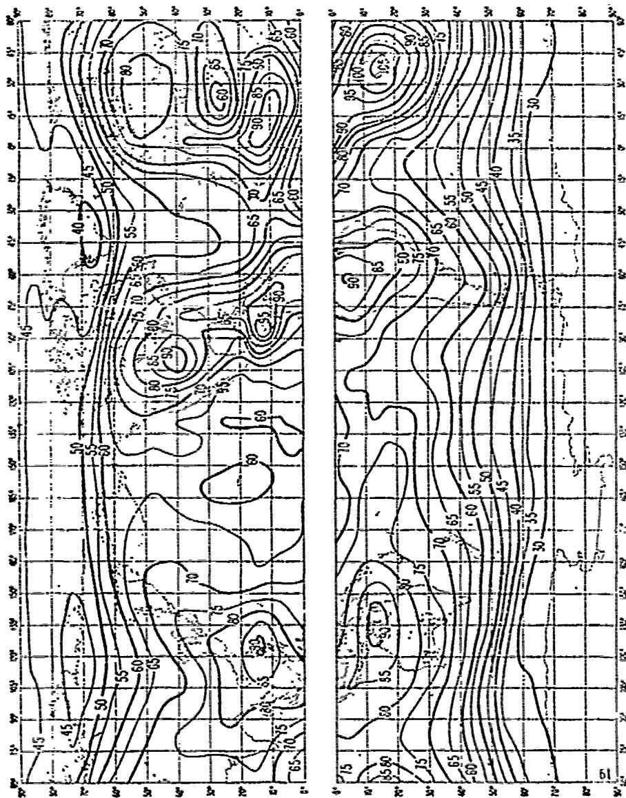
Expected values of atmospheric radio noise, F_{0m1} , (db above kT_b at 1 Mc/s) (Summer, 2000-2400 h.)
