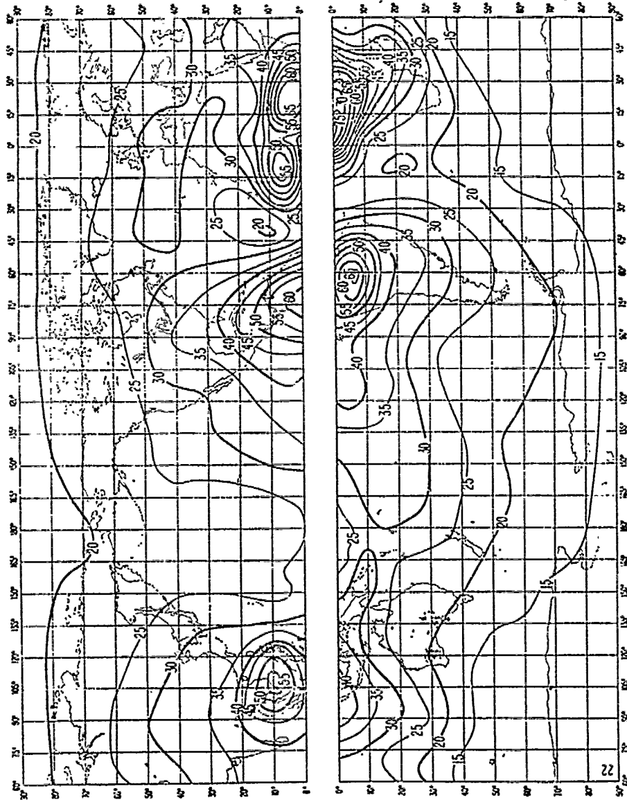
Expected values of atmospheric radio noise, F_{mn} (db above kT_{b0} at 1 Mc/s) (Autumn: 0800-1200 h.)
