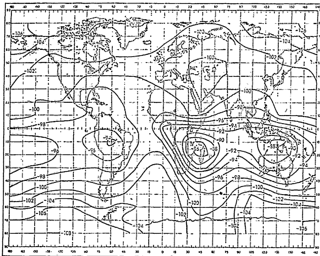
Fig. 6 — Expected atmospheric noise at 10 kc/s in decibels relative to 1 \text{ v/m}/\sqrt{c/s} (data from CCIR 322)
