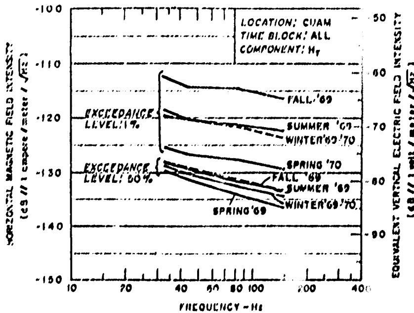
Fig. 6 - Spectra of 1 percent and 50 percent exceedance levels for H_T , Guam where H_T is the (H_z(0.01)^2 + H_y(0.01)^2)^{1/2} or (H_z(0.5)^2 + H_y(0.5)^2)^{1/2}
