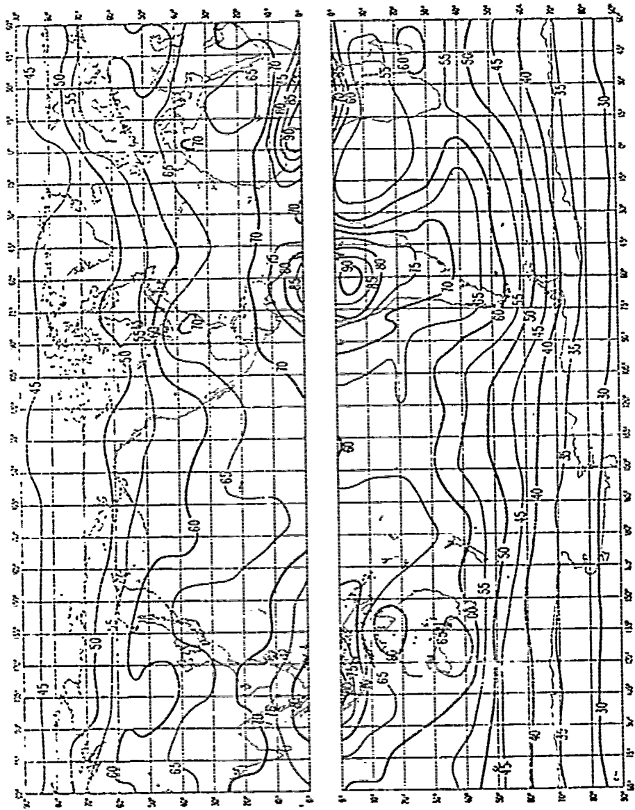
Expected values of atmospheric radio noise, F_{am} , (db above kT_{amb} at 1 Mc/s) (Winter: 2000-2400 h.)
