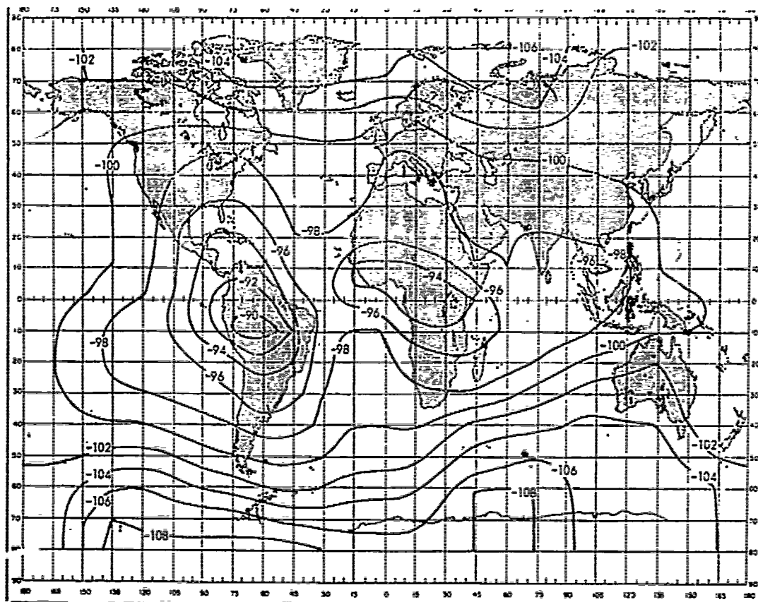
Fig. 22 — Expected atmospheric noise at 10 kc/s in decibels relative to 1 \text{ v/m}/\sqrt{\text{c/s}} (data from CCIR 322)
