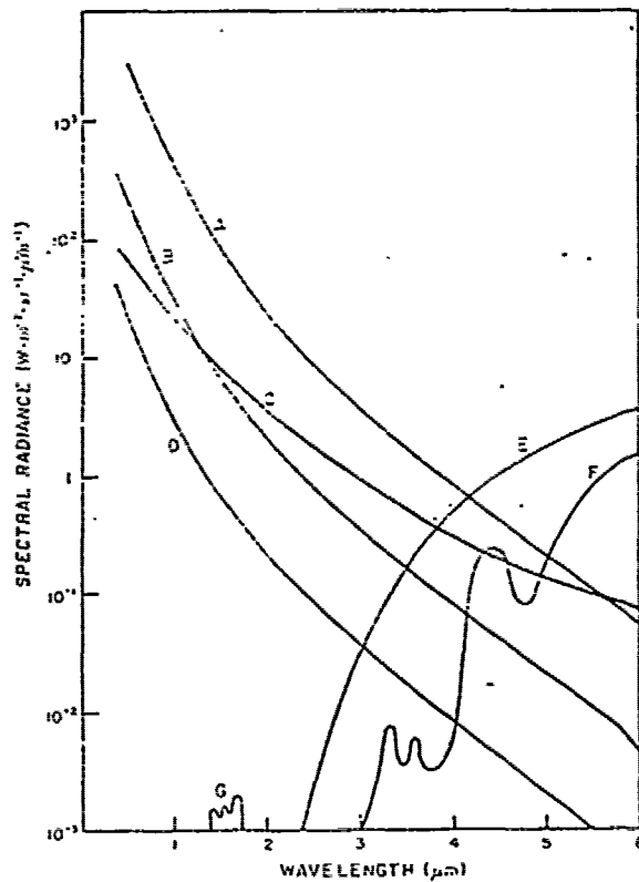
Day sky background data (absorption bands of Fig. 2 not included). Curve A : scattered sunlight, 94 km visibility, \theta = 10^\circ , \Phi = 60^\circ . Curve B : scattered sunlight, 94 km visibility, \theta = 40^\circ , \Phi = 60^\circ . Curve C : cloud or fog transmitting 50 percent, \theta = 30^\circ , \Phi = 50^\circ . Curve D : scattered sunlight, 94 km visibility, \theta = 90^\circ , \Phi = 60^\circ . Curve E : blackbody radiation at 283°K. Curve F : water vapor and CO 2 atmospheric emission. Curve G : bright aurora. \theta is angle through which light is scattered into field of view and \Phi is the zenith angle of field of view (after Stewart and Hershfield [8]).
