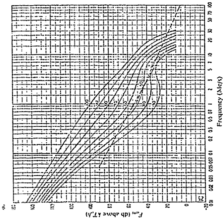
Variation of radio noise with frequency (Autumn; 2000-2400 h.)
