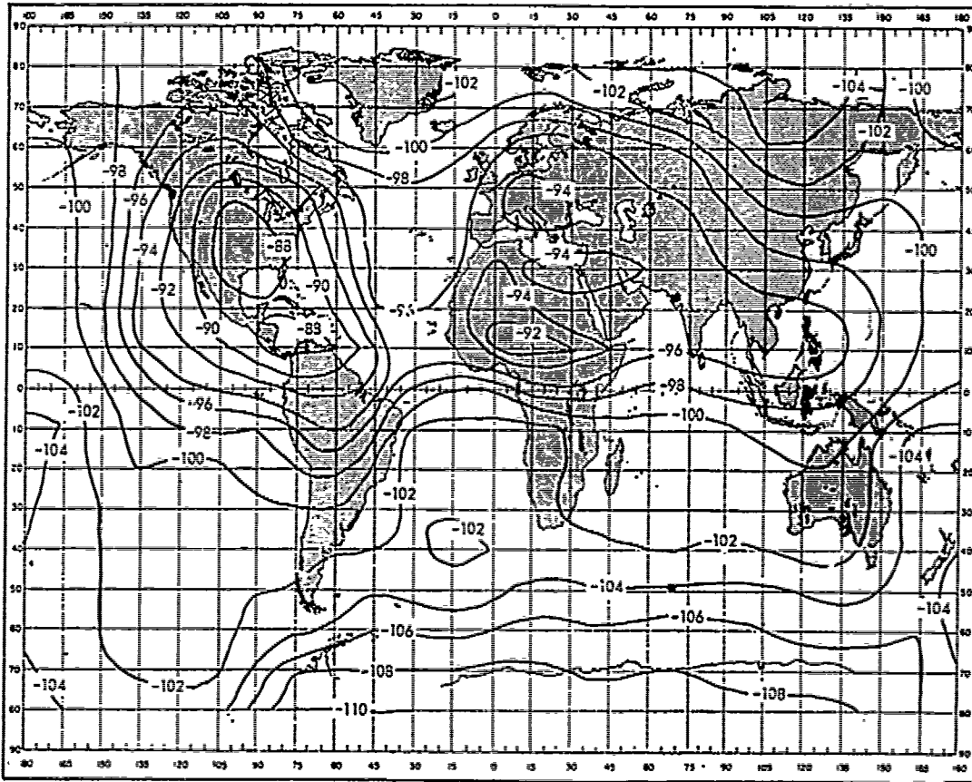
Fig. 21 — Expected atmospheric noise at 10 kc/s in decibels relative to 1 \text{ v/m}/\sqrt{c/s} (data from CCIR 322)
