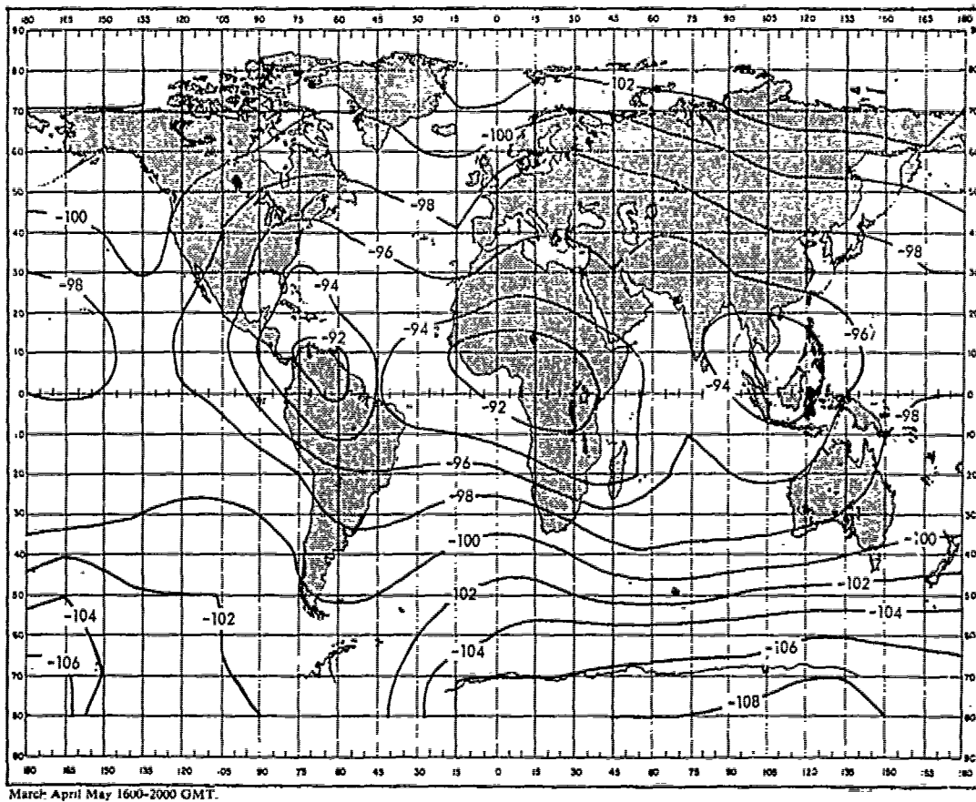
Fig. 14 — Expected atmospheric noise at 10 kc/s in decibels relative to 1 \text{ v/m}/\sqrt{c/s} (data from CCIR 322)
