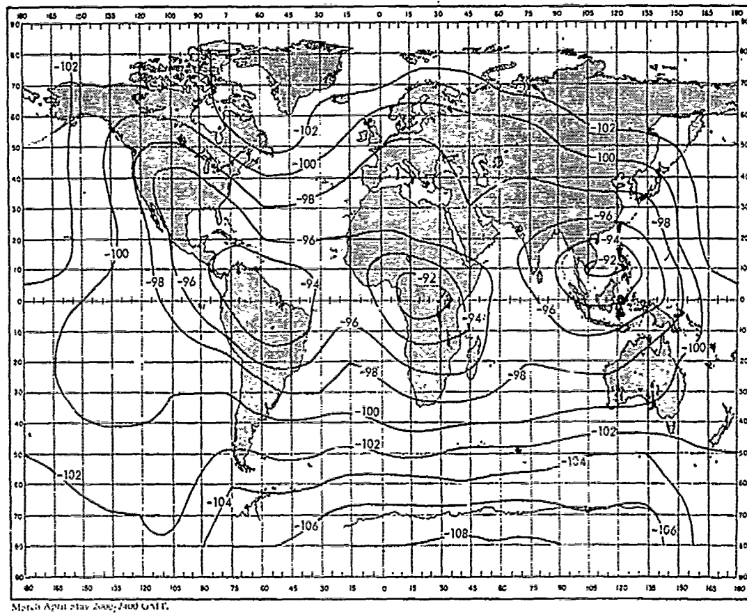
Fig. 15 — Expected atmospheric noise at 10 kc/s in decibels relative to 1 \text{ v/m}/\sqrt{c/s} (data from CCIR 322)
