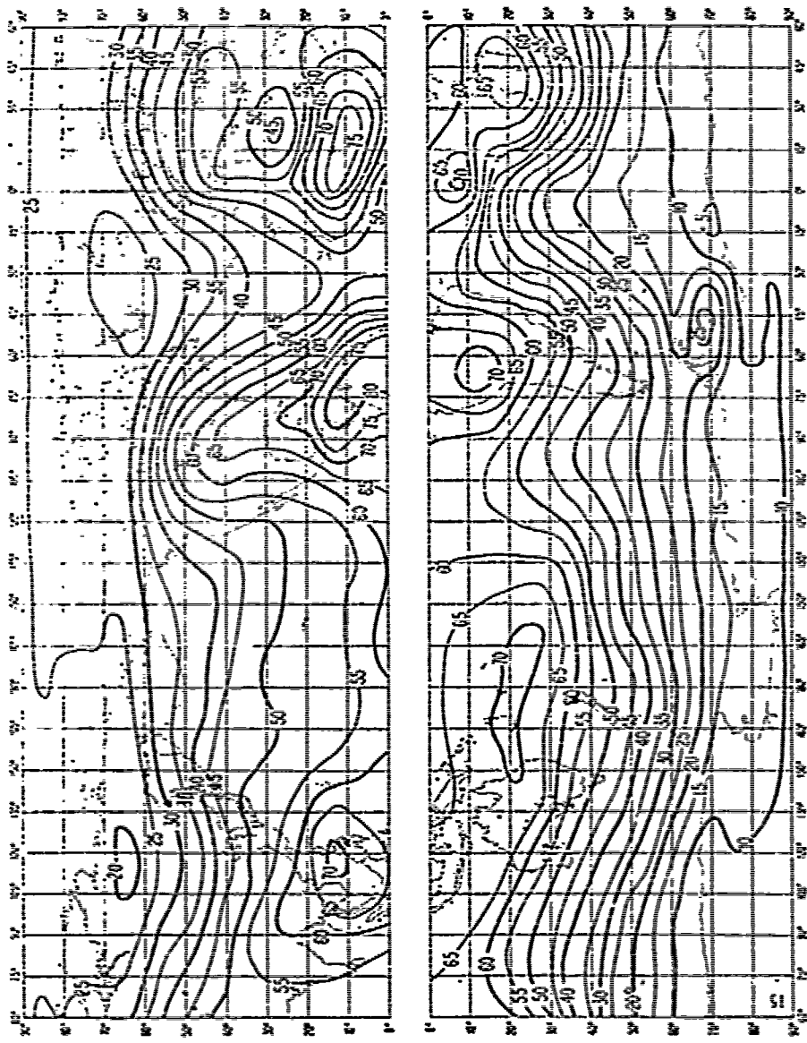
Expected value of atmospheric radio noise, f_{mn} (dB above kT_b at 1 Mc/s) (Summer, 0400-0800 h.)
