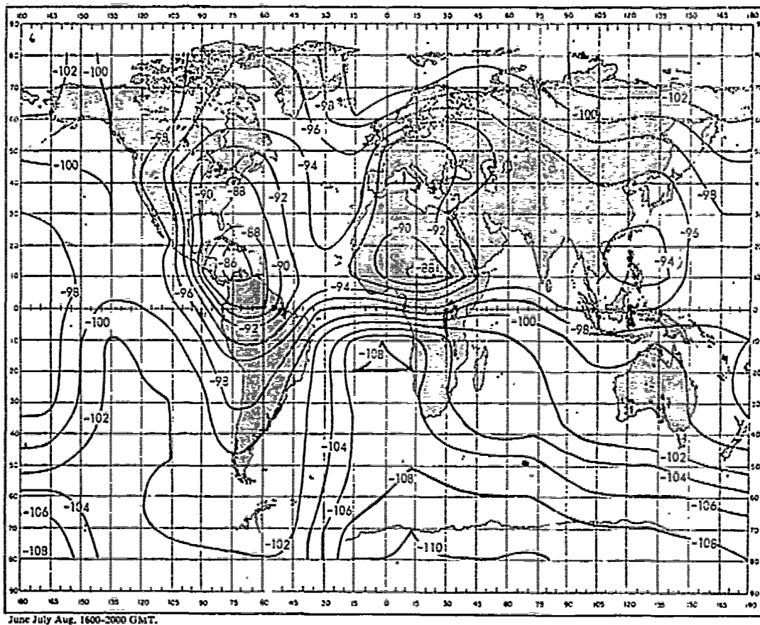
Fig. 20 — Expected atmospheric noise at 10 kc/s in decibels relative to 1 \text{ v/m}/\sqrt{c/s} (data from CCIR 322)
