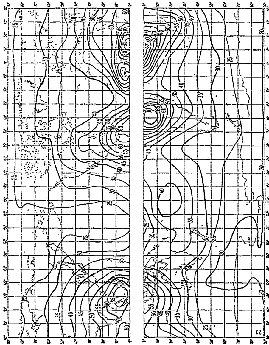
Expected values of atmospheric radio noise, F_{atm} , (db above kT_b at 1 Mc/s) (Autumn: 1200-1600 h.)
