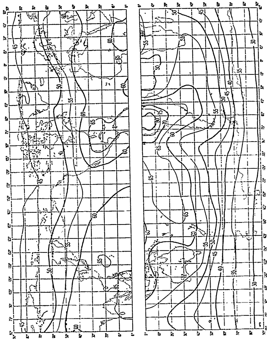
Expected values of atmospheric radio noise, \Gamma_{fm} , (db above fT_b at 1 Mc/s) (Winter: 0400-0800 h.)
