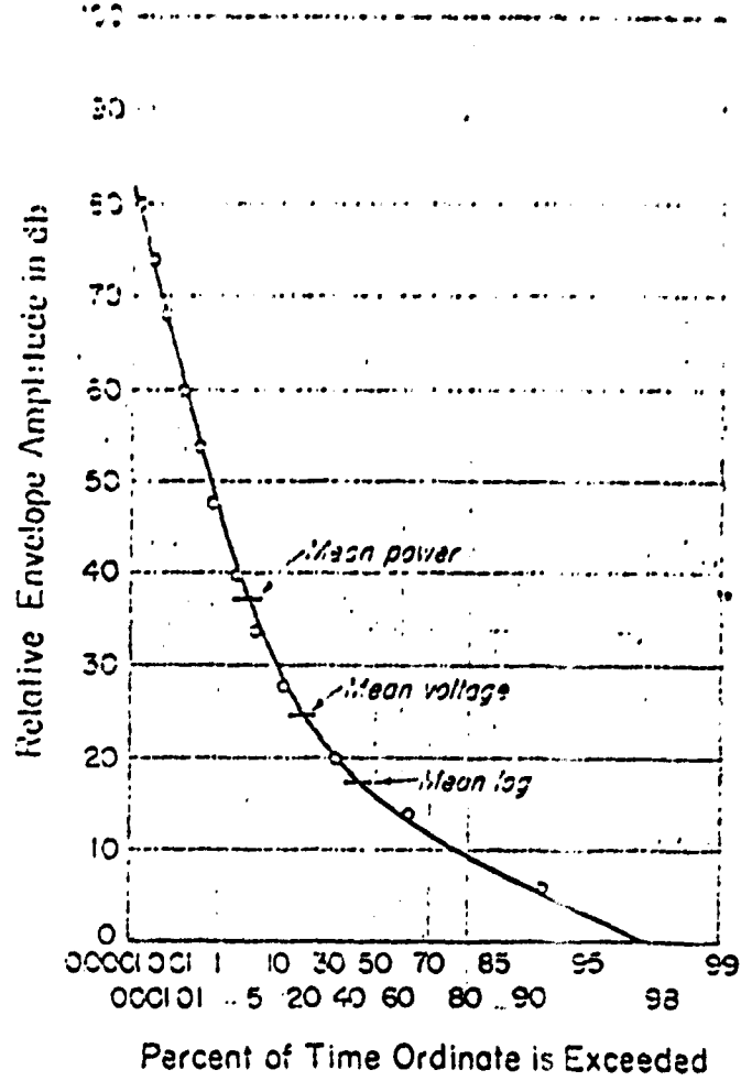
Fig. 1 — Typical amplitude-time distribution of short-term variations
