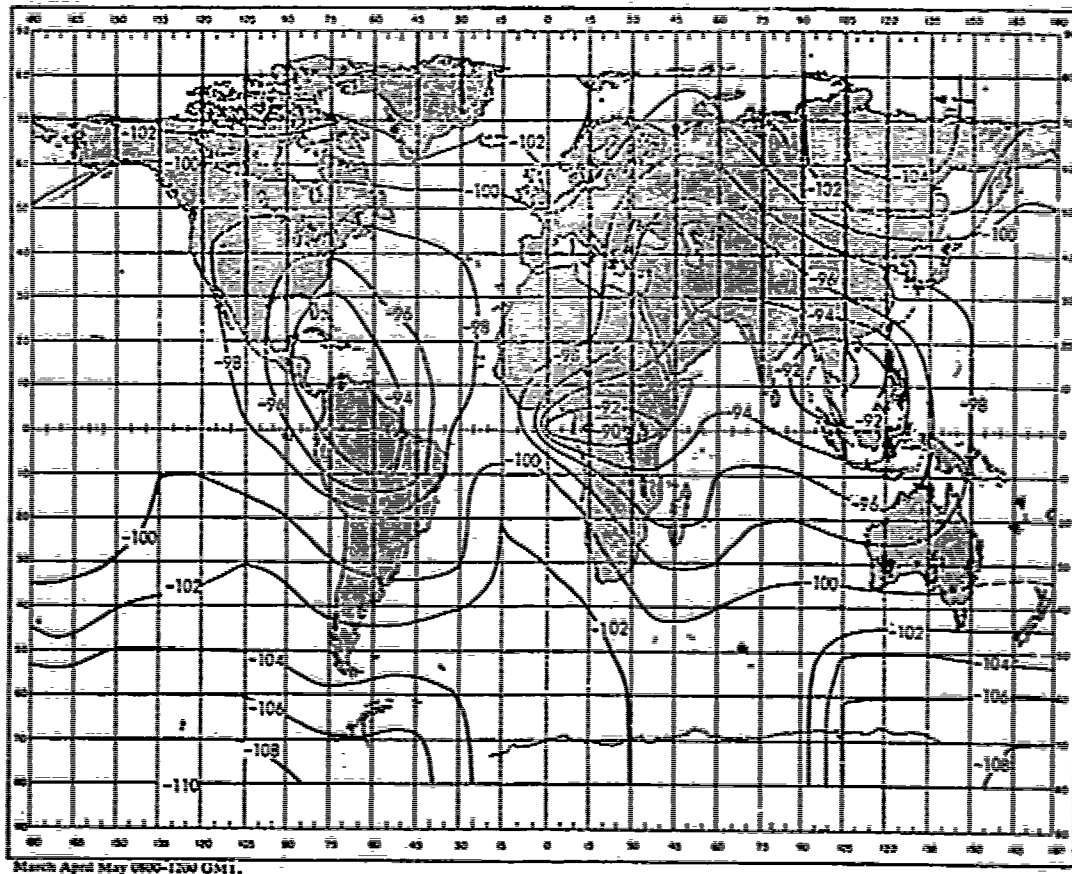
Fig. 12 — Expected atmospheric noise at 10 kc/s in decibels relative to 1 \text{ v/m}/\sqrt{c/s} (data from CCIR 322)
