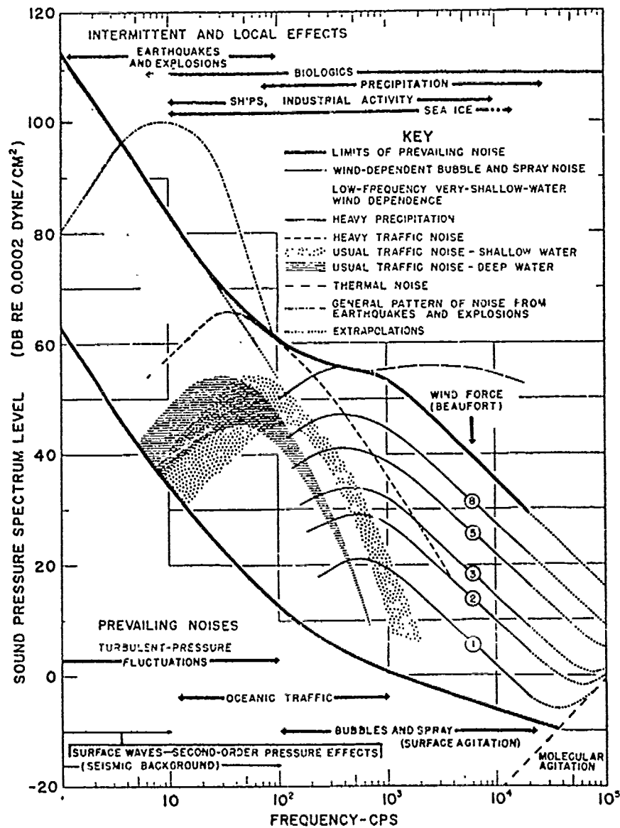
Fig. 2 — A composite of ambient-noise spectra, summarizing results and conclusions concerning spectrum shape and level and probable sources and mechanisms of the ambient noise in various parts of the spectrum between 1 cps and 100 kc. The key identifies component spectra. Horizontal arrows show the approximate frequency band of influence of the various sources. An estimate of the ambient noise to be expected in a particular situation can be made by selecting and combining the pertinent component spectra.
