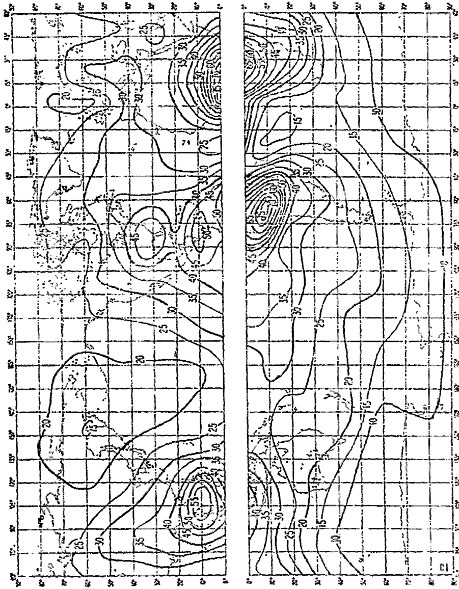
Expected values of atmospheric radio noise, F_{min} , (db above k/f_o F_2 at 1 Mc/s) (Sp. int. 0.600-1.200 Mc/s)
