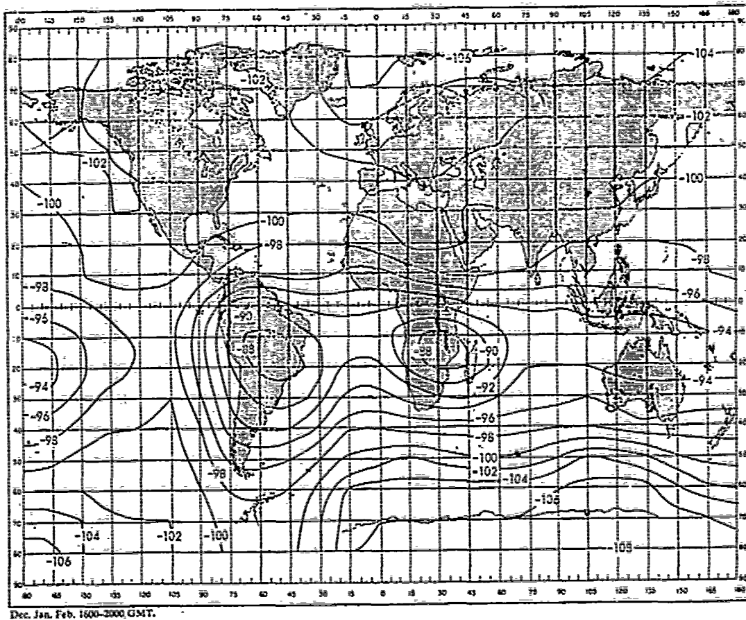
Fig. 8 — Expected atmospheric noise at 10 kc/s in decibels relative to 1 \text{ v/m}/\sqrt{\text{c/s}} (data from CCIR 322)
