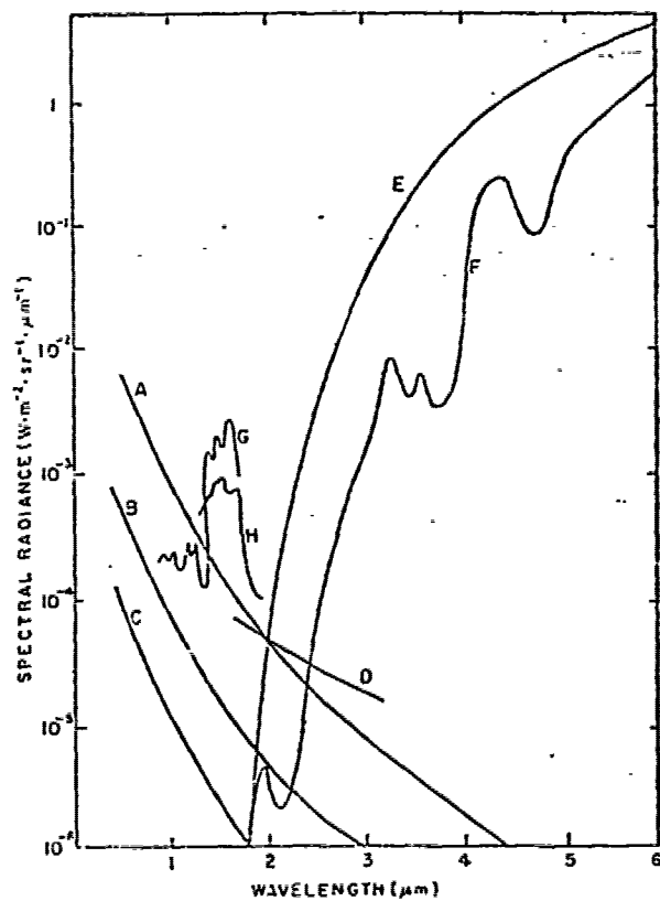
Night sky background data (absorption bands of Fig. 2 not included) Curve A : full Moon, 94 km visibility, \theta = 10^\circ , \Phi = 60^\circ . Curve B : full Moon, 94 km visibility, \theta = 40^\circ , \Phi = 60^\circ . Curve C : full Moon, 94 km visibility, \theta = 90^\circ , \Phi = 60^\circ . Curve D : maximum scatter from city lights. Curve E : blackbody radiation at 283°K. Curve F : water vapor and \text{CO}_2 atmospheric emission. Curve G : bright aurora. Curve H : airglow. \theta is angle through which light is scattered into field of view and \Phi is the zenith angle of field of view (after Stewart and Hopfield [8]).
