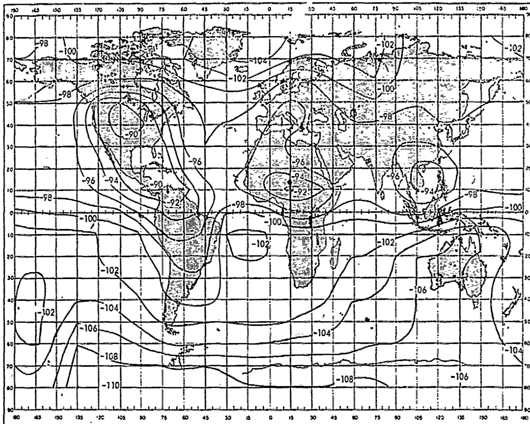
Fig. 16 -- Expected atmospheric noise at 10 kc/s in decibels relative to 1 \text{ v/m}/\sqrt{c/s} (data from CCIR 322)
