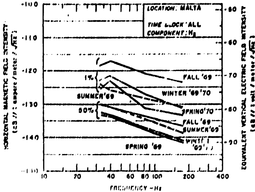
Fig. 5 - Spectra of 1 percent and 50 percent exceedance levels for H_z , Malta, for each season
