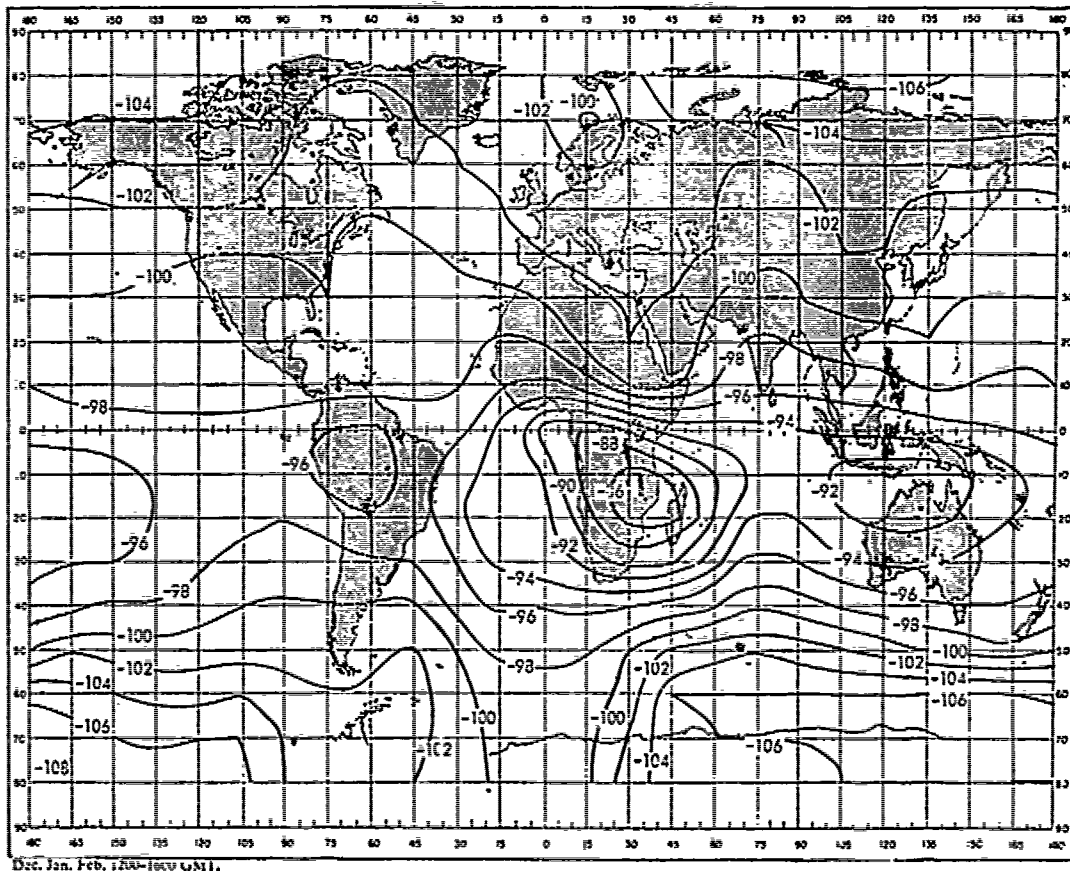
Fig. 7 — Expected atmospheric noise at 10 kc/s in decibels relative to 1 \text{ v/m}/\sqrt{\text{c/s}} (data from CCIR 322)
