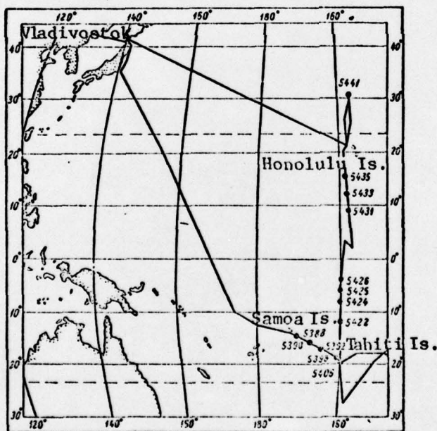
Schematic map of stations (closed circles) with underwater actinometric measurements in the Pacific Ocean. Arabic numerals near black circles indicate station numbers.
