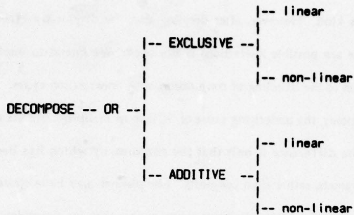
Figure 21. A Planning Taxonomy for Disjunction
