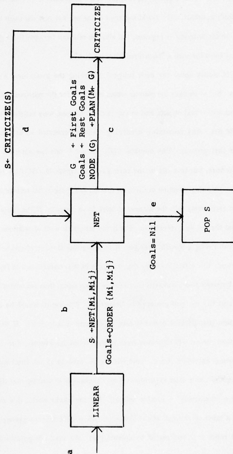
FIGURE 14 NET REFINEMENT
