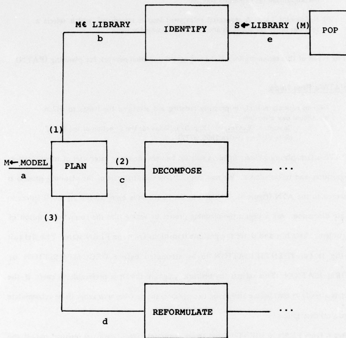
FIGURE 4 PATN's PLAN NODE
