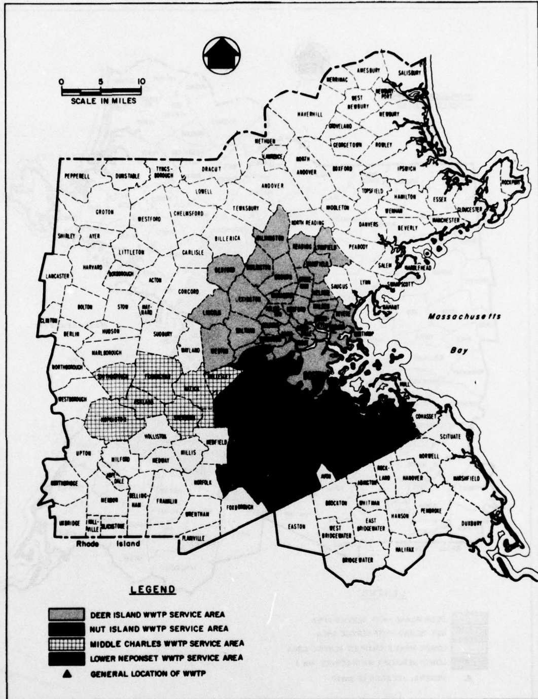
FIG. 5-1 ALTERNATIVE A
