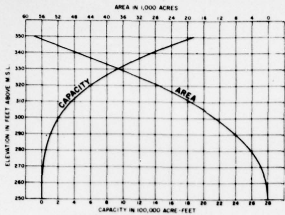
AREA-CAPACITY CURVES
