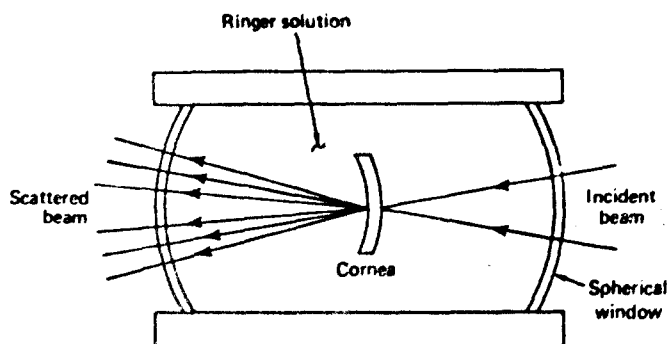
Fig. 1 Cornea Light-Scattering Sample Cell. (76-3/47)
