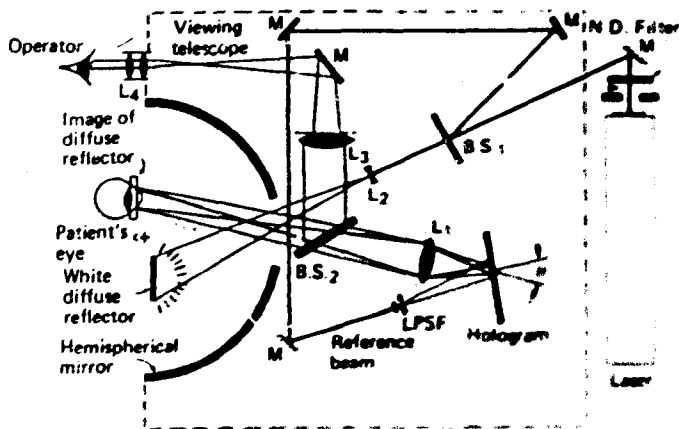
Fig. 1 Holographic Camera. (188761)
