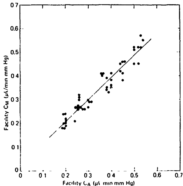
Fig 3 A Comparison of the Facility of Various Lengths of PE Tubing as Measured Directly by Bubble Movement in the Calibrated Pipette ( C_A ) and as Measured by the Constant-Pressure Tonographic Instrument ( C_M ) (76-3/41)
