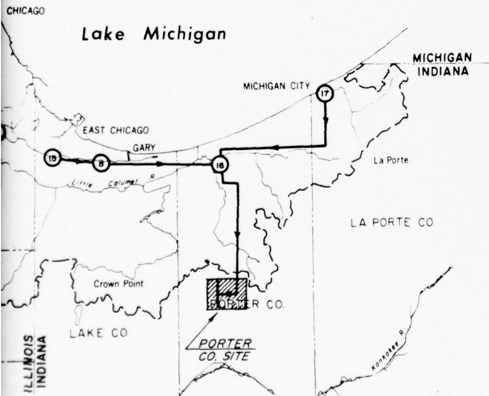
Figure D-II-C-6 AGRICULTURAL UTILIZATION OF ADVANCED BIOLOGICAL SLUDGE For ALTERNATIVE III D-II-C-14
