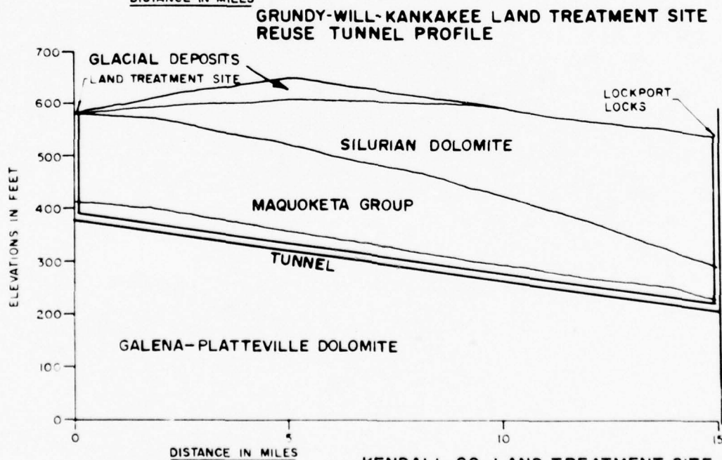
KENDALL CO. LAND TREATMENT SITE REUSE TUNNEL PROFILE
