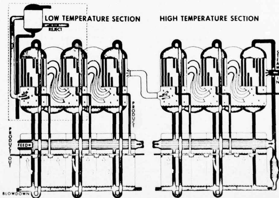
FIGURE R-30. COMBINATION VTE-MSF DISTILLATION PROCESS
