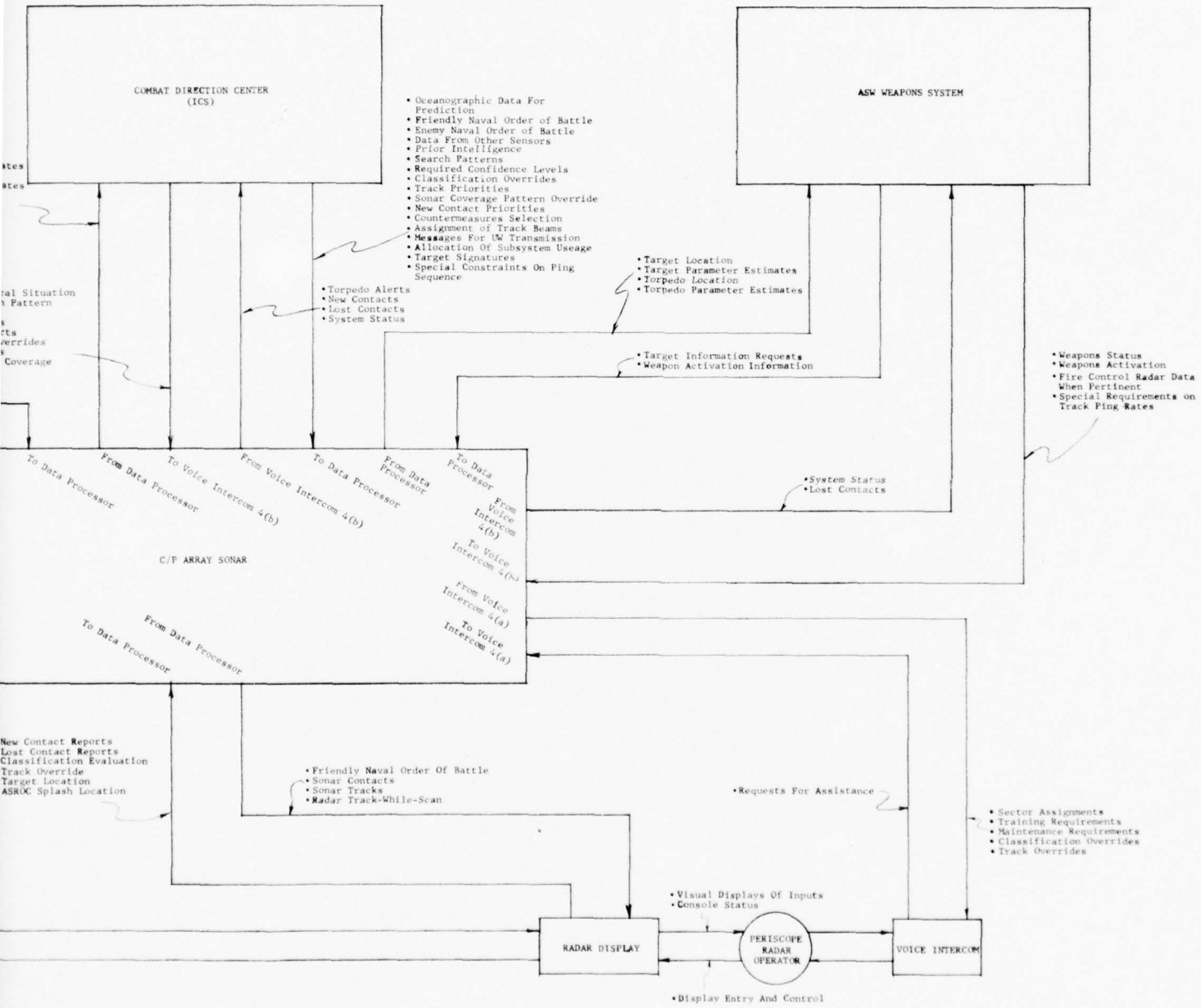
FIGURE 2.3.3-2 SONAR INTERFACE INFORMATION FLOW
