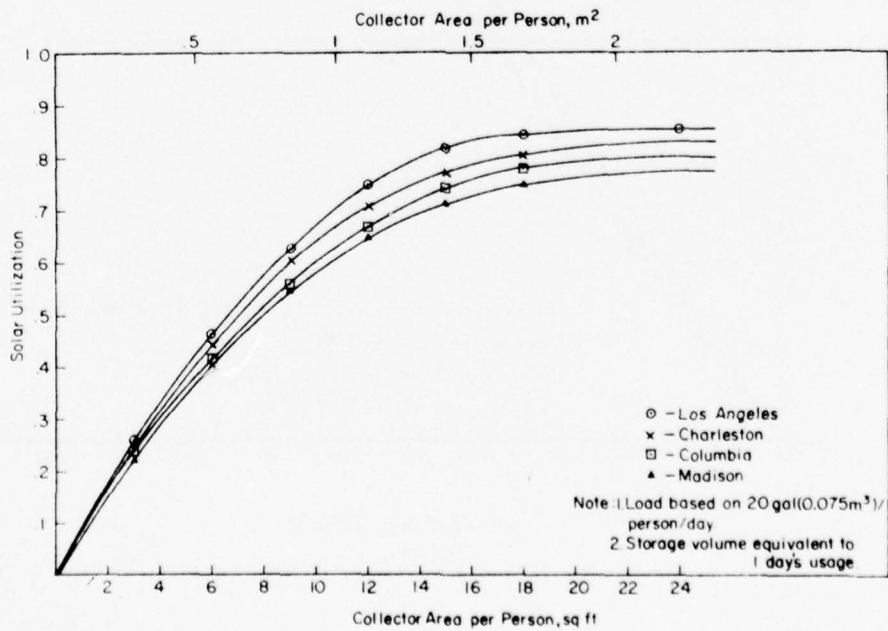
Figure 4. Collector area vs solar utilization.
