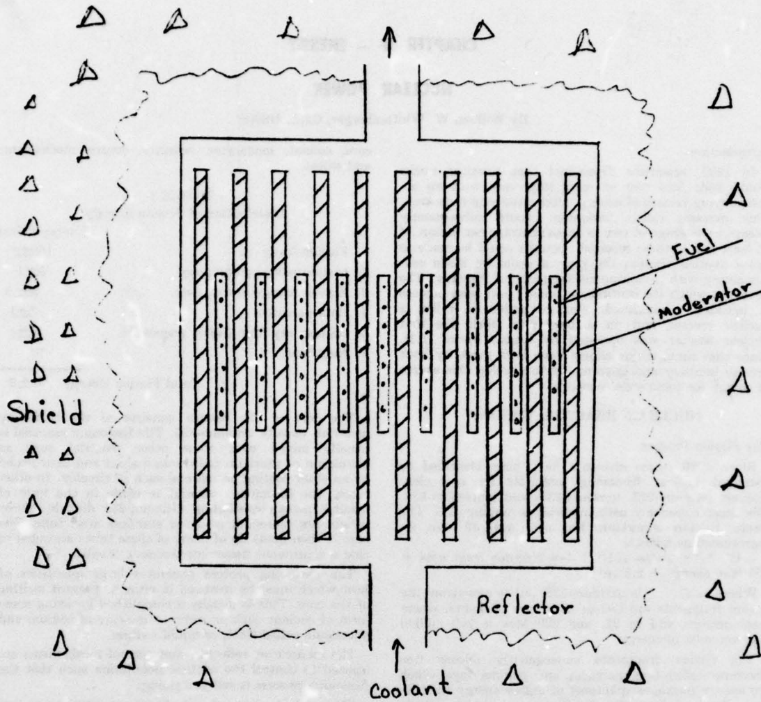
Figure 1. Reactor Core.
