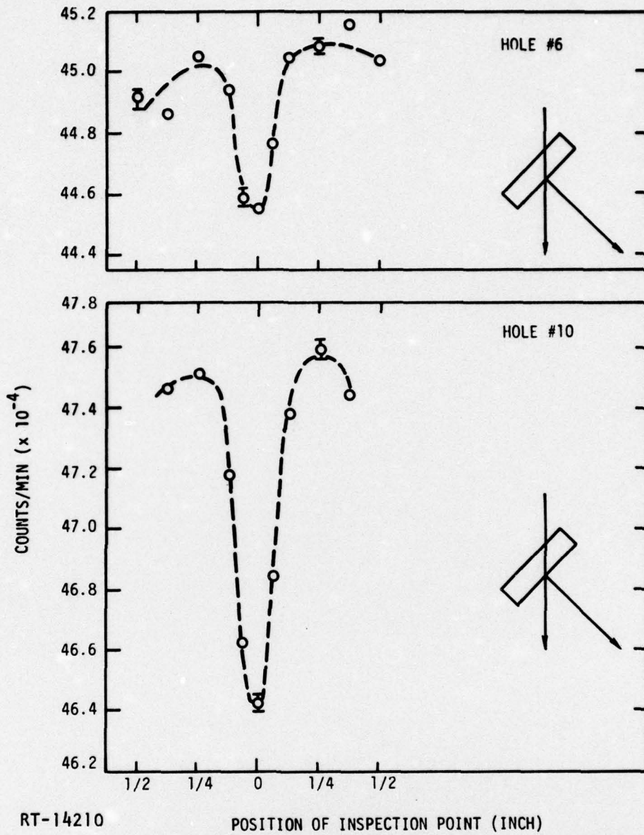
RT-14210 Figure 29. Response of the photon scattering gauge to holes 6 and 10 at one depth each
