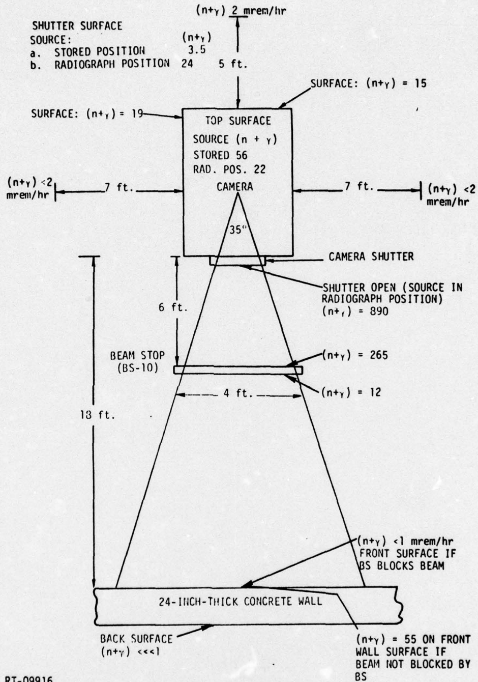
Figure 7. Camera radiation dose profile (10 mg 252 Cf) [all values of (n+γ) are mrem/hr]
