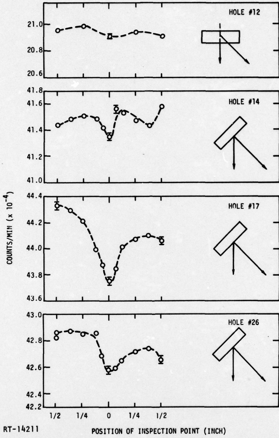
RT-14211 Figure 30. Response of the photon scattering gauge to holes 12, 14, 17, and 21 at one depth each
