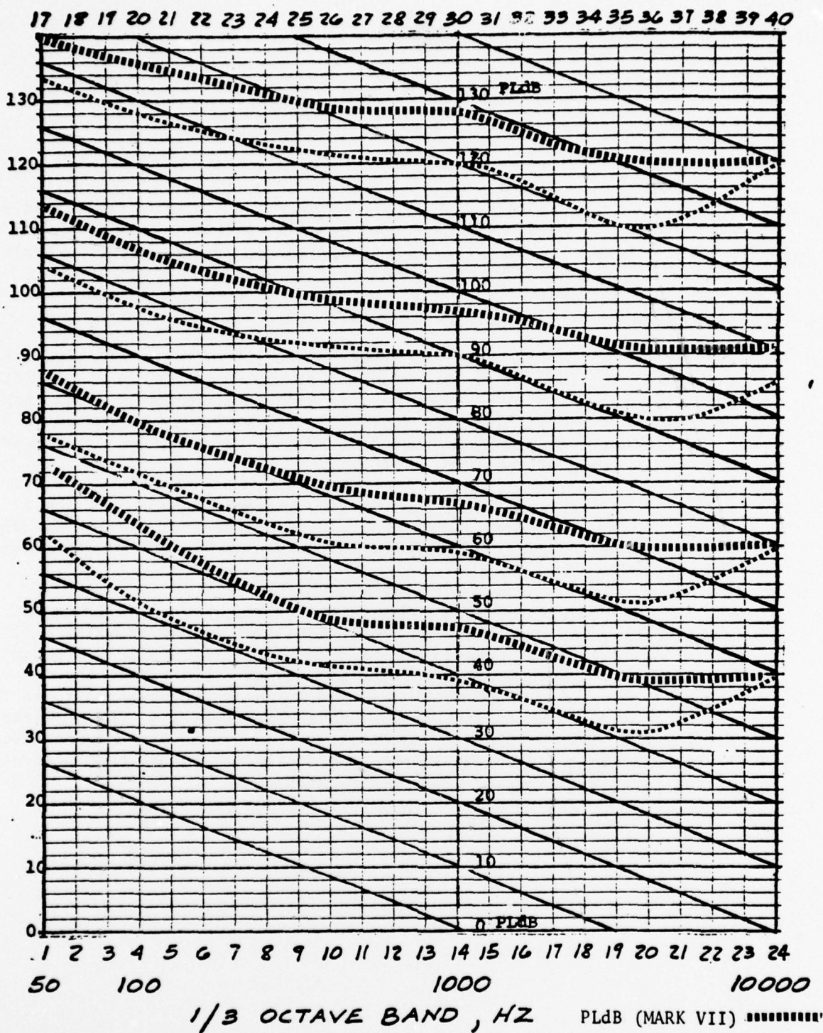
FIGURE 10. COMPARISON OF PNdB, PLdB (MARK VII) AND PLdB (EQUATIONS 11 & 12) PERCEIVED LEVEL CONTOURS
