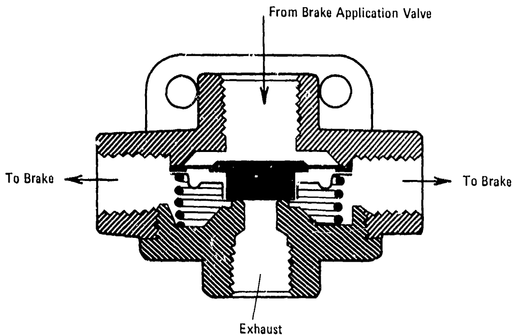
Figure 15-15. Quick-Release Valve
