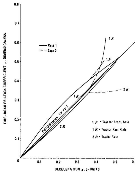
Figure 9-10. Tire-Road Friction Utilization, Cases 1 and 2, W_2 = 43,000 \text{ lb}
