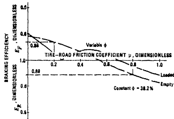
Figure 14-22. Braking Efficiency for Variable Ratio Braking
