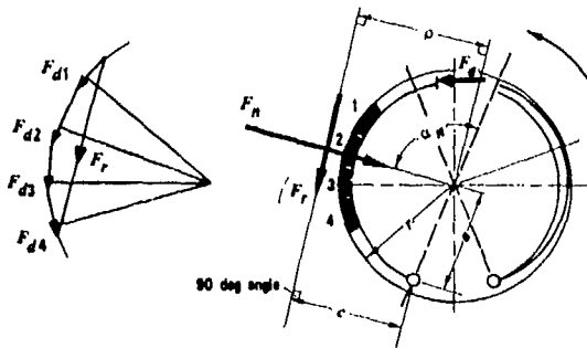
Figure 2-7. Leading Shoe Analysis
