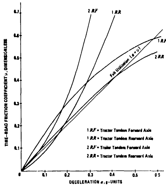
Figure 9-25. Tire-Road Friction Utilization for 3-S2 Tractor-Semitrailer (Empty) With Proportioning (No Front Brakes)
