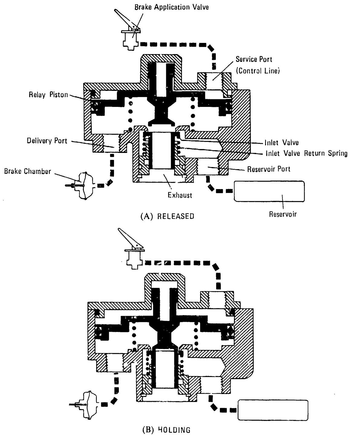
Figure 15-16. Relay Quick-Release Valve
