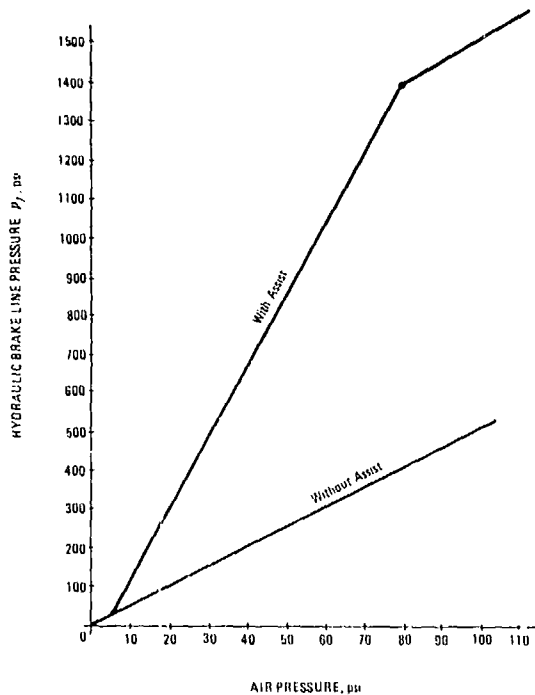
Figure 5-13. Air-Over-Hydraulic Brake Characteristic
