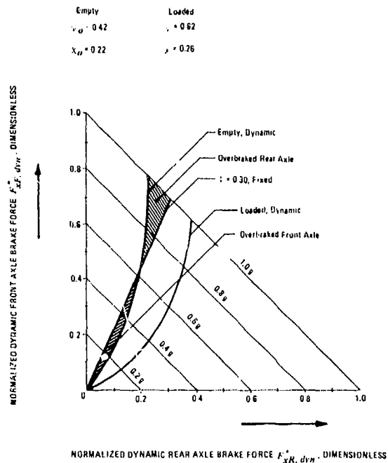
Figure 8-3. Normalized Dynamic Brake Forces
