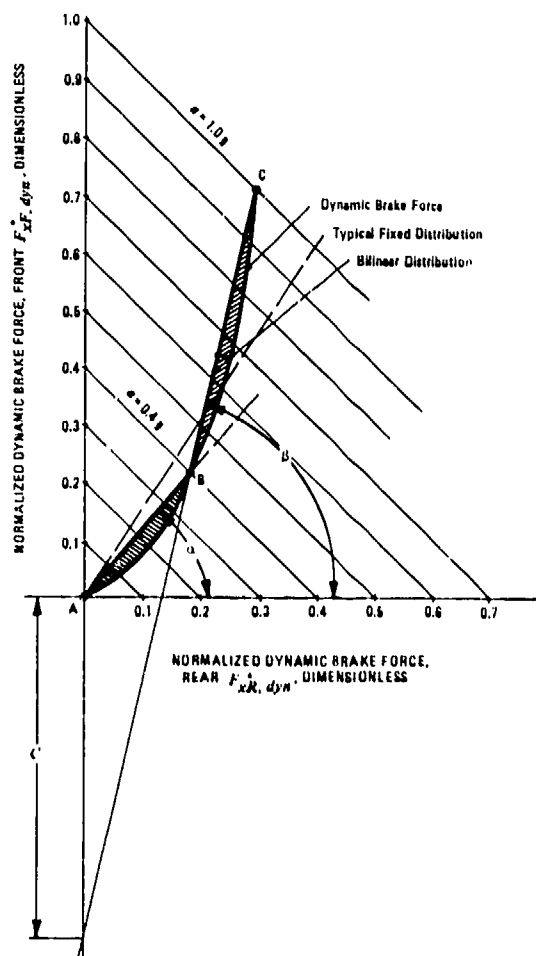
Figure 9-1. Dynamic and Actual Bilinear Brake Forces of Two-Axle Vehicle
