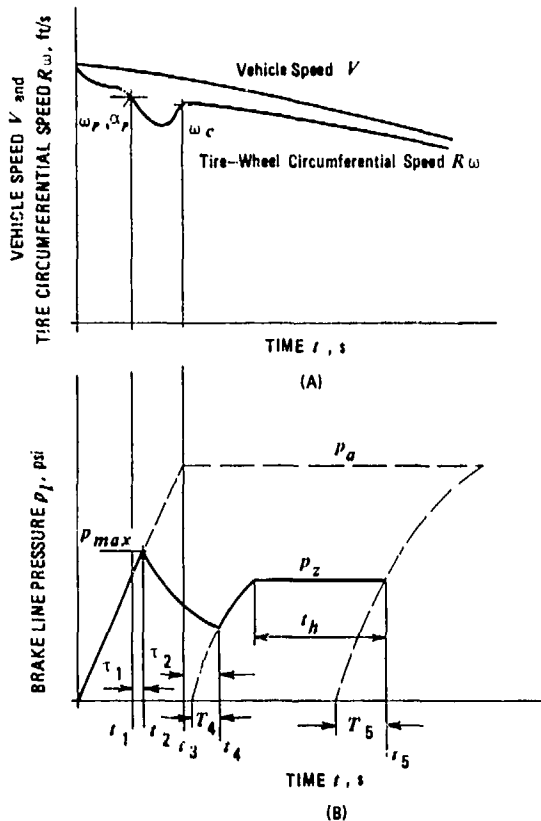
Figure 10-3. Wheel-Antilock Control for an Air Brake System
