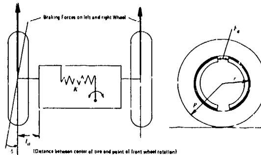
Figure 12-12. Steering Schematic
