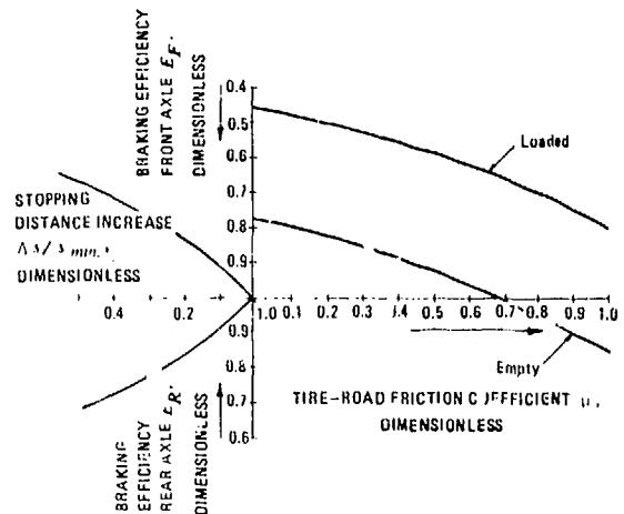
Figure 8-7. Braking Efficiency Diagram
