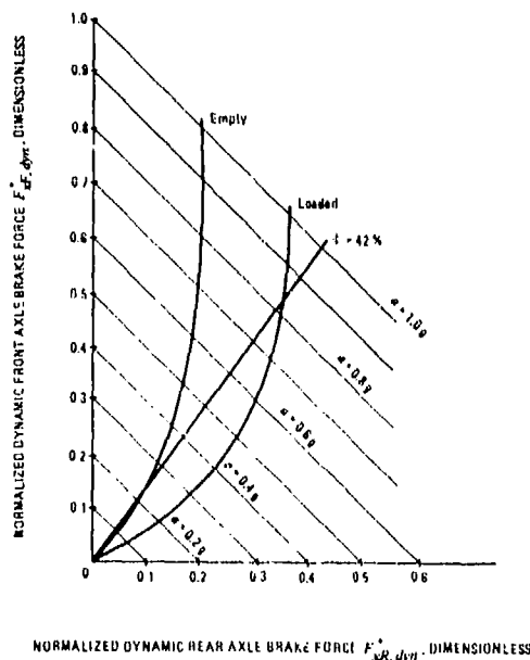
Figure 14-12. Normalized Dynamic and Actual Brake Forces, Vehicle No. 6
