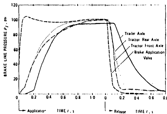
Figure 11-4. Brake Response Times For Tractor-Semitrailer Combination
