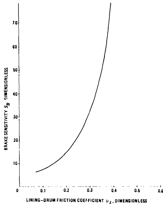
Figure 14-2. Brake Sensitivity
