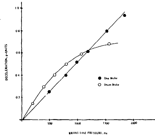
Figure 2-25. Comparison of Measured Braking Performance of Disc and Drum Brakes for a Truck
