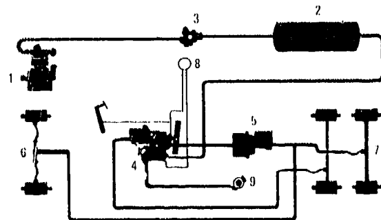
Figure 5-12. Air-Over-Hydraulic Brakes for Tandem Axle Truck
