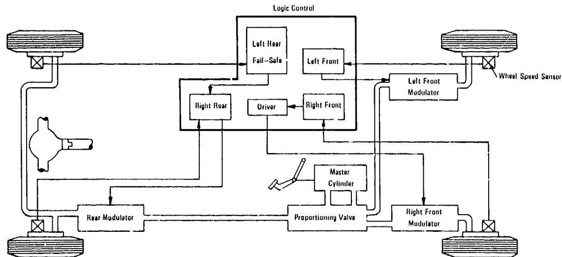
Figure 10-4. Independent Front, Select-Low Rear, Control Method Wheel-Antilock Brake System
