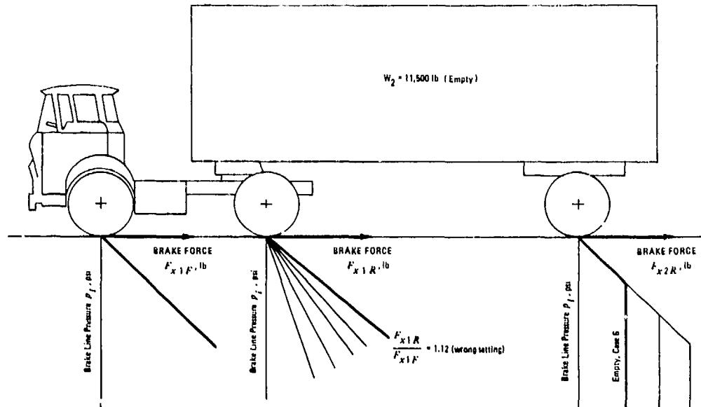
Figure 9-15. Schematic Brake Force Distribution, Case 6
