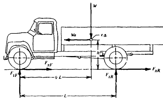
Figure 8-1. Forces Acting on a Decelerating Vehicle
