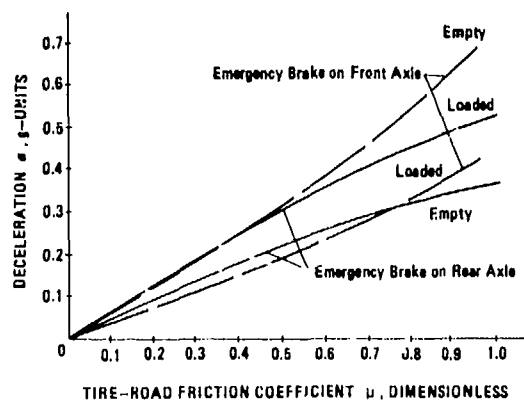
Figure 14-6. Emergency Brake Performance, Vehicle No. 6
