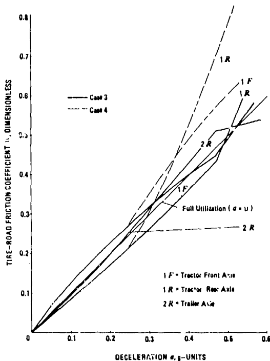
Figure 9-12. Tire-Road Friction Utilization, Cases 3 and 4, W_2 = 27,000 \text{ lb}
