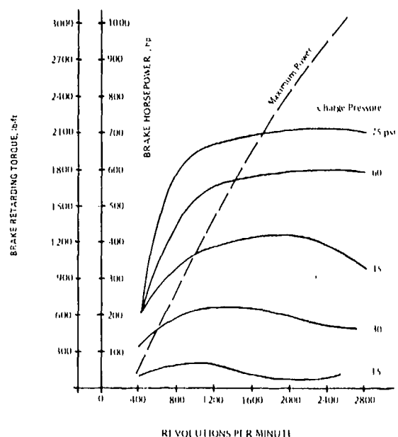
Figure 4-2. Hydrodynamic Retarder Performance Characteristics
