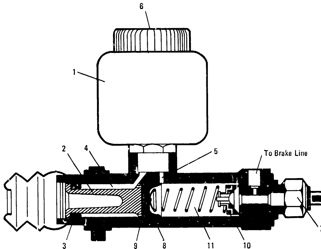
Figure 15-2. Master Cylinder
