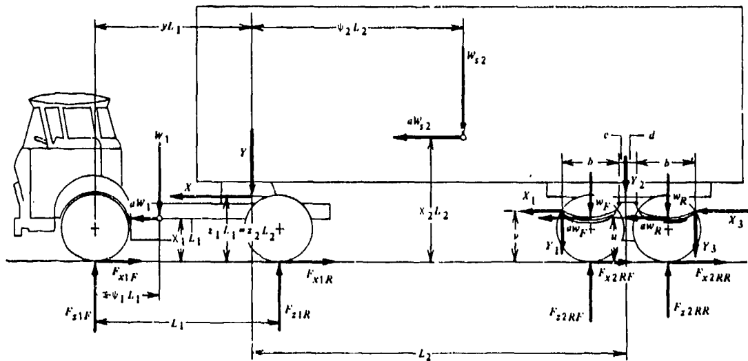
Figure 8-34. Forces Acting on a Tractor-Semitrailer Equipped With Two-Leaf Suspension
