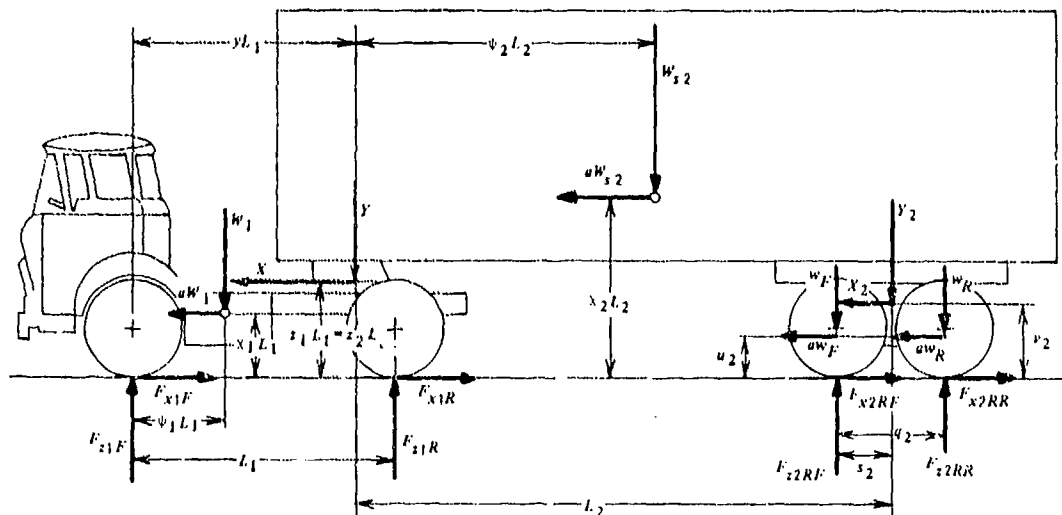
Figure 8-37. Forces Acting on a Tractor-Semitrailer Equipped With Walking Beam Suspension
