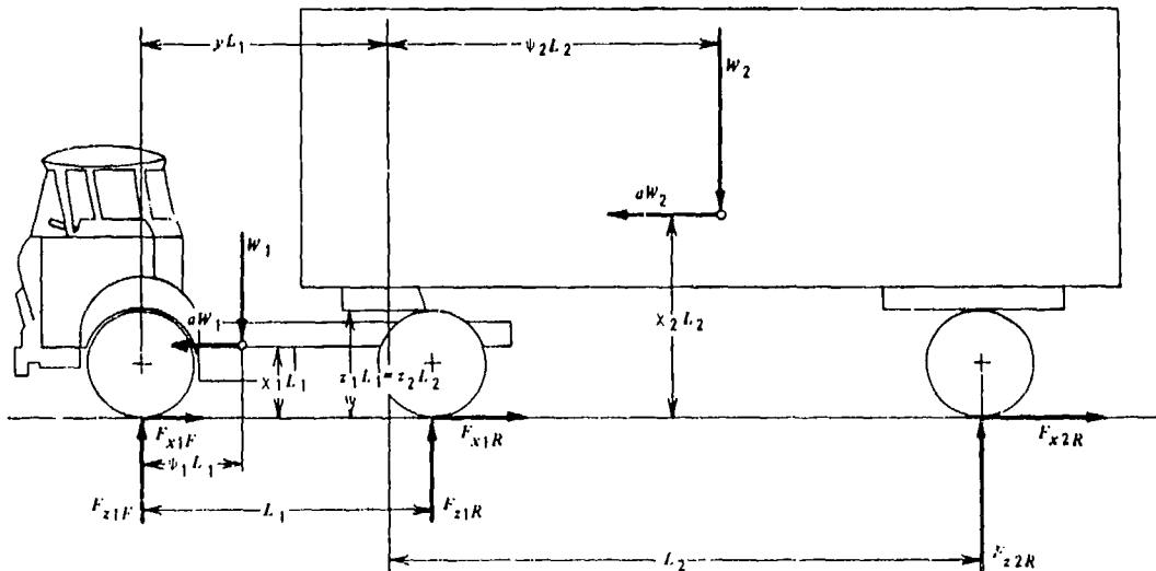
Figure 8-29. Forces Acting on a Decelerating Tractor-Semitrailer
