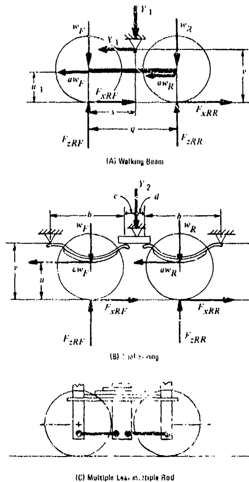
Figure 8-15. Tandem Axle Suspensions
