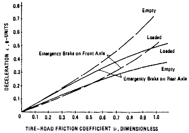
Figure 14-5. Emergency Brake Performance, Vehicle No. 4
