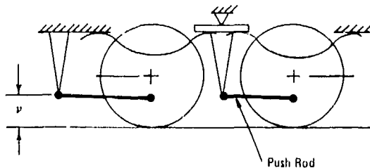
Figure 8-24. Two-Leaf-Two-Rod Suspension
