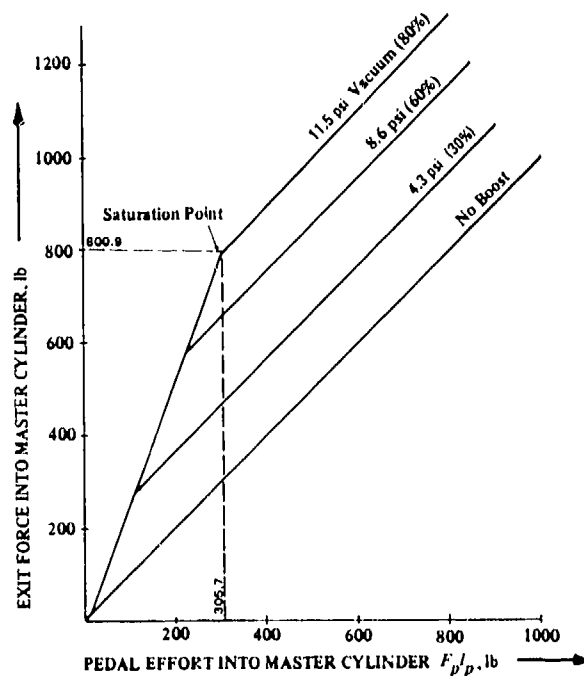
Figure 5-4. Mastervac Characteristics
