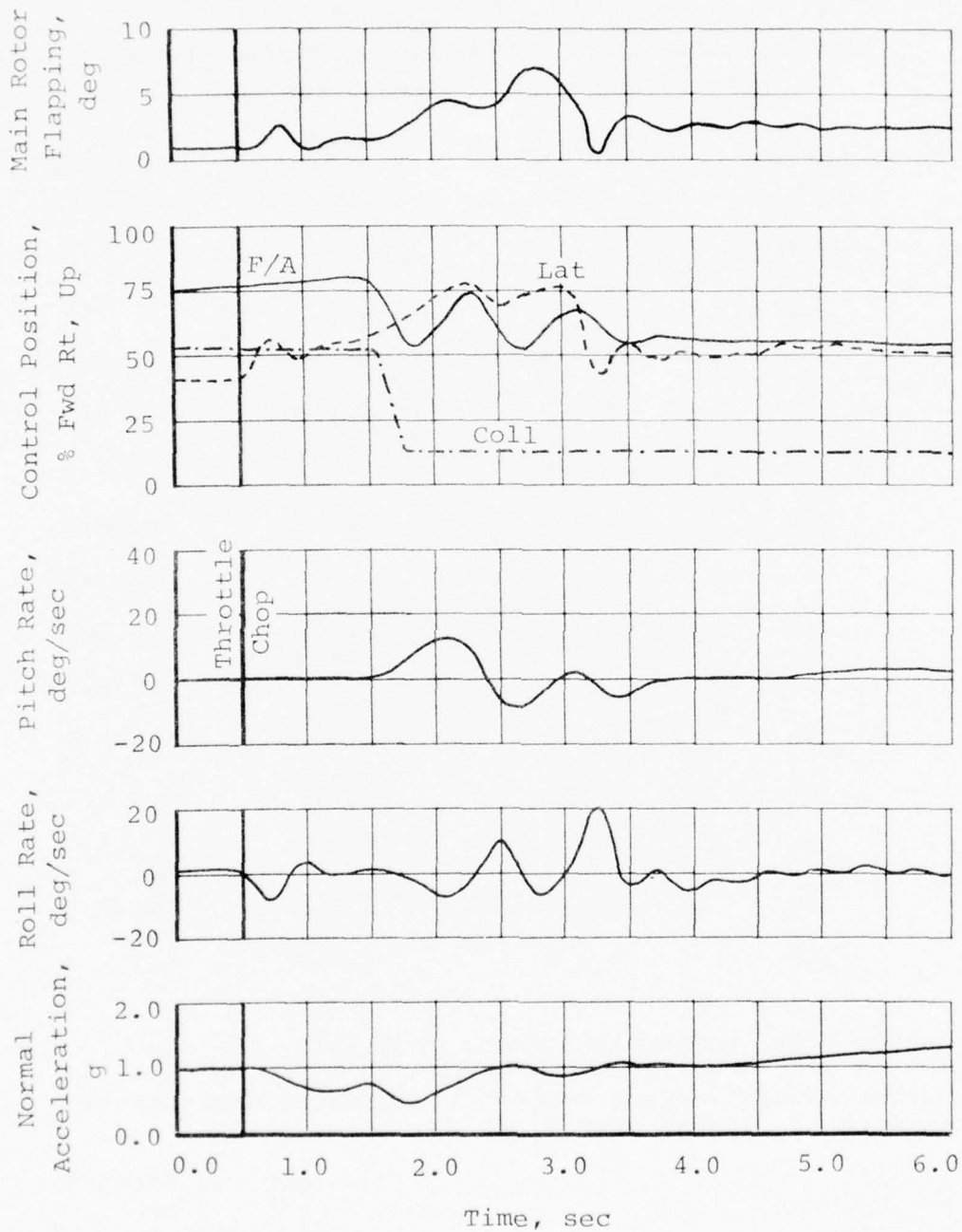
Figure 23. Typical autorotation entry maneuver.
