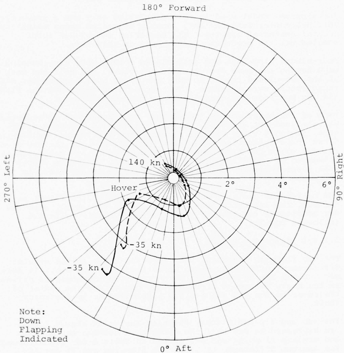
Figure 18. Effect of hub restraint on main rotor flapping in trimmed level flight.
