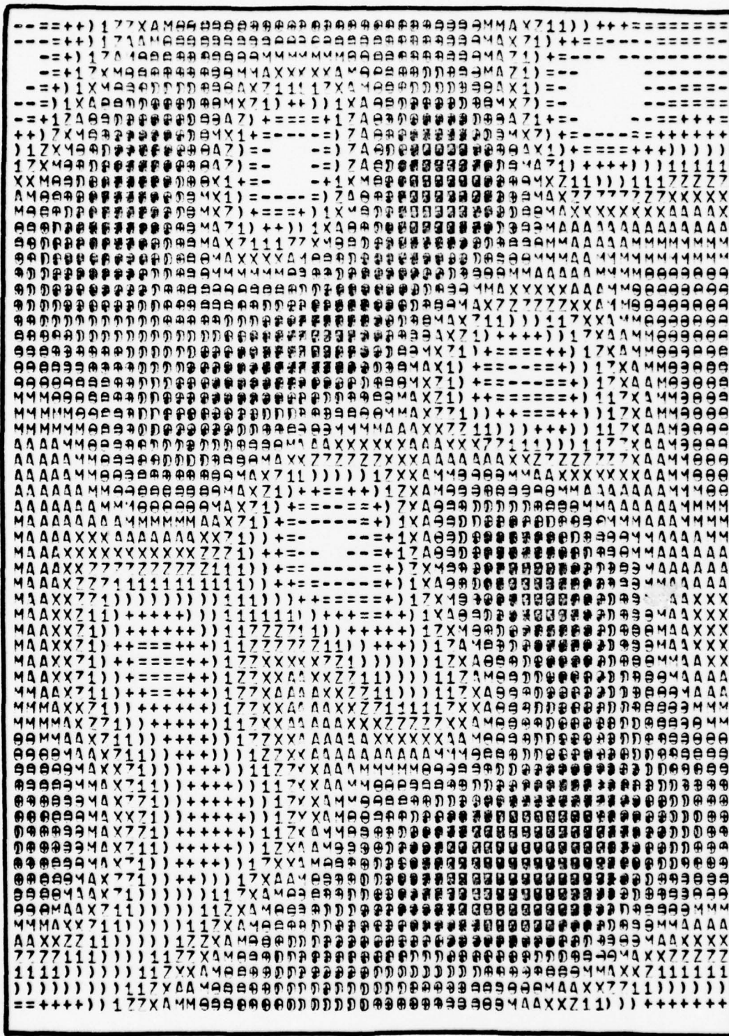
Fig. 9. New Symbol 6 from Gram-Schmidt Orthogonalization.
