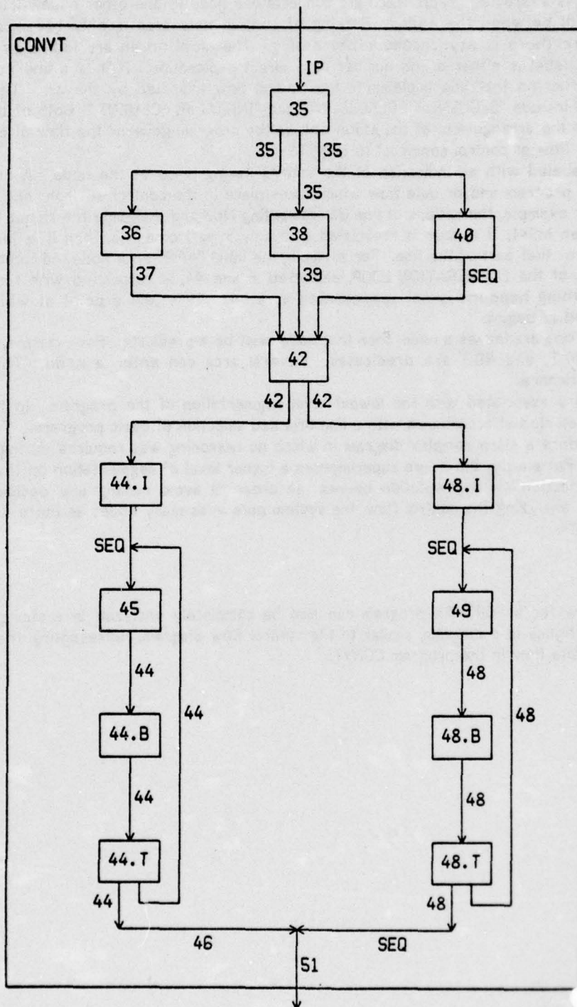
Fig 26: The control flow in the program CONVY. SEQ=SEQUENTIAL PLACEMENT, IP=INITIAL PLACEMENT.
