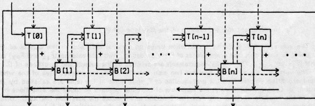
Fig. 18: Schematic for the plan for an unbounded computation achieving the \{G[i]\}
