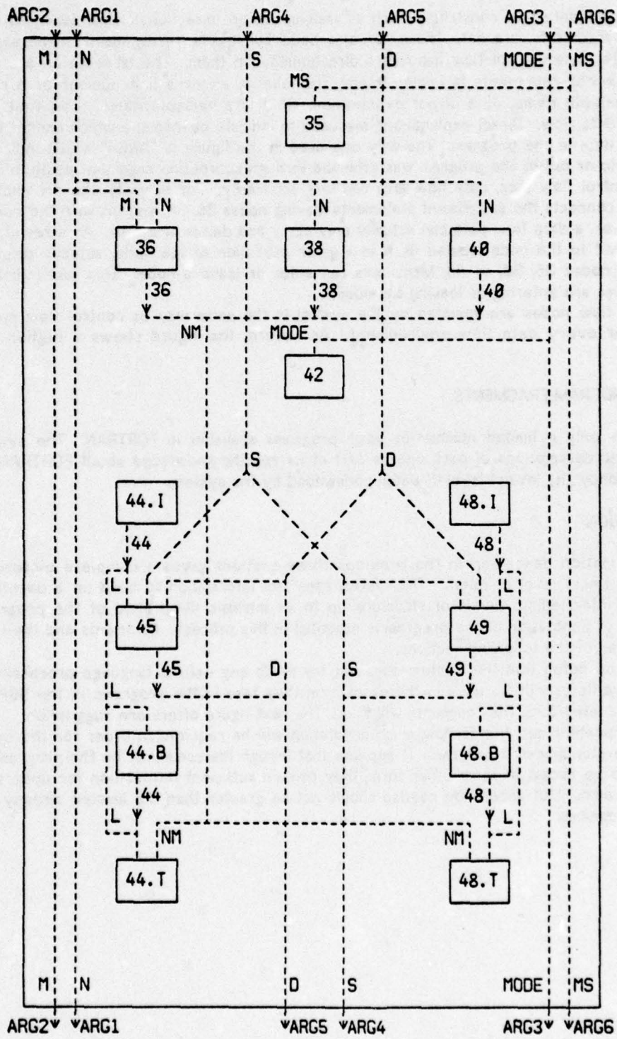
Fig. 27: The data flow in the program CONVNT
