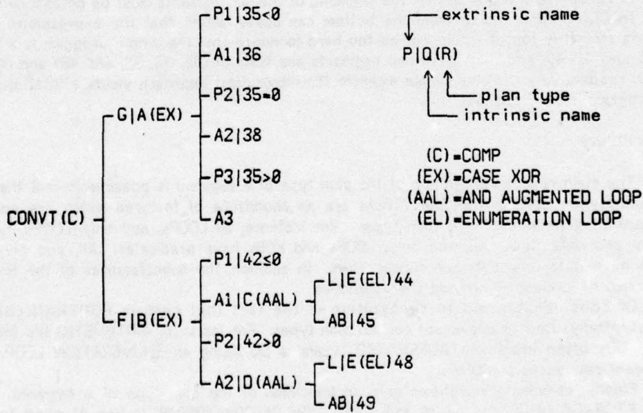
Fig. 29: Schematic of the grand plan for CONV T. This is a shorthand notation for a diagram of the grand plan similar to the diagrams for the plan types in section III.3. This figure shows how the plans are imbedded. The diagrams in section III.3 show what the diagram corresponding to each node of the schematic looks like.
