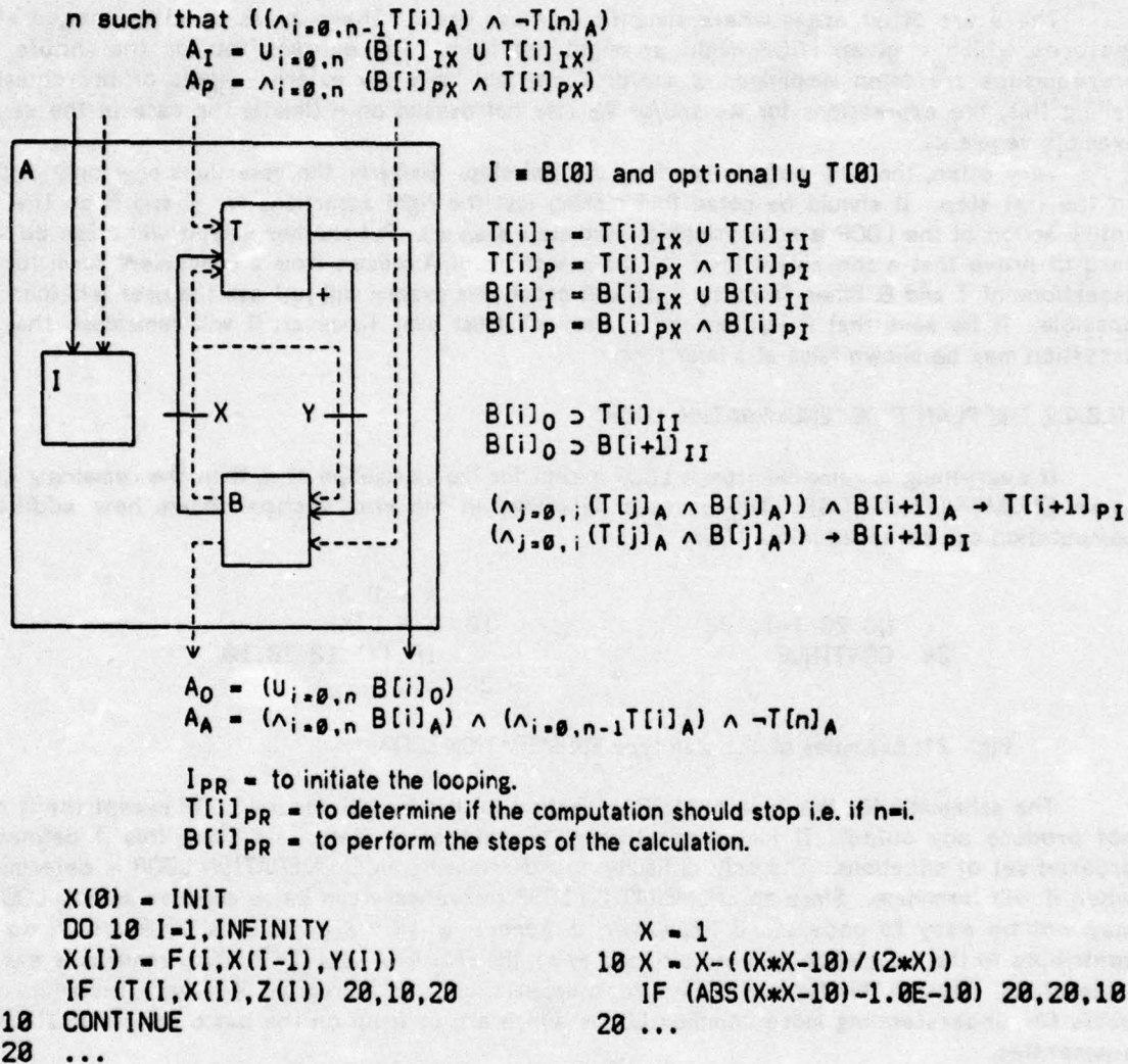
Fig. 20: Schematic for, and examples of, the plan type LOOP
