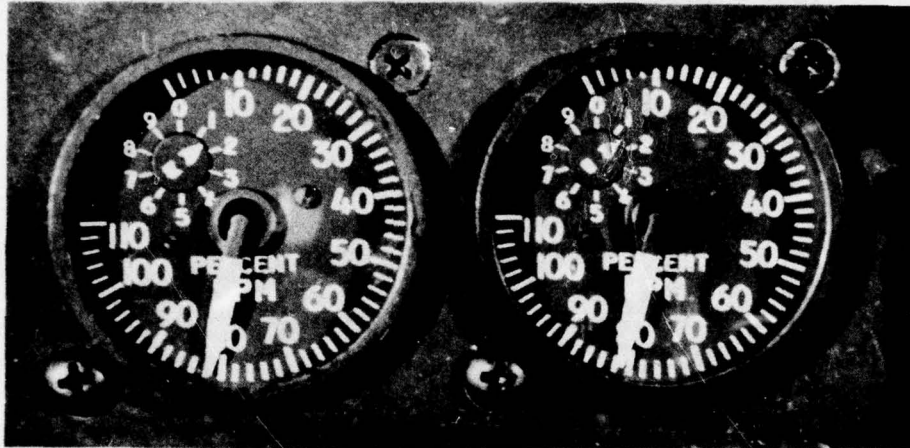
Figure 13. Tachometers
