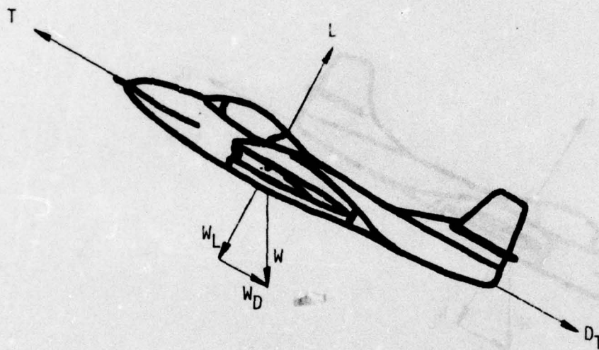
Figure 4. Level Climb
