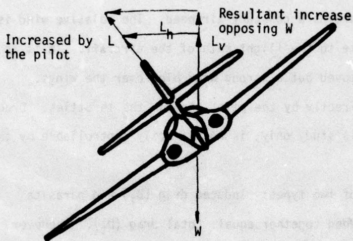
Figure 3. Left Turn (Rear View)
