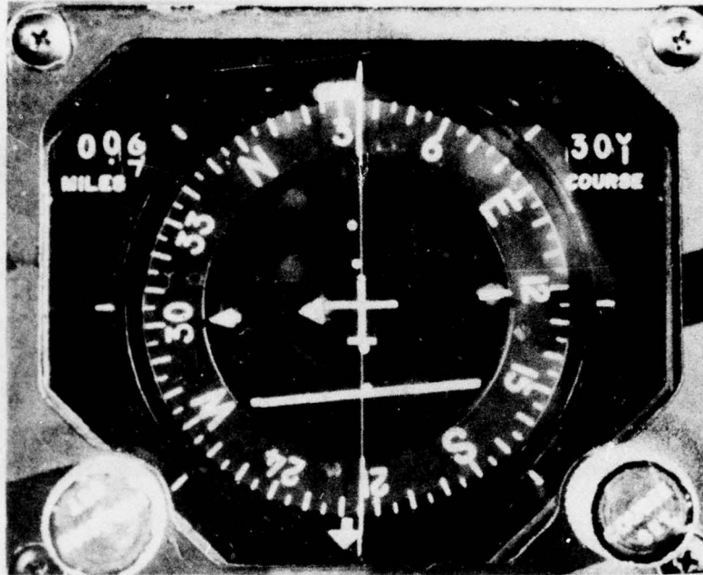
Figure 12. Heading Indicator
