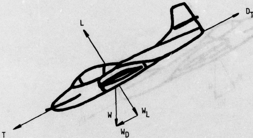
Figure 5. Level Descent
