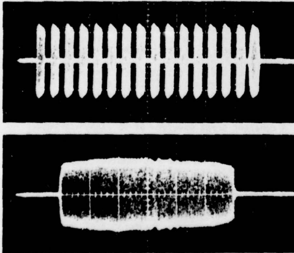
Fig. 7 (a) Burst waveform consisting of 16 linear-FM subpulses. Horizontal scale is 10 \mu s /div. (b) Detailed view of one linear-FM subpulse. Horizontal scale is 0.5 \mu s /div.
