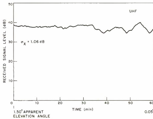
Fig. III-2. Received signal levels at low elevation angles.
