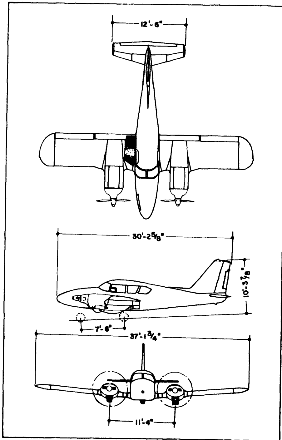
Figure 3. General dimensions of M6del PA23-250C Airplane.
