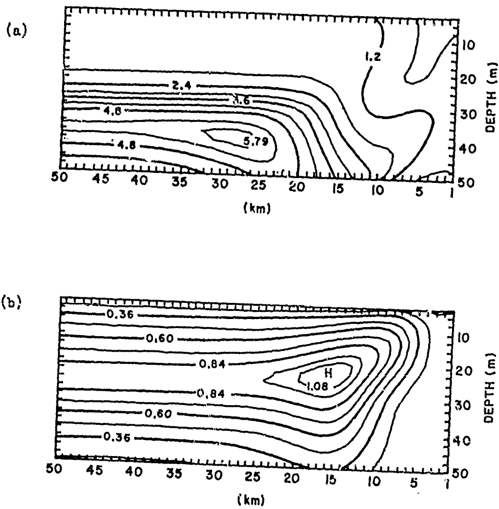
Fig. 22. (a) Ammonia field after 10 days in the strong upwelling case. Contour intervals are 0.6 \mu\text{gat NH}_4 \ell^{-1} . (b) Spatial distribution of detritus after 10 days in the strong upwelling case. Contour intervals are 0.12 \mu\text{gat N } \ell^{-1} .
