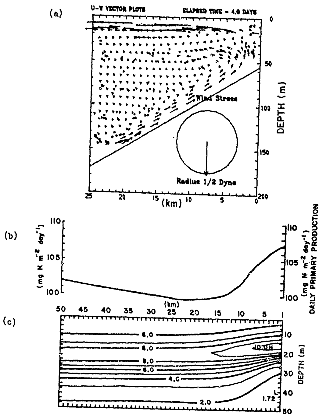
Fig. 18. (a) The upwelling circulation in the transverse plane normal to the coast after 4 days in the strong upwelling case. The bottom topography and the wind stress at day 4 are also shown. The maximum u and w velocities in the field are -2.9 \text{ cm sec}^{-1} and 1.4 \times 10^{-2} \text{ cm sec}^{-1} , respectively. (b) The gross primary productivity of the water column after 4 days in the strong upwelling case. (c) The spatial distribution of phytoplankton after 4 days in the strong upwelling case. Contour intervals are 1 \mu\text{gat N l}^{-1} .
