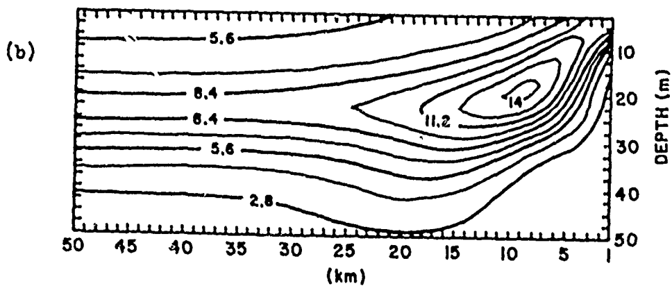
Fig. 30. (a) The spatial distribution of phytoplankton on August 5 in the intermittent upwelling case. Contour intervals are 1.2 \mu\text{gat N l}^{-1} . (b) Same as (a) but on August 15. Contour intervals are 1.4 \mu\text{gat N l}^{-1} .
