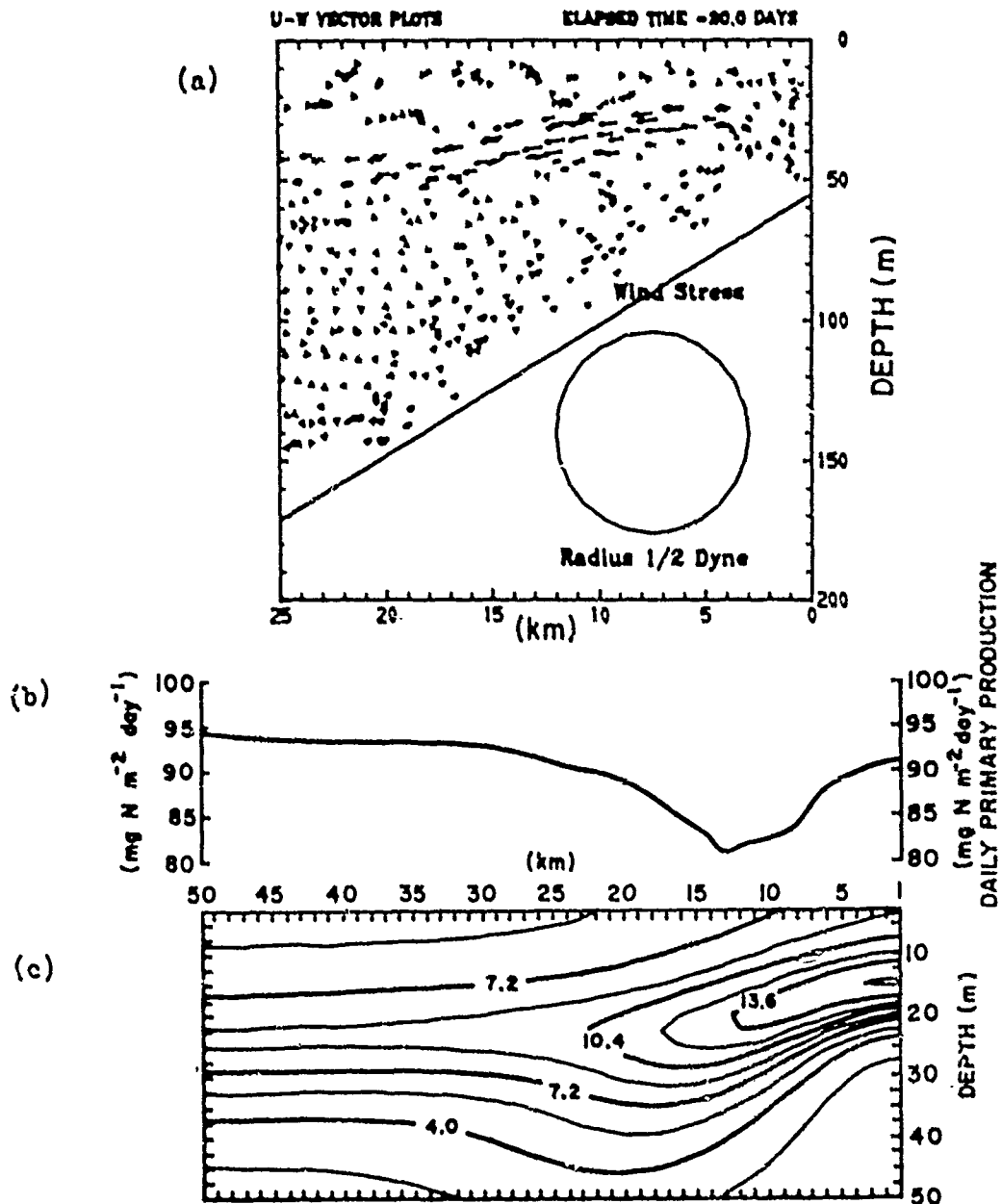
Fig. 24. Same as Fig. 18 but for day 20. The maximum u and w velocities in (a) are \approx 2.8 \text{ cm sec}^{-1} and 7.9 \times 10^{-3} \text{ cm sec}^{-1} , respectively. Contour intervals in (c) are 1.6 \mu\text{gat N l}^{-1} .
