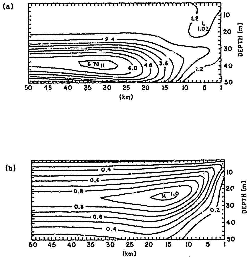
Fig. 34. The ammonia field on August 15 in the intermittent upwelling case. Contour intervals are 0.6 \mu\text{gat NH}_4 \text{ l}^{-1} . (b) The spatial distribution of detritus on August 15 in the intermittent upwelling case. Contour intervals are 0.1 \mu\text{gat N l}^{-1} .
